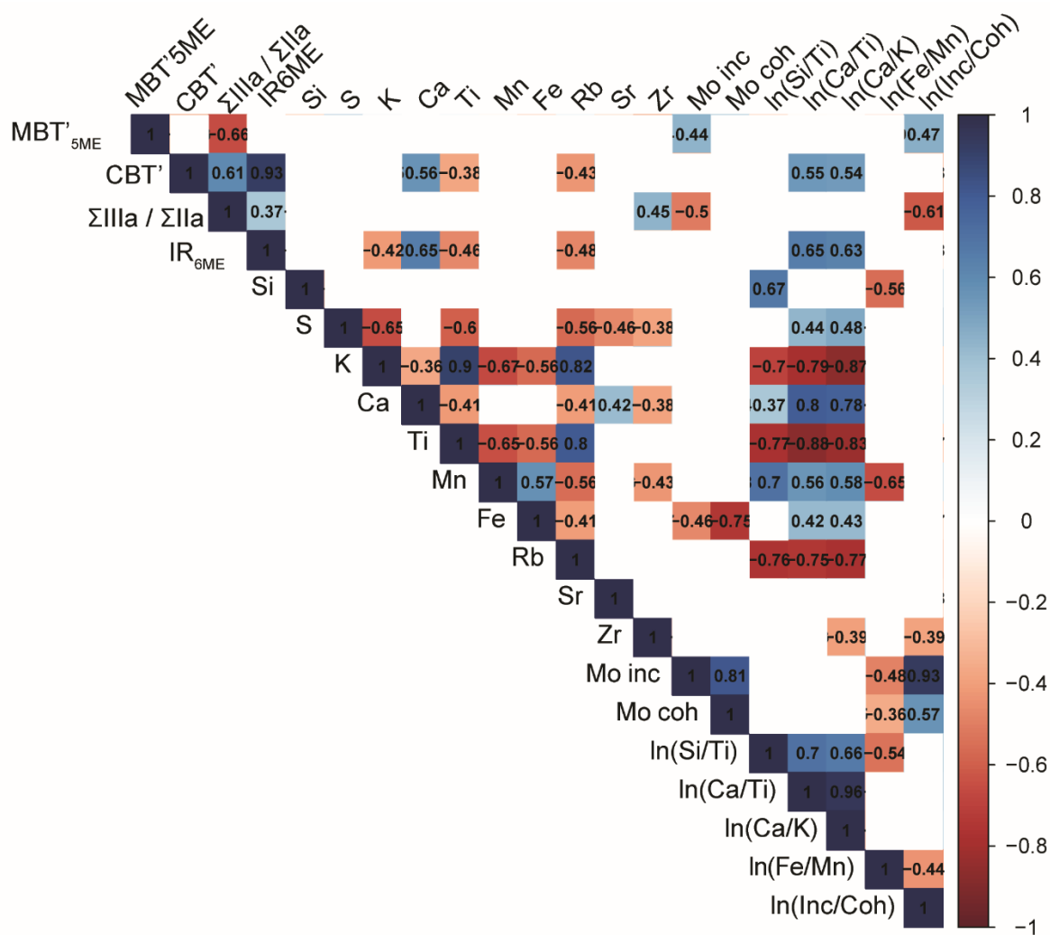
Figure S8. Pearson's correlation coefficients between the main GDGT metrics and \mu -XRF data from Meerfelder Maar. Shown are significant correlations only.
