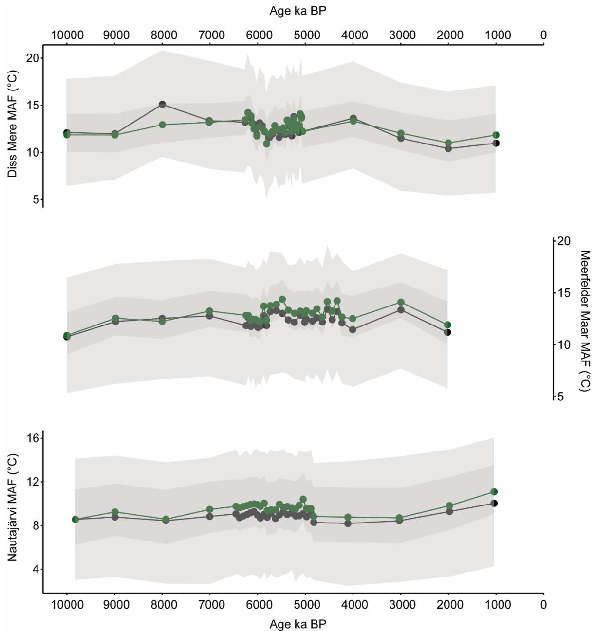
Figure S2. Mean Temperature of Months Above Freezing (MAF) reconstructions from each of the lake sites in this study. The two different reconstructions are black) Bayesian-based MAF reconstructions (Martinez-Sosa et al., 2021); and green) multivariate methylation set MAF reconstructions (Raberg et al., 2021). The dark grey error bars are the calibration uncertainty associated with Raberg et al. (2021). The light grey error bars represent the 95% confidence interval associated Martinez-Sosa et al. (2021).
