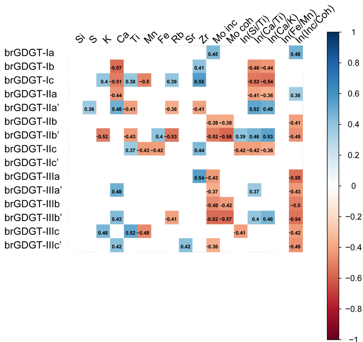
Figure S7. Pearson's correlation coefficients between identified GDGT compounds and \mu -XRF data from Meerfelder Maar. Shown are significant correlations only.
