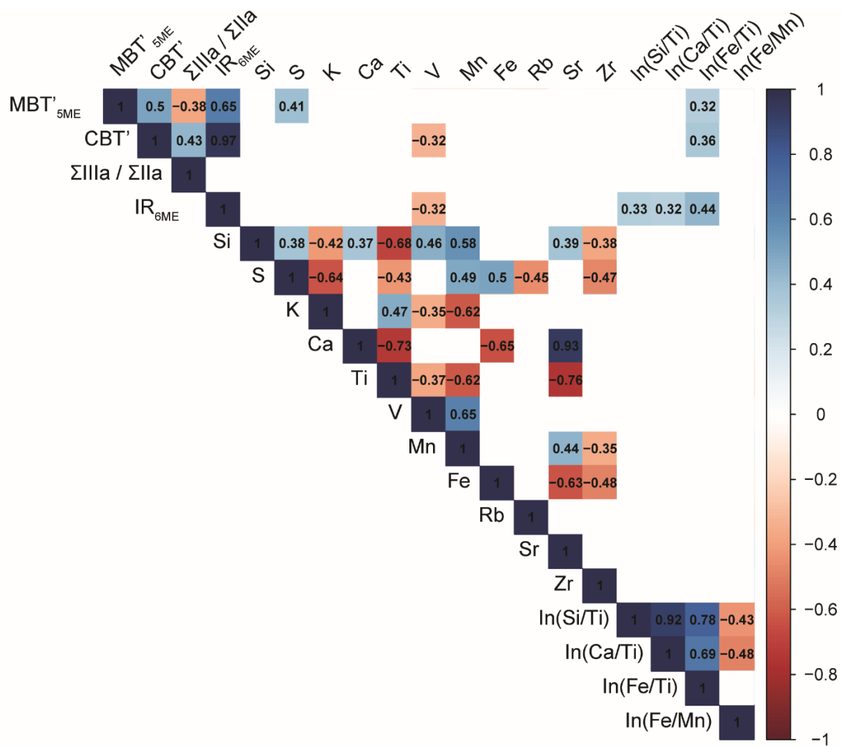
Figure S4. Pearson's correlation coefficients between the main GDGT metrics and \mu -XRF data from Diss Mere. Shown are significant correlations only.
