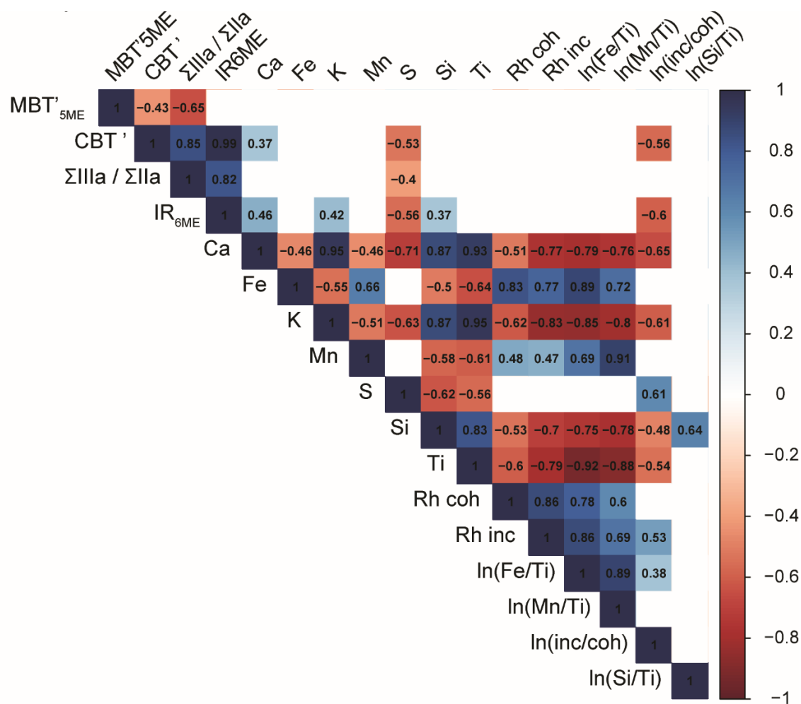
Figure S6. Pearson's correlation coefficients between the main GDGT metrics and \mu -XRF data from Nautajärvi. Shown are significant correlations only.
