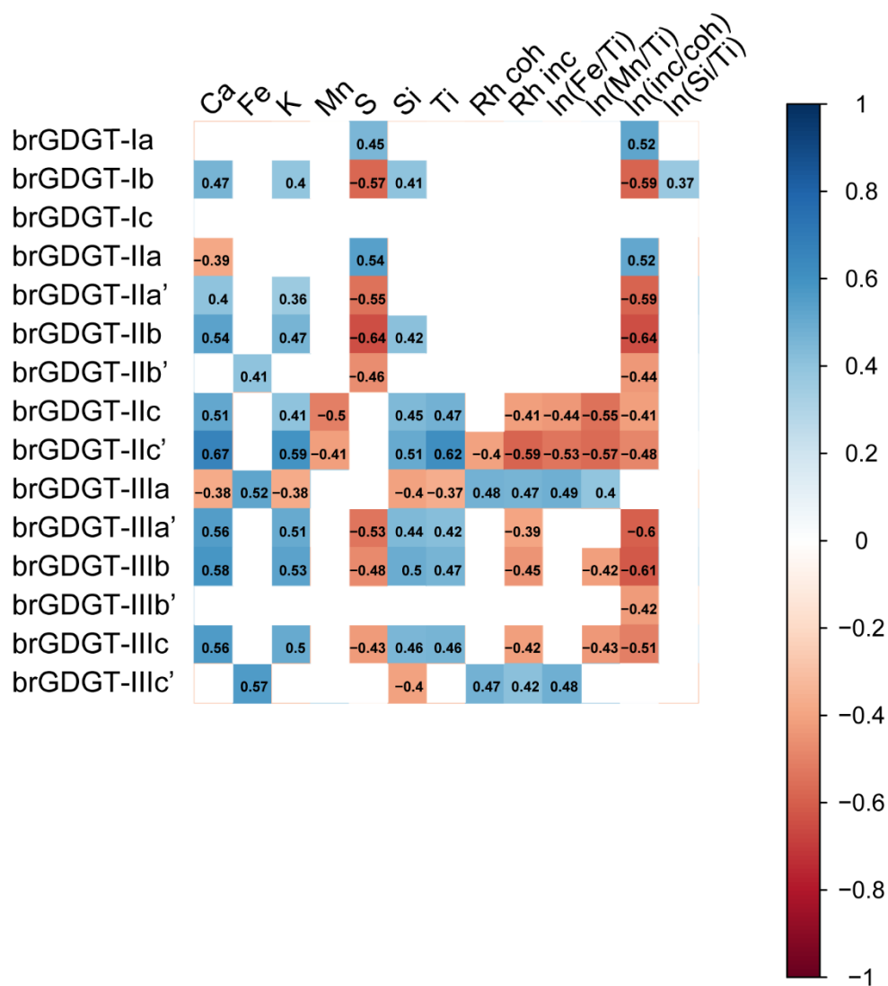
Figure S5. Pearson's correlation coefficients between identified GDGT compounds and \mu -XRF data from Nautajärvi. Shown are significant correlations only.
