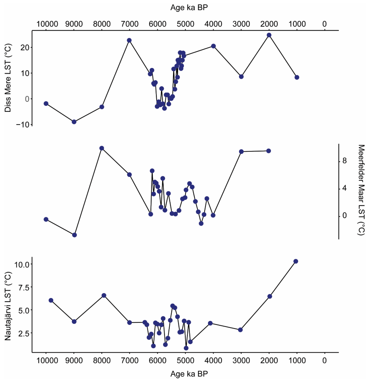
Figure S1. Lake Surface Temperature (LST) reconstructions from the three sites in this study.
