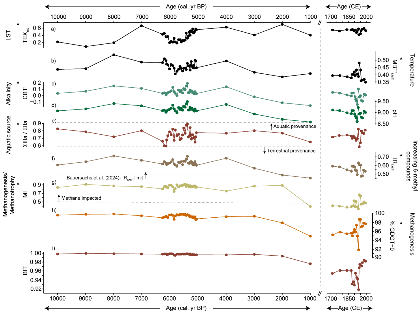
Figure 5: Main GDGT reconstructions from Diss Mere. Shown are a) TEX 86 ; b) MBT' 5ME (De Jonge et al., 2014); c) CBT' (De Jonge et al., 2014); d) reconstructed pH (Russell et al., 2018); e) \Sigma IIIa / \Sigma IIa ratios with cut offs from Xiao et al. (2016); f) IR 6ME (De Jonge et al., 2014; Bauersachs et al., 2024); g) the methane index (Zhang et al., 2011); h) % GDGT-0 and i) the branched vs isoprenoid tetraether index (BIT).
