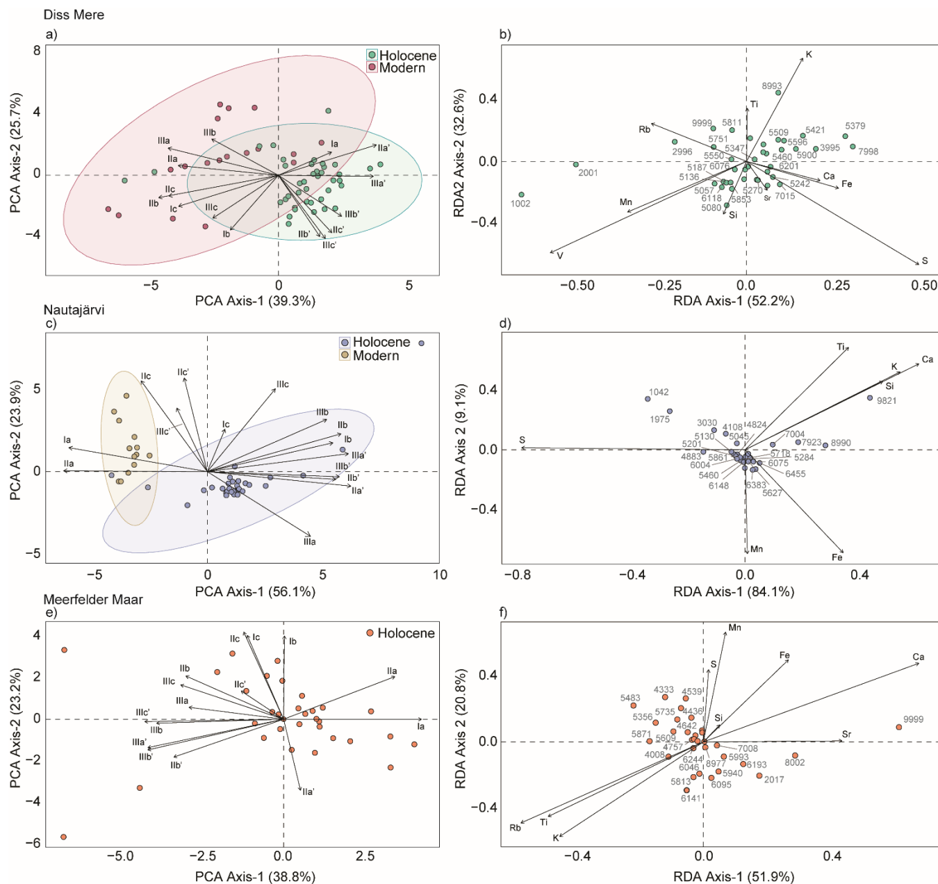
Figure 4: Principal components analysis (PCA) left, and redundancy analysis (RDA) right. a) and b) detail the plots from Diss Mere; c) and d) from Nautajärvi; and e) and f) from Meerfelder Maar. a) and c) show modern (last 300-years) and Holocene sample distributions within the PCA plots. Explanatory variables in the RDA plots are major elements from \mu -XRF data (from Martin-Puertas et al. (2012); Boyal et al. (2024); Lincoln et al. (2025)) with numerical points showing the median age of samples.
