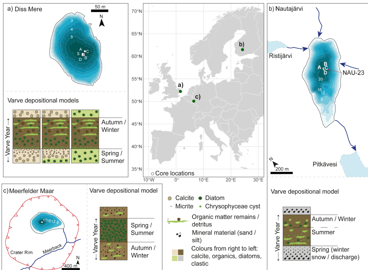
Figure 1: Location of each of the sites in Europe: a) Diss Mere, UK; b) Nautajärvi, Finland; c) Meerfelder Maar, Germany. Site boxes reveal lake bathymetry with depths and inflows/outflows. Varve depositional models are added to each box which demonstrate the main varve facies from each location, with three varve microfacies at Diss Mere and one each at Nautajärvi and Meerfelder Maar. Letters denote different cores from a) and b). Diss Mere adapted from Boyall et al. (2023); Nautajärvi adapted from Lincoln et al. (2025).
