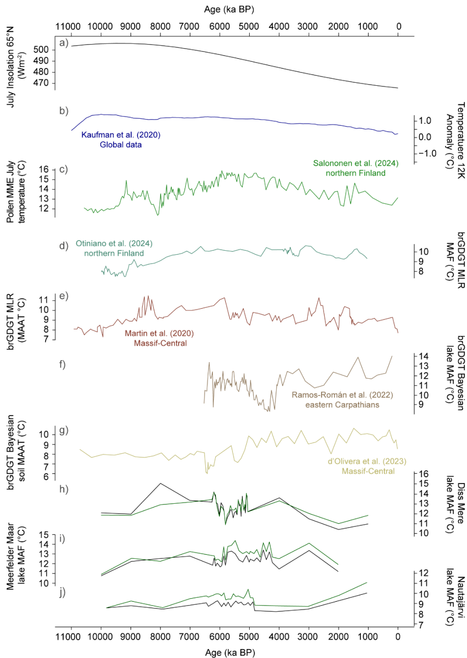
595 Figure 9: Comparative Holocene climate records. a) summer insolation at 65°N; b) Holocene global surface temperature anomalies (Kaufman et al., 2020); c) a pollen-based multi-method ensemble of Holocene July temperatures (Salonen et al., 2024); d) brGDGT 600 multiple linear regression MAF temperatures, northern Finland (Otiniano et al., 2024); e) brGDGT multiple linear regression MAAT temperatures, Massif-Central, France (Martin et al., 2020); f) brGDGT Bayesian MAF temperatures, eastern Carpathians, Romania (Ramos-Román et al., 2022); g) brGDGT Bayesian MAAT temperatures, Massif-Central, France (d'Olivera et al., 2023); and h, i, j) the Bayesian lake MAF (black; Martinez-Sosa et al., 2021) and methylation set multivariate regression MAF reconstructions (green; Raberg et al., 2021) from sites in this study.
