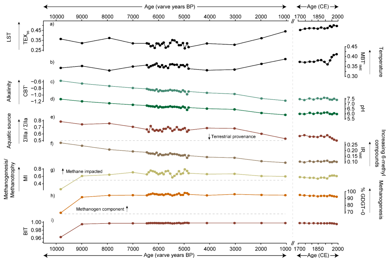
Figure 6: Main GDGT reconstructions from Nautajärvi. Shown are a) \text{TEX}_{86} ; b) \text{MBT}'_{5\text{ME}} (De Jonge et al., 2014); c) \text{CBT}' (De Jonge et al., 2014); d) reconstructed pH (Russell et al., 2018); e) \Sigma\text{IIIa} / \Sigma\text{IIa} ratios with a cut off from Xiao et al. (2016); f) \text{IR}_{6\text{ME}} (De Jonge et al., 2014); g) the methane index (Zhang et al., 2011); h) % GDGT-0 and i) the branched vs isoprenoid tetraether index (BIT).
