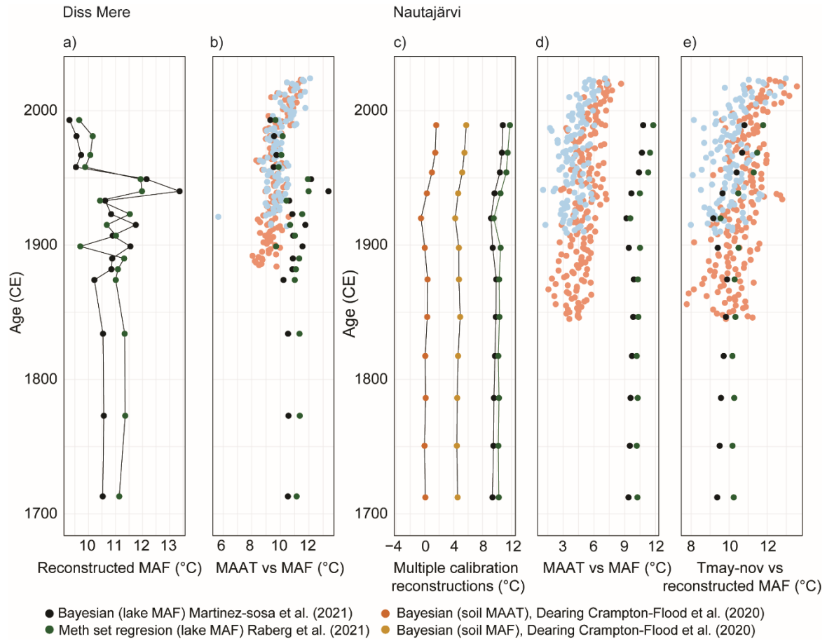
Figure 8: Modern (< 300-year) temperature reconstructions from Diss Mere and Nautajärvi. Shown are a) GDGT-based MAF reconstructions at Diss Mere; b) this data alongside modern MAAT instrumental data from both the Lowestoft meteorological station (light blue) and from 5 km gridded temperatures using the HadUK dataset (light orange; Hollis et al., 2019); c) GDGT-based MAAT and MAF reconstructions at Nautajärvi; d) these GDGT-based MAF reconstructions alongside modern MAAT instrumental data from the Heinola Asemantaus (light blue) and Helsinki Kaisaniemi (light orange) meteorological stations; and e) Nautajärvi GDGT reconstructions against re-sampled May–November meteorological station air temperature data.
