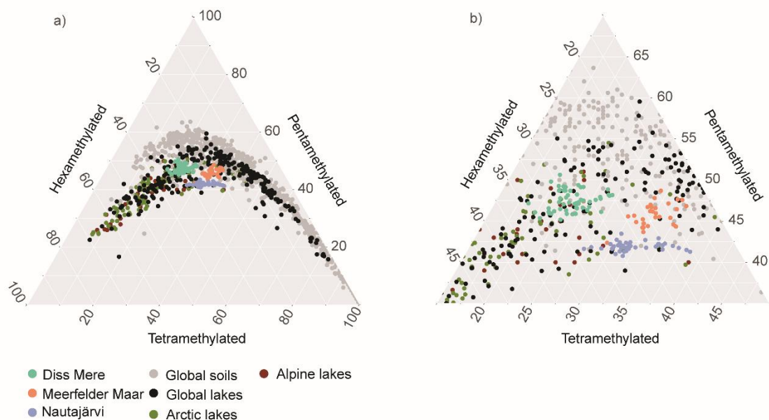
Figure 3: Ternary plots showing a) the relative proportions of tetramethylated, pentamethylated and hexamethylated compounds from Diss Mere, Meerfelder Maar and Nautajärvi, respectively against the same data from a global brGDGT peat and soil dataset (grey; Dearing Crampton-Flood et al., 2020); a global lake dataset (black; Martinez-Sosa et al., 2021); Arctic lakes (green; Raberg et al., 2021) and Alpine lakes (red; Bauersachs et al., 2024); and b) an inset figure of a).
