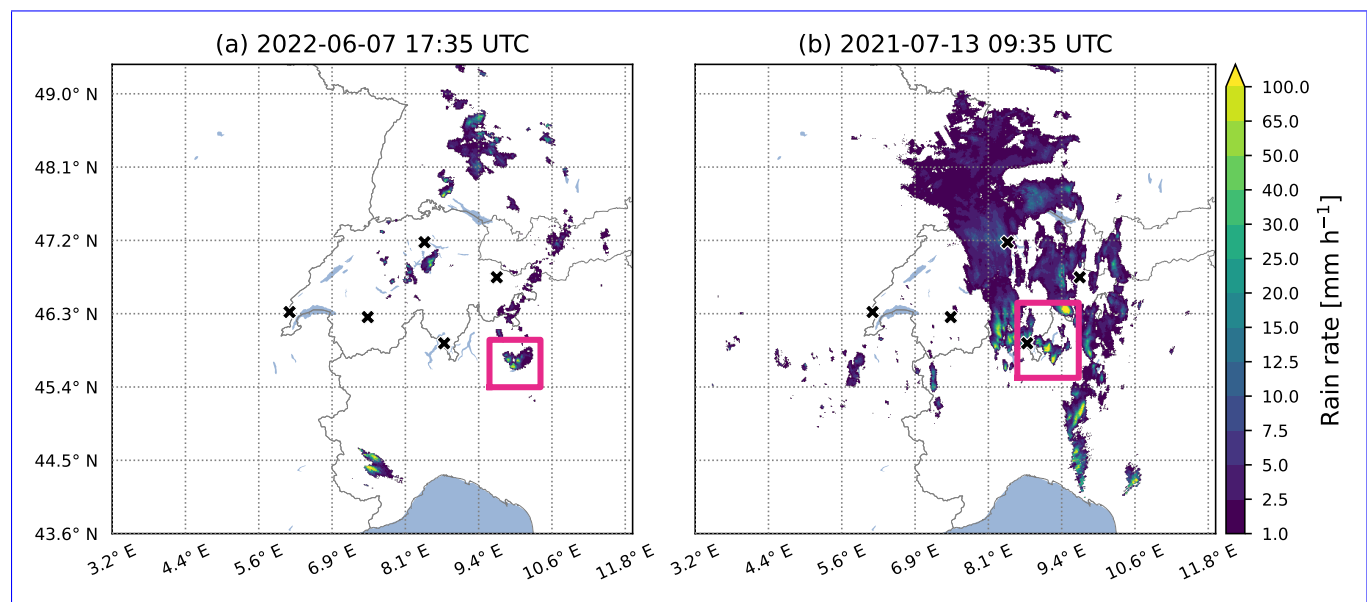
Figure 3. Overview of the rainfall field for the case studies at (a) June 7th 2022 17:35 UTC and (b) July 13th 2021 09:35 UTC. The magenta boxes indicate the area shown in (a) Fig. 4 and (b) Fig. 5. The crosses indicate radar locations, and the distance between the grid lines is 100 km.
