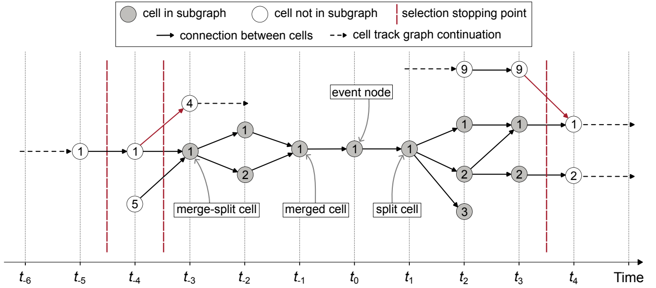
Figure 2. Example of cell subgraph selection from the cell track graph. For the event node (t_0, 1) labelled 1 at time t_0 the subgraph selection stopping points are presented with dashed vertical lines and cells accepted into the subgraph are coloured as grey. The arrows in the graph represent the temporal connections between the cells.
