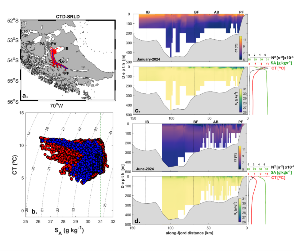
Figure 5. a) Locations of the hydrographic profiles of Absolute Salinity ( S_A ) and Conservative Temperature (CT) acquired via CTD-SRLD (Southern elephant seals) and CTD-AML. CTD-SRLD data points within Bahia Inutil, Whiteside Channel, and Almirantazgo Fjord are marked in red. b) CT/SA diagram the complete dataset (red dots) whereas in blue dots are the January and June elephants seals data showed in c) and d). Segmented black lines are isopycnals of conservative density anomaly ( \sigma_{CT} )
