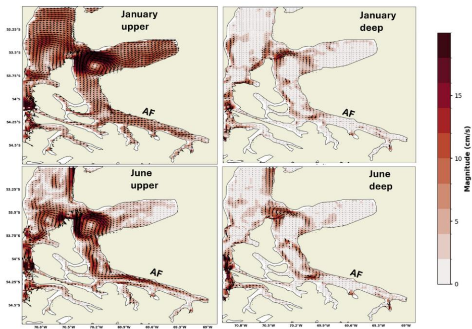
A3. MIKE 3D output model of IFOP – CHONOS. Upper and deeper circulation in the study region to determine the exchange fluxes in the Almirantazgo fjord (AF).
