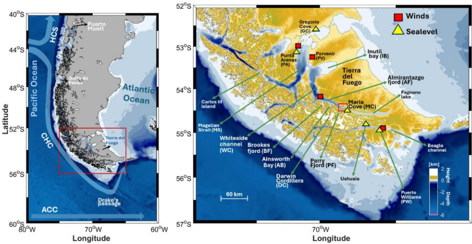
195 Figure 1: Study region. At the left side, a regional map of the interest region shows the main currents systems: the Humboldt Current System (HCS), the Cape Horn Current (CHC) and the Antarctic Circumpolar Current (ACC). At the right, the complexity of the Southern Patagonia it is shown, here bathymetry and topography are showed in colorscale. Geographic features referenced in the text are identified, including Magellan Strait (MS), Inutil Bay (IB), Whiteside Channel (WC), Almirantazgo Fjord (AF), Brookes Fjord (BF), Ainsworth Bay (AB), Parry Fjord (PF), and Maria Cove (MC). The Darwin Cordillera is denoted by white-shaded high-altitude areas on the island of Tierra del Fuego. Depths and highs data were downloaded from https://www.gebco.net/data-products/gridded-bathymetry-data .
