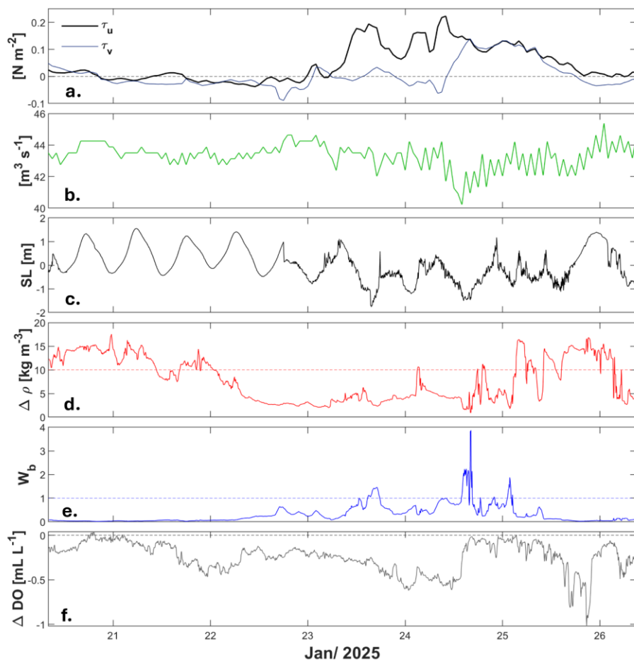
Figure 9. Short time-series acquired at mooring site A2 in Maria Cove (January 20–26, 2025). Panels display, a ) along-fjord ( \tau_u ) and cross-fjord ( \tau_v ) wind-stress components, b ) Azopardo discharge, c ) demeaned sealevel, d ) density gradient ( \Delta\rho ), e ) Wedderburn number ( W_b ) and f ) Dissolved Oxygen gradient ( \Delta DO ).
