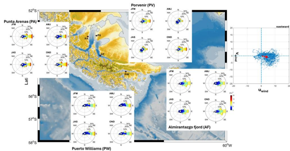
A1. Regional wind climatology for the 1970-2024 period. Wind direction follows the oceanographic convention (indicating the direction towards which the wind blows).
