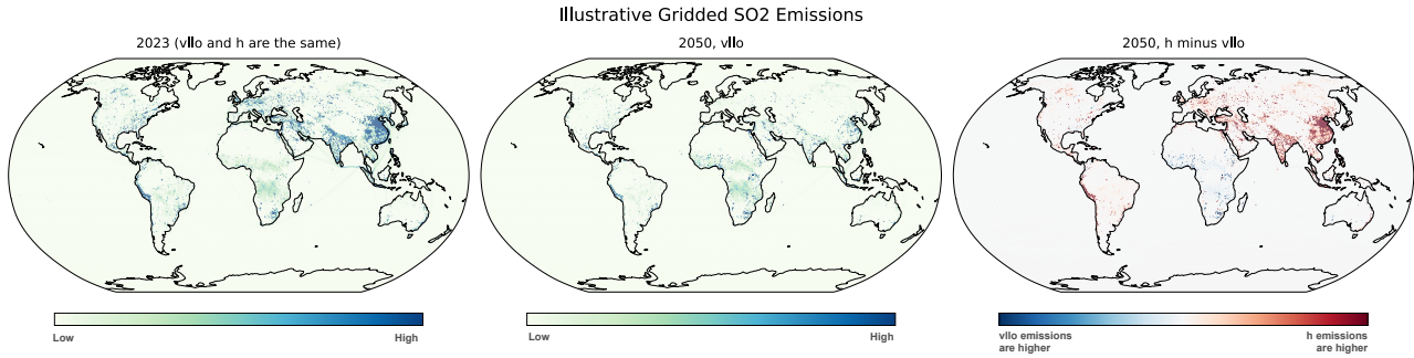
Figure 8. An indicative illustration of possible gridded SO 2 emissions for esm-scen7-vl (VL) and esm-scen7-h (H) marker pathways. Shown are the total emissions for (left to right) the harmonization year 2023 (end of historical data and start of scenarios), esm-scen7-vl in 2050, and their difference between esm-scen7-vl and esm-scen7-h for 2050. The emission totals include anthropogenic emissions at the surface, vertically integrated aircraft emissions, and open burning emissions.
