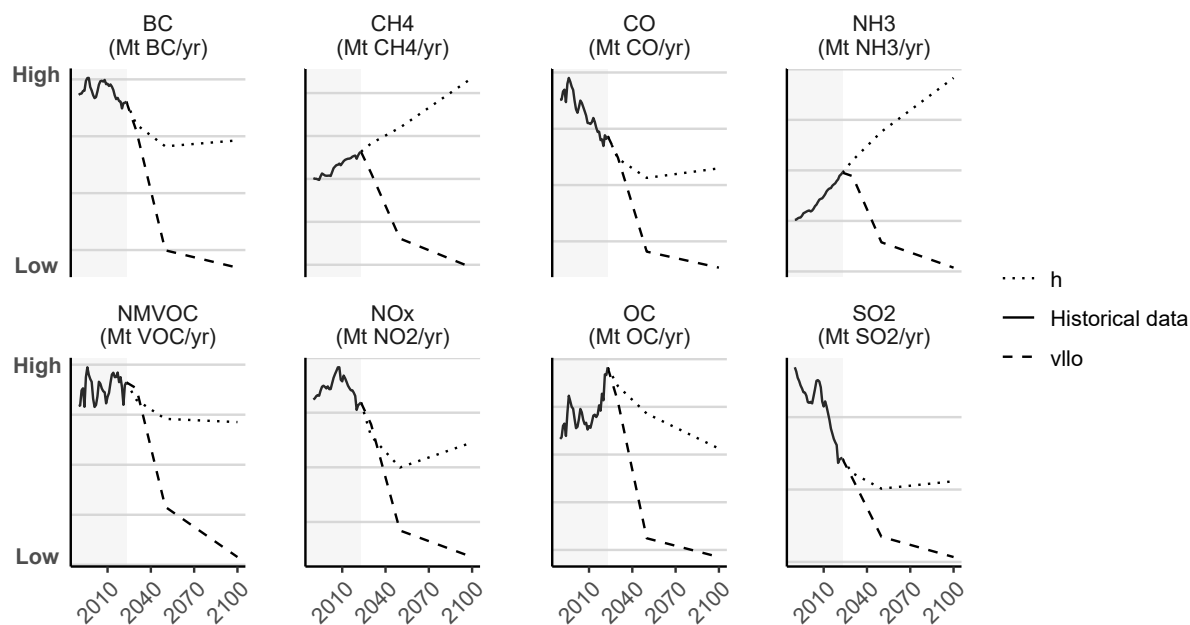
Figure 7. An indicative illustration of possible global trajectories for esm-scen7-vll0 ( esm-scen7-vl ( VLL0VL )) and esm-scen7-h (H) marker pathways in CMIP7 scenarios for 2023–2100. Shown are (a) primary energy split by different energy carriers, and (b) CH 4 and a set of selected SLCFs, harmonized to historical emissions for CMIP7 until 2023 inclusive.
