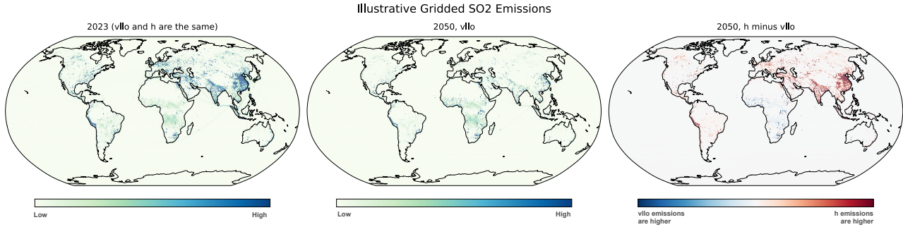
Figure 8. An indicative illustration of possible gridded SO 2 emissions for esm-scen7-v1o esm-scen7-vl ( V1LOVL ) and esm-scen7-h (H) marker pathways. Shown are the total emissions for (left to right) the harmonization year 2023 (end of historical data and start of scenarios), esm-scen7-v1o esm-scen7-vl in 2050, and their difference between esm-scen7-v1o esm-scen7-vl and esm-scen7-h for 2050. The emission totals include anthropogenic emissions at the surface, vertically integrated aircraft emissions, and open burning emissions.
