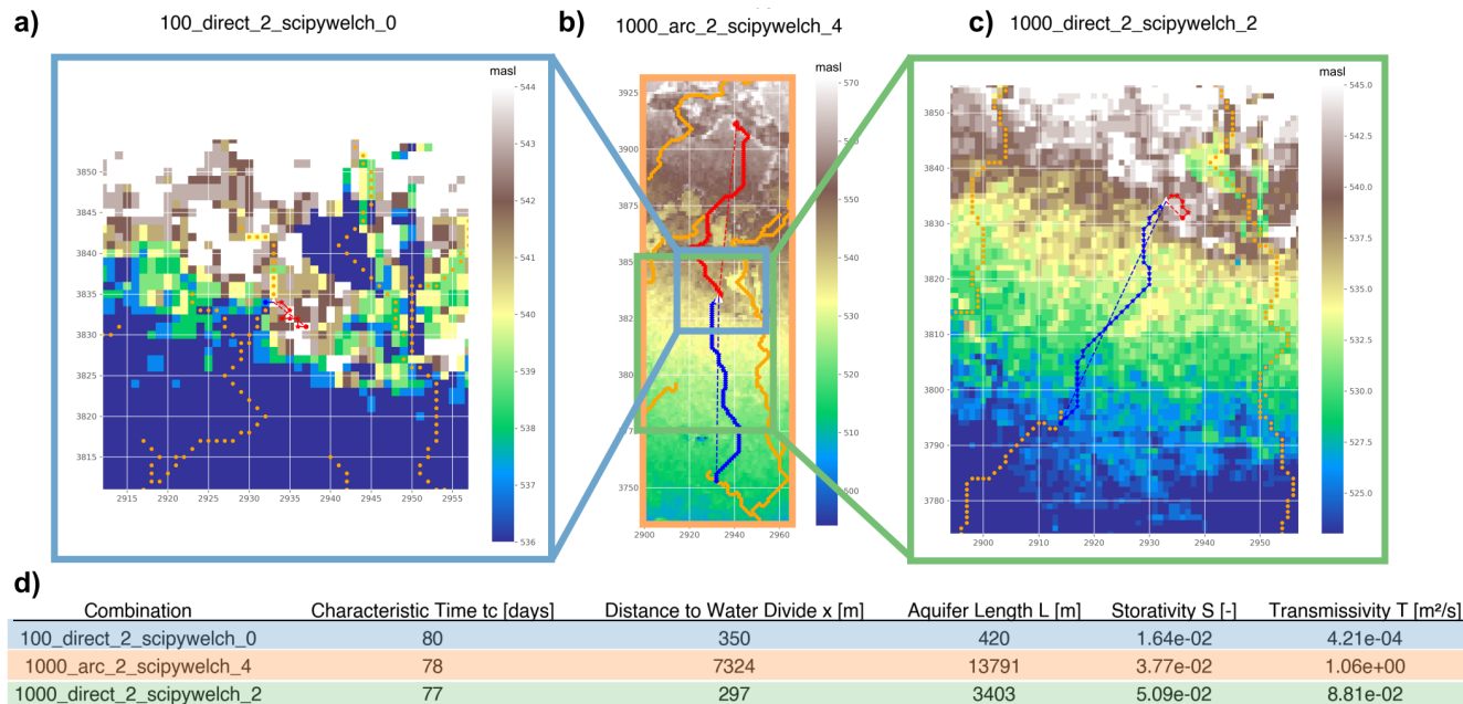
Figure A2. Resulting flow lines for three different parameter sets. (a) Flow lines generated with the smallest flow accumulation threshold (100), resulting in the shortest flow paths. Streams extend far into the hills, reducing the distance from the well to the nearest river (blue lines). With no smoothing applied to the flow direction, the upstream path terminates early (red lines). (b) The longest flow lines, produced using a higher flow accumulation threshold (1,000). Here, rivers appear less dendritic, and the distance from the well to the river increases. Strong smoothing of the flow direction (level 4) causes the upstream segment to reach higher elevations. The arc length (indicated by stars) is used to measure the path, in contrast to the direct connection (dashed lines). (c) A parameter set that yields flow lines of intermediate length, which is selected for further analysis in this study. (d) A table summarizing the key values for each parameter set. The distance to the water divide x represents the distance from the well to the water divide. The aquifer length L is defined as the sum of the upstream and downstream segments.
