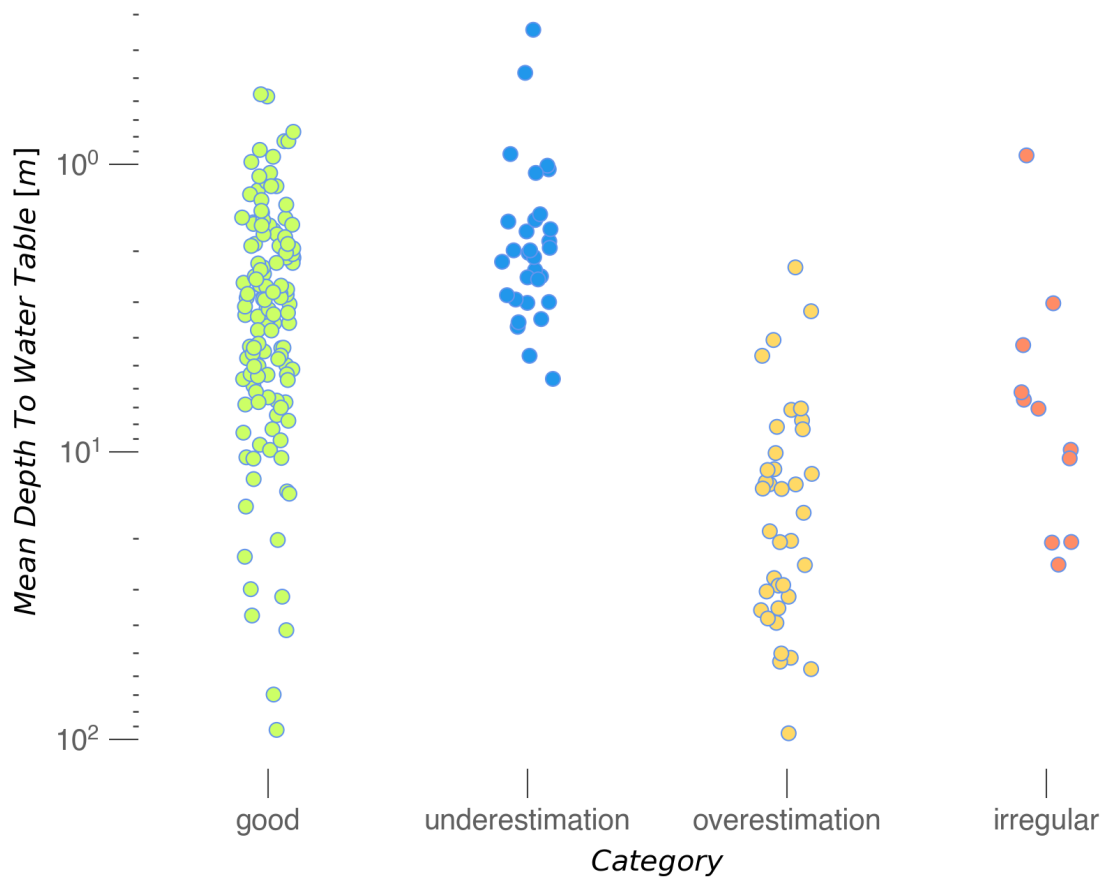
Figure 7. The four categories of the GoF in relation to the mean depth to the groundwater table. Good fitting spectra appear for across all depths. Shallow wells tend to be underestimated while deeper wells tend to be overestimated.
