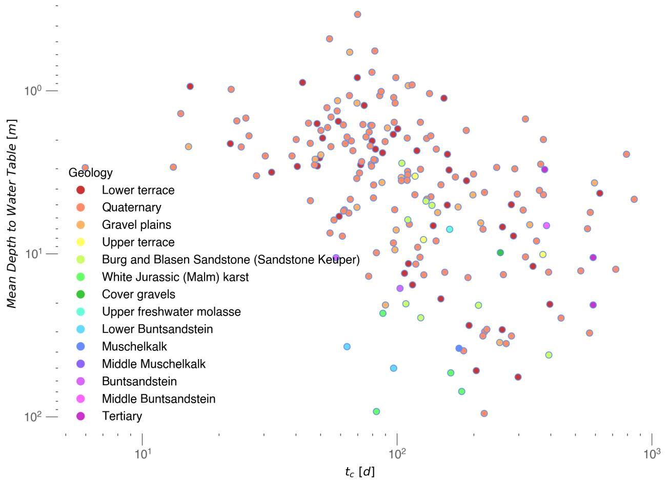
Figure 8. Scatter plot of depth to the water table (m) versus aquifer response time t_c (days), categorized by aquifer geology. Each point represents a groundwater well, with colors indicating different aquifer types.
