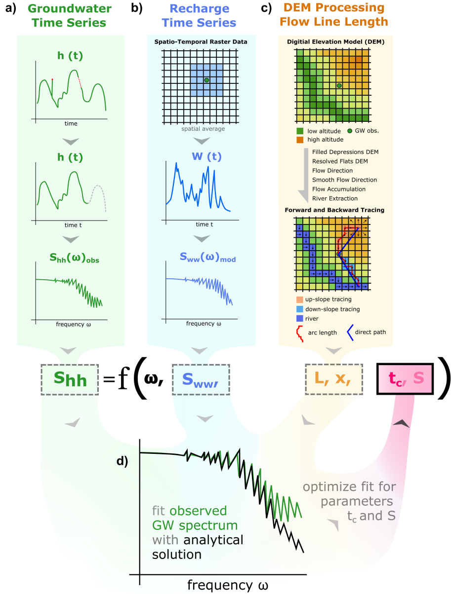
Figure 2. Overview of the spectral analysis (SpA) workflow. The aim is to acquire aquifer parameters based on the spectral representation response of groundwater and recharge time series, accompanied by geometric information of the aquifer (flow line length ) derived from DEM processing. a) Processing of groundwater level time Series and transfer to frequency domain, b) extraction of recharge time series from spatio-temporal simulations of the mesoscale hydrological model mHM and spatially averaged for shaded region, c) DEM processing and consecutive flow line (FL) estimation, d) measured groundwater level spectrum fitted with semi-analytical solution with t_c and S subject to optimization.
