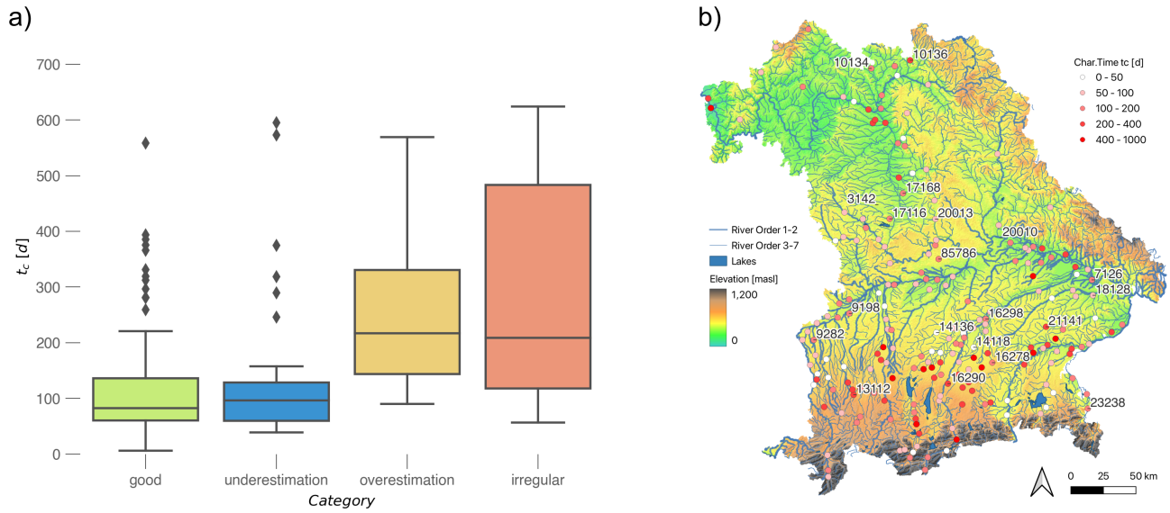
Figure 6. (a) Box plots of resulting aquifer response times for each category. Y-limits were trimmed and three outliers were cut off. (b) Map of Bavaria with SRTM OpenTopography (2013) as basemap and rivers from German Federal Institute for Hydrology - BfG (2022) showing the spatial distribution of obtained t_c .
