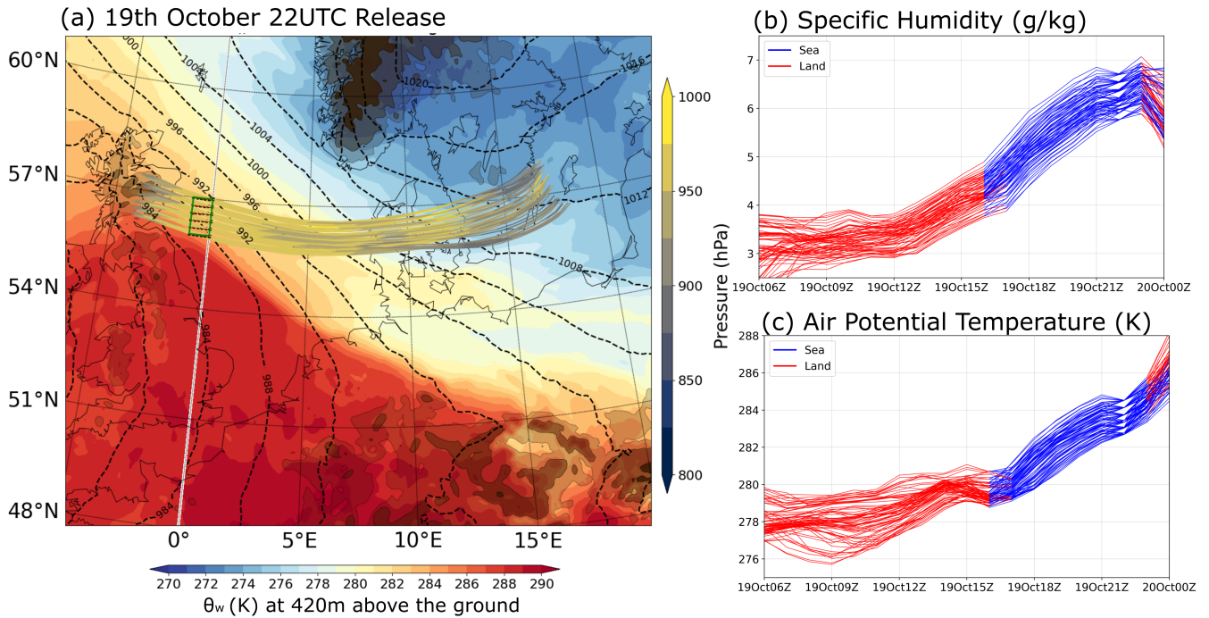
Figure 7. Same as Figure 6, but for trajectories released at 19 October 2023 22 UTC. In panel (a), \theta_w at 420 m and the sea-level pressure (hPa) field is valid at 19 October 2023 15 UTC.
