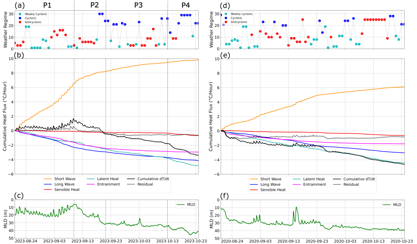
Figure 2. Atmospheric and oceanic drivers of 2023 MHW (left column, a-c) contrasted with conditions during the same period in the non-MHW year of 2020 (right column, d-f). The top panels show the evolution of the synoptic weather regime using a 30 regime classification for Northwest Europe (Neal et al., 2016); coloured by regime category: Weak (cyan), Low (blue), and High (red) (a, d). The middle panels show the cumulative heat flux tendency components in ^{\circ}\text{C}/\text{Hour} (b, e), including Shortwave (orange), Longwave (blue), Sensible Heat (red), Latent Heat (cyan), Entrainment (magenta), and a Residual (grey) term. The net cumulative temperature tendency (Cumulative dT/dt ) is shown in black. The bottom panels show the MLD in meters (c, f).
