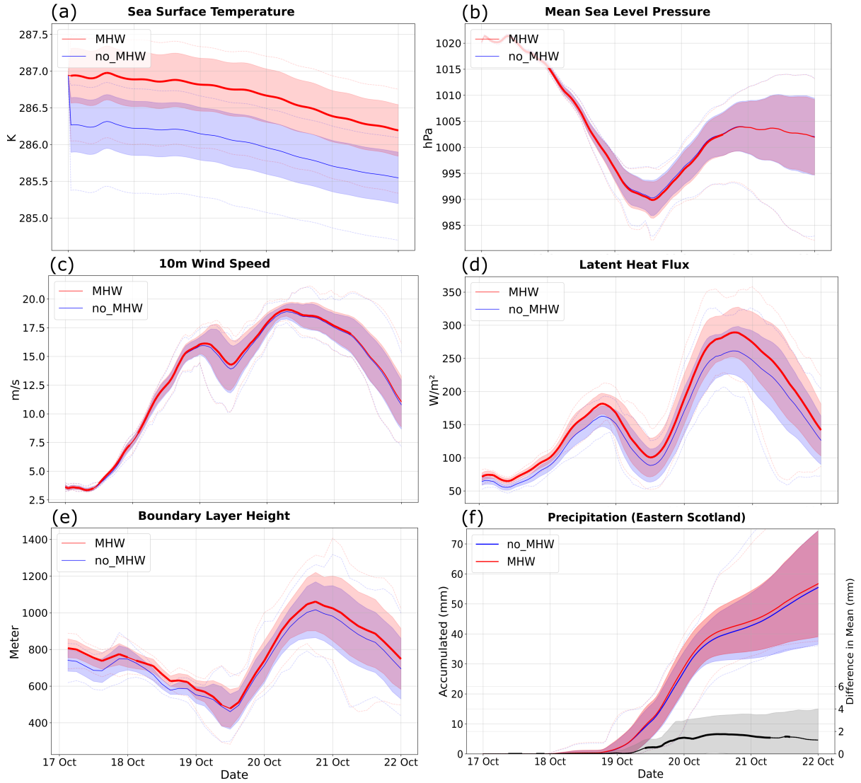
Figure 8. Time series comparing the MHW (red) and no_MHW (blue) 18-member ensemble simulations over the 5-day forecast period from 17-21 October. For each panel, solid lines represent the mean, dashed lines show the full ensemble range (minimum and maximum), and the shaded areas denote \pm 1 standard deviation. The panels display: (a) sea surface temperature (K), (b) mean sea level pressure (hPa), (c) 10-metre wind speed (m/s), (d) surface latent heat flux ( W/m^2 ), and (e) planetary boundary layer height (m), with each variable averaged over the Central North Sea. Panel (f) shows the accumulated precipitation over Eastern Scotland (red box in Figure 4, mm, left axis) and the difference between the ensemble means (MHW - no_MHW, black line, right axis). Thicker segments of the MHW line indicate statistical significance at the 99% confidence level ( p < 0.01 ) based on a paired t-test between corresponding ensemble members ( MHW_i - no\_MHW_i ). For precipitation in f, the significance is highlighted by a thick line on the difference plot (black line) for visibility.
