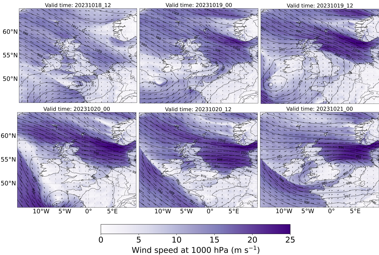
Figure 3. Synoptic evolution of Storm Babet shown via 12-hour forecast fields at selected times from 18 to 21 October 2023. Shading shows wind speed at 1000 hPa (m s -1 ), arrows show wind direction, and contours show mean sea-level pressure (hPa). The figure highlights the development of the storm and the persistent southeasterly flow over the North Sea prior to the heaviest rainfall over eastern Scotland.
