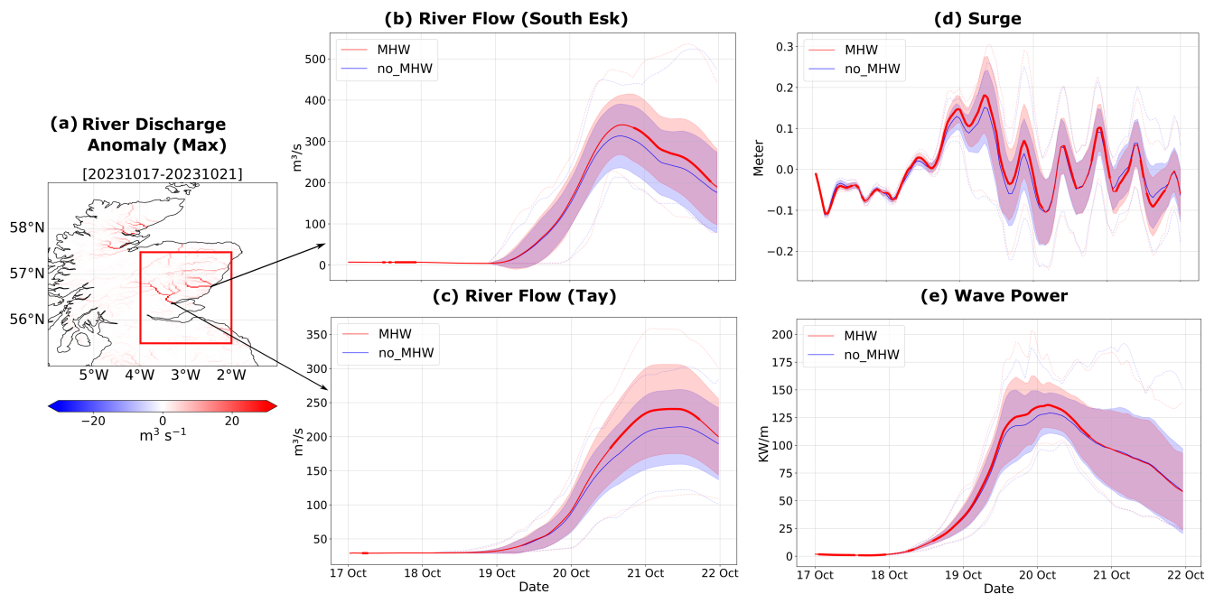
Figure 9. (a) Maximum river discharge anomaly (MHW – no_MHW) b) river flow in the mouth of river South Esk, (c) river flow in River Tay, d) surge on the Eastern Scotland red box (sea only), surge is computed using ocean model total water level - tide-only run, e) Wave power in Eastern Scotland red box (sea only). Thicker segments of the MHW line indicate statistical significance at the 99% confidence level ( p < 0.01 ) based on a paired t-test between corresponding ensemble members ( MHW_i - no\_MHW_i ).
