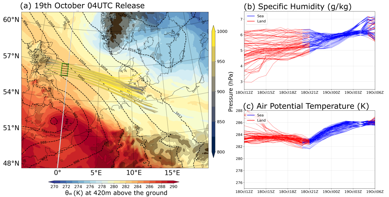
Figure 6. Air parcel trajectories and thermodynamic evolution for the 19 October 2023 04 UTC release. (a) Wet-bulb potential temperature ( \theta_w ) at 420 m above ground level, overlaid with sea-level pressure (hPa) valid on 18 October 21 UTC (midpoint of the trajectory) and 18-hour trajectories (16-hour backward + 2-hour forward) released from 56.0°N-57.0°N, 1.0°W-0.0°E at 925-970 hPa. (b) Specific humidity (g/kg) along the trajectories. (c) Air potential temperature (K). Red: Parcels over land; Blue: Parcels over the ocean.
