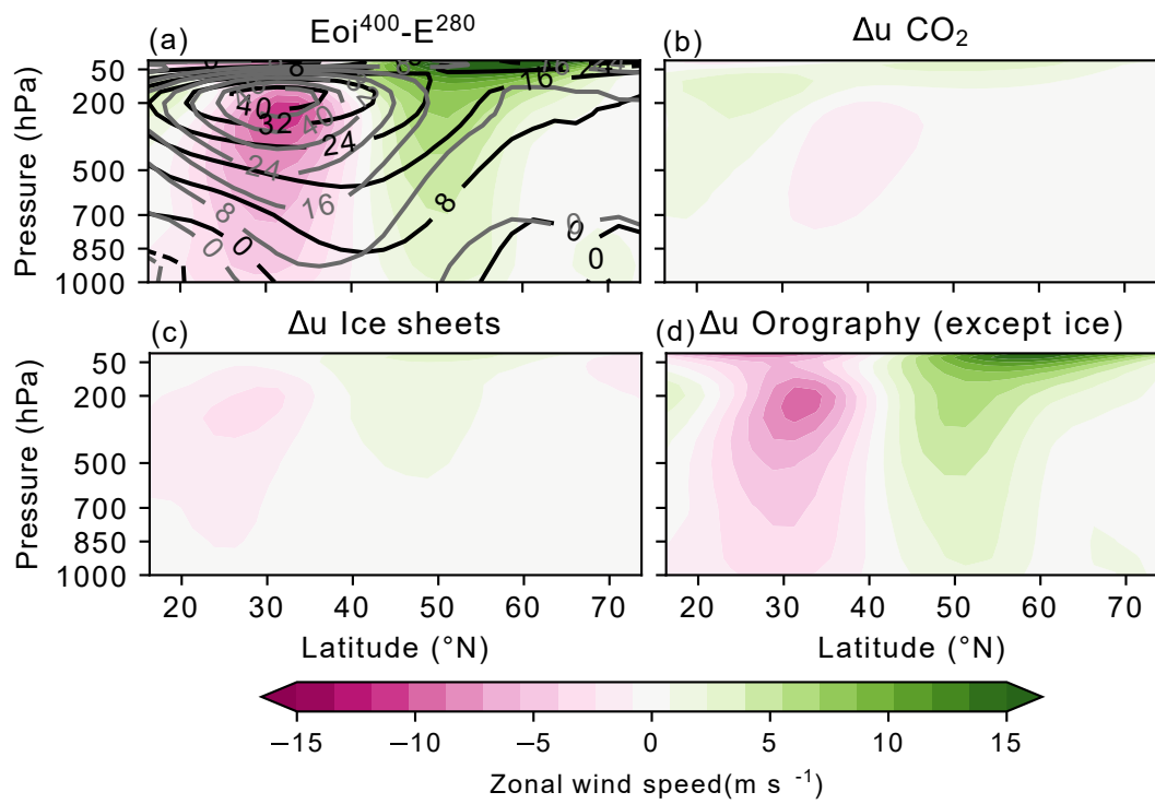
Figure 5. Change in boreal winter (DJF), zonally averaged, North Pacific zonal wind speed between the Late Pliocene ( Eoi^{400} ) and the Pre-industrial ( E^{280} ) in HadCM3 and the contribution of the change from CO_2 , ice sheet and orography forcings to the total change. In plot (a) the grey contours represent the E^{280} values and the black contours represent the Eoi^{400} values.
