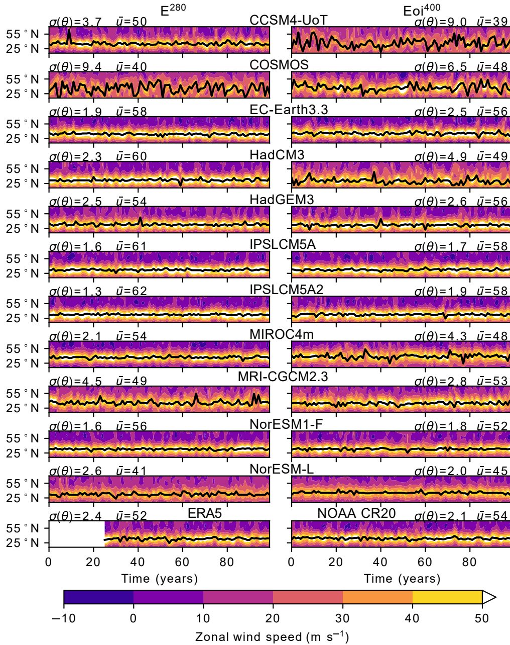
Figure 8. Hovmöller diagrams for the zonal mean wind speed at 200hPa-200hPa in January for 100 years for the North Pacific. The left-hand side is from the PI-E 280 (pre-industrial) experiments and the right-hand side is from the LP-Eoi 400 (Late Pliocene) experiments with the exception of the bottom two panels which show the reanalysis data. The dashed-black line indicates the latitude of maximum zonal wind speed. The standard deviation in the latitude ( \sigma(\theta) ) and mean maximum zonal wind speed ( \bar{u} ) are shown for each subplot.
