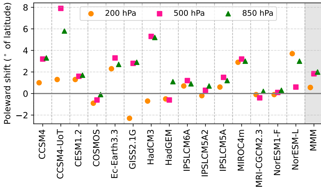
Figure 2. Poleward shift of the latitude of maximum zonal wind in the North Pacific region in boreal winter (DJF) at three pressure levels across all the models and the multi-model mean (MMM) . Positive values indicated the jet is poleward in the Late Pliocene experiments compared to the pre-industrial control simulations.
