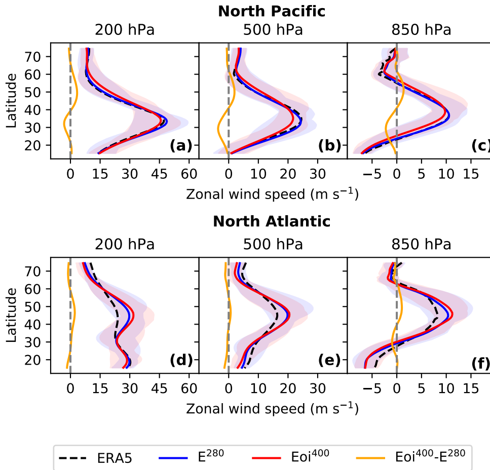
Figure 1. Multi-model Boreal winter (DJF), multi-model mean zonal wind speeds for the PI-pre-industrial (blue E^{280} ), LP-Late Pliocene (red E^{oi^{400}} ) and LP-PI the anomaly (orange E^{oi^{400}} - E^{280} ). ERA5 reanalysis data is shown in the dashed black line. A-C (a)-(c) is for the North Pacific region and D-F (d)-(f) is for the North Atlantic. Shading represents the multi model range.
