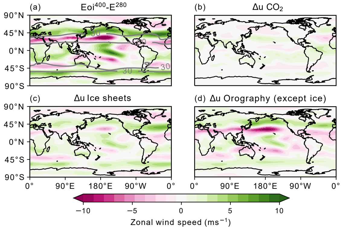
Figure 4. Change in 200hPa-boreal winter (DJF) 200 hPa zonal wind speed between the Late Pliocene ( Eoi^{400} ) and the Pre-industrial ( E^{280} ) in HadCM3 and the contribution of the change from \text{CO}_2 , ice sheet and orography forcings forcing to the total change. In plot (a) the grey contours show the 30 \text{ m s}^{-1} value in the E^{280} experiment.
