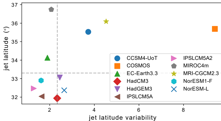
Figure 7. Latitude of maximum zonal wind speed and standard deviation of this latitude ( jet latitude variability ) in the PlioMIP2 PI-E 280 ( pre-industrial ) simulations compared to the ERA5 reanalysis data (dashed gray-grey lines) in the North Pacific region for January .
