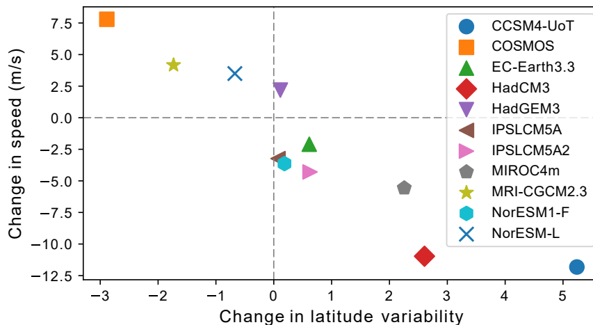
Figure 9. Change in the mean speed of the January North Pacific jet stream and the change in the variability of the jet stream position. Each model in the ensemble is labelled. The dashed gray lines divide the graph into quadrants, where the upper left section shows models with an increased speed and decreased variability and the lower right quadrant contains models with a slower speed and increased variability.
