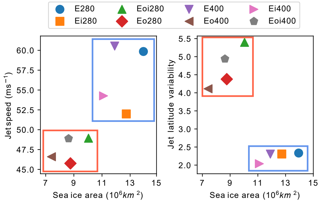
Figure 11. January Northern Hemisphere sea ice area and January North Pacific jet stream speed ( left ), and jet latitude variability ( right ) at 200 hPa in HadCM3. The red box groups experiments with Late Pliocene orography and the blue box groups experiments with pre-industrial orography.
