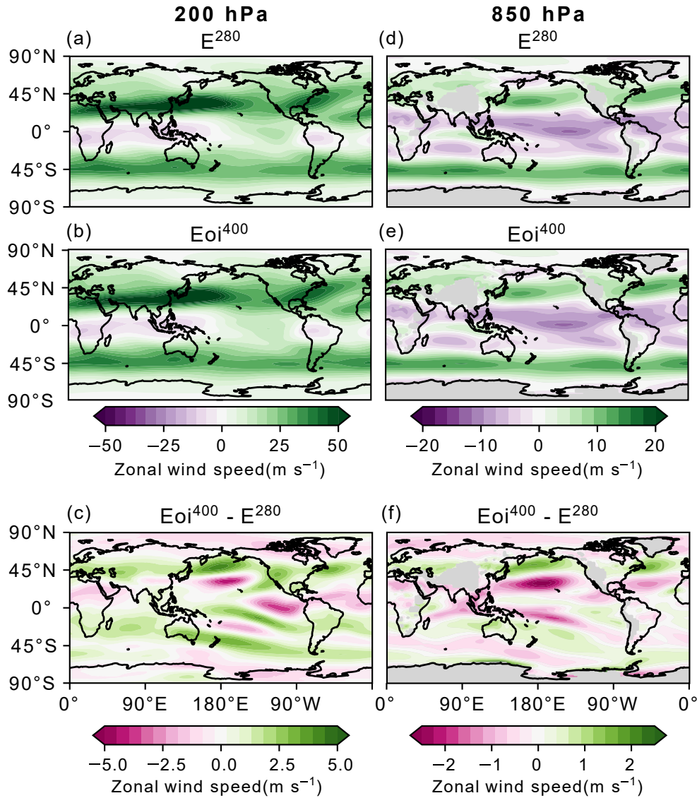
Figure 3. Multi-model mean zonal wind speeds for 200hPa-200 hPa (left) and 850hPa-850 hPa (right). The lower plots show the difference between the Late Pliocene ( Eoi 400 ) and the Pre-Industrial ( E 280 ). Note the difference in scales between the two pressure levels.
