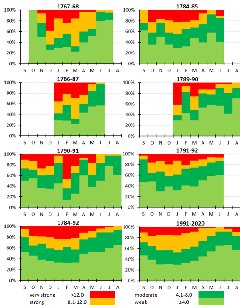
Fig. 3. Day-to-day variation in atmospheric pressure for the historical period Nuuk (according to daily averages). Graph for individual months, seasons and years, cumulated to 100%
