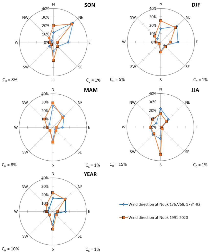
Fig. 7. Seasonal (SON, DJF, etc. MAM, JJA) and annual (YEAR) frequencies (in %) of wind directions and calms (C) at Nuuk in historical (1767/68; 1784–92) and contemporary (1991–2020) periods
