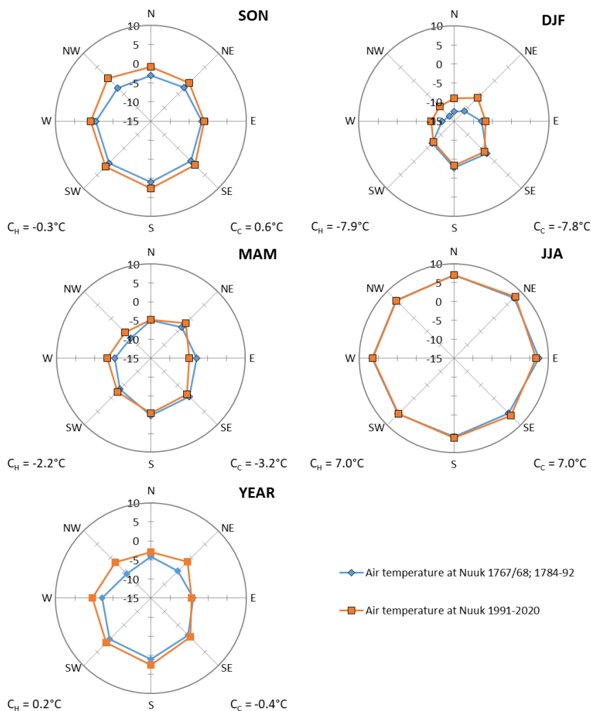
Fig. 8. Seasonal (SON, DJF, etc. MAM, JJA) and annual (YEAR) average values of air temperature (in °C) according to different directions at Nuuk in historical (1767/68; 1784–92) and contemporary (1991–2020) periods
