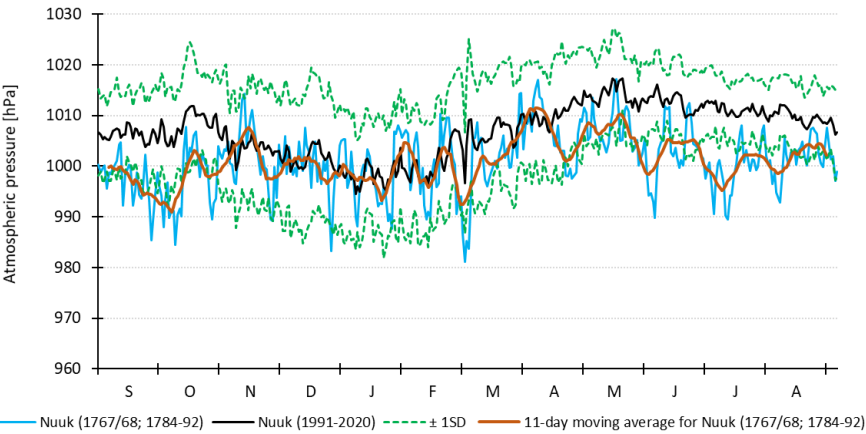
262 263 Fig. 4. Annual course of daily means of atmospheric pressure and 11-day moving average at Nuuk in 264 the historical (1767/68; 1784–92) and contemporary (1991–2020) periods, along with the standard 265 deviation 266 Explanations: SD – standard deviation ( \pm 1SD )
