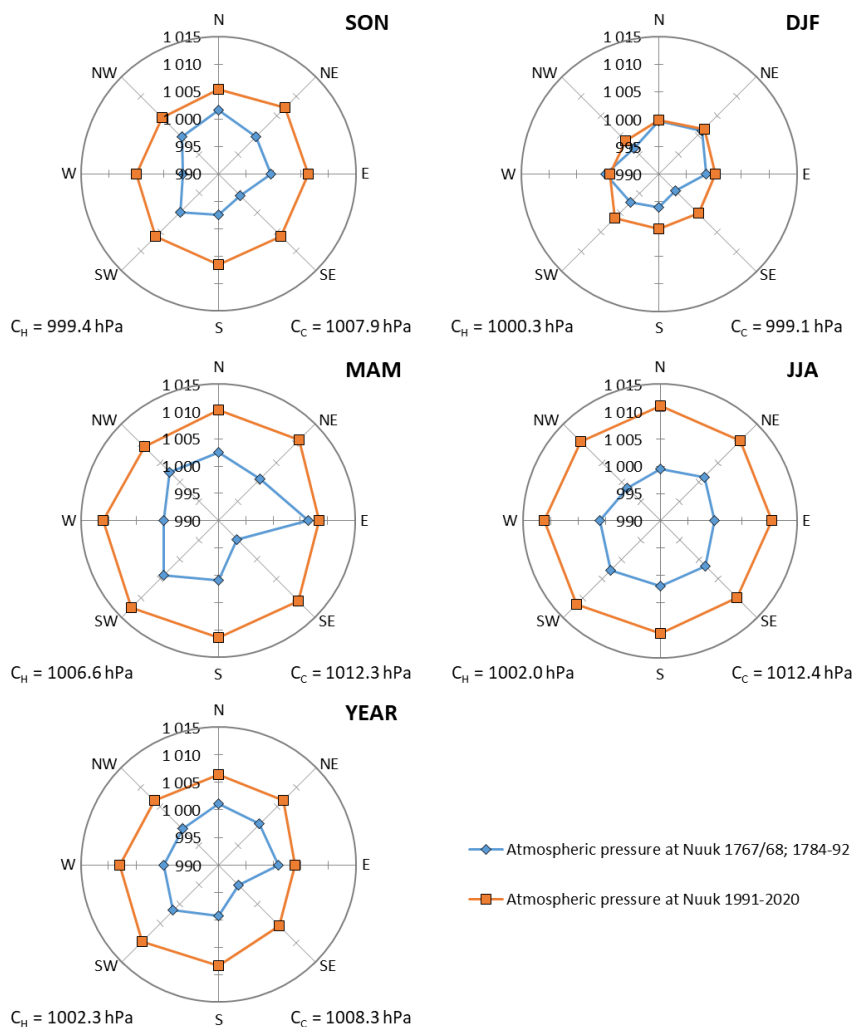
Fig. 9. Seasonal (SON, DJF, etc. MAM, JJA) and annual (YEAR) average values of air pressure (in hPa) according to wind direction at Nuuk in historical (1767/68; 1784–92) and contemporary (1991–2020) periods
