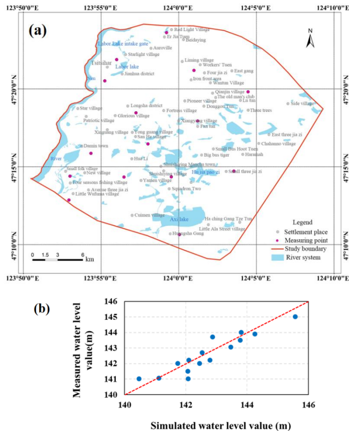
295 Figure 5. (a) Distribution of groundwater level measurement points in 2020; (b) Fitting diagram between simulated water level and measured data
