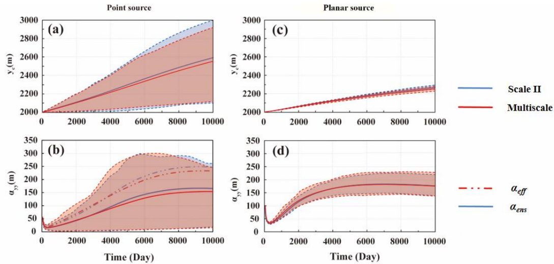
330 Figure 6. Results of Temporal evolution of longitudinal (a, c) solute transport distances distance y_c(t) and (b, d) macro-dispersivity on two scales with time under two release conditions \alpha(t) for multiscale (red) and Scale II (blue) models under point-source release (a, b) and planar-source release (c, d) conditions. Solid lines denote ensemble means, and shaded envelopes represent the 10th–90th percentile ranges.
