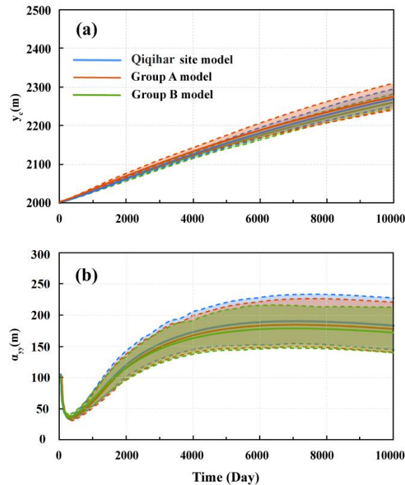
Figure 7. Results Effect of lithofacies proportions on longitudinal (a) solute transport distances distance y_c(t) and (b) macro-dispersivity \alpha(t) under different lithofacies volume proportion scenarios planar-source release condition. Group A and Group B represent more mixed and fine-dominated architectures, respectively. Solid lines denote ensemble means, and shaded envelopes represent the 10th–90th percentile ranges.
