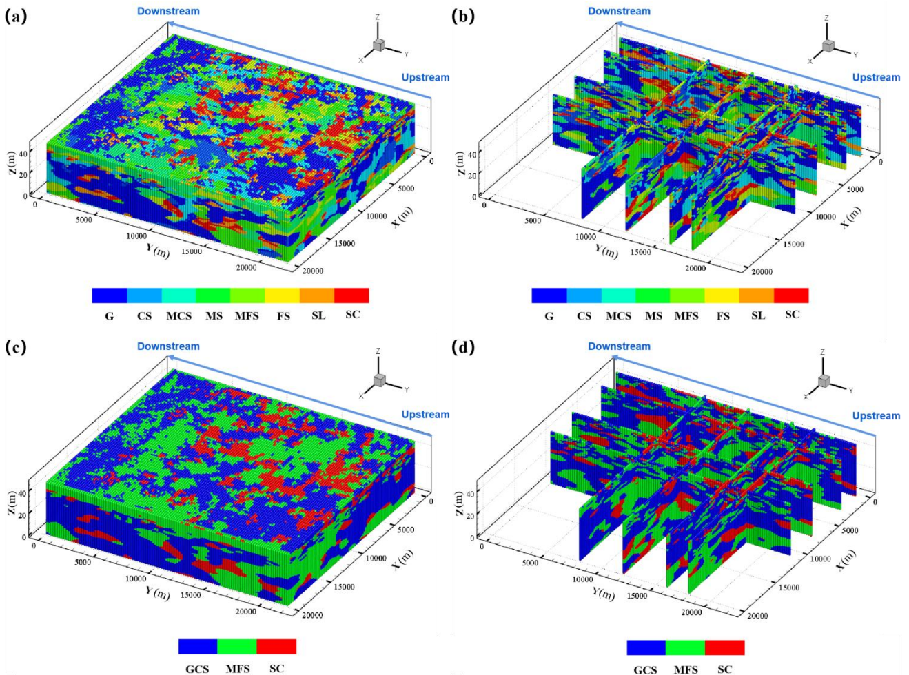
Figure 3. An example of multiscale model: (a) 3-D facies, (b) 2-D sections; and Scale II model: (c) 3-D facies, (d) 2-D sections. Section lines are located at x = 600\text{m}, 3000\text{m}, 7600\text{m}, 11000\text{m} and y = 8000\text{m}, 12000\text{m}, 16000\text{m}, 18000\text{m}
