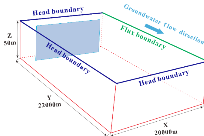
245 Figure 4. Conceptual hydrogeologic model of the study area and schematic diagram of solute plume planar source release conditions. The left side corresponds to the Nen River, and the pollution source is oriented approximately perpendicular to the regional groundwater flow direction.
