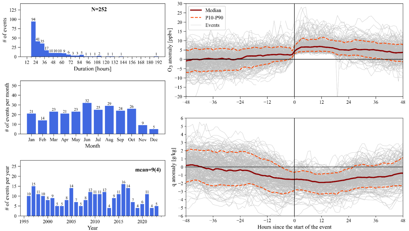
4 5 Figure 5. SUTO events as detected at Tololo according to anomalies in ozone (positive) and water vapor (negative). The 6 upper left panel shows the number of events according to duration in hours. The middle-left panel describes the seasonal distribution 7 considering all events occurring in each month. The bottom left panel indicates the number of events per year between November 8 1995 and December 2023. To the right we show the behavior of each event (grey thin lines) as well as their statistics per percentile: 9 10 (dashed orange line), 50 (dark red line) and 90 (dashed orange line). The upper (lower) right panel shows the statistics for ozone 10 (water vapor mixing ratio).
