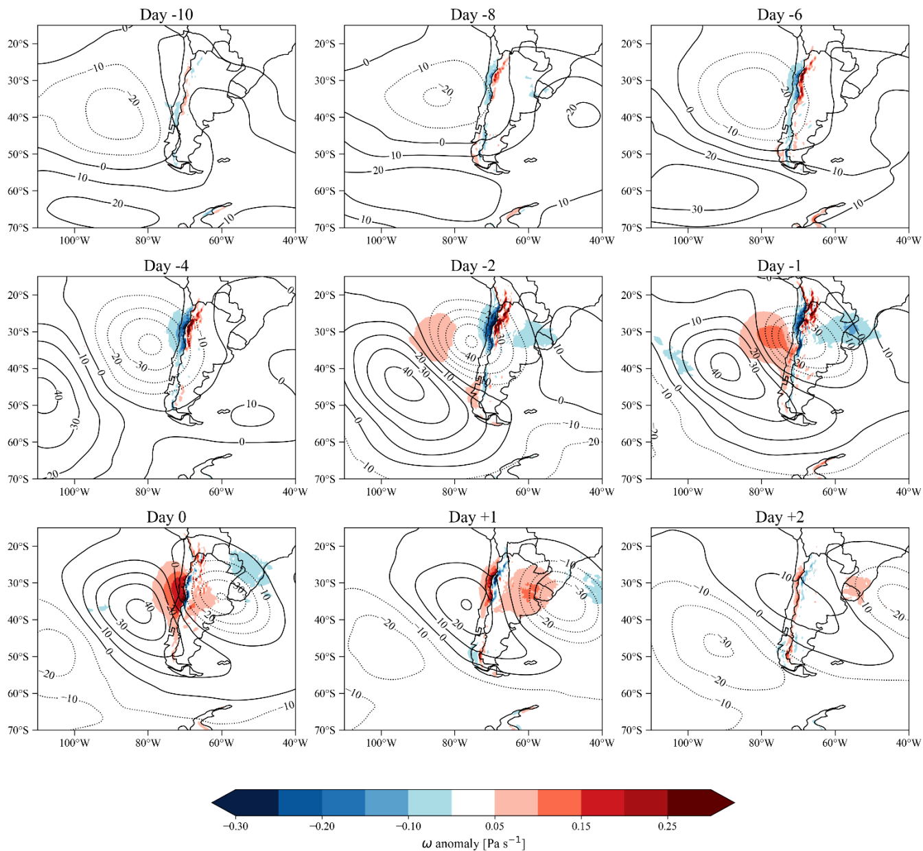
3 4 Figure 6. Composite maps of geopotential height and vertical velocity anomalies at 500 hPa during SUTO events. Contours 5 denote geopotential height anomalies in meters, where positive (negative) anomalies are solid (dotted) contours. Shaded areas denote 6 vertical velocity anomalies in Pa/s.
