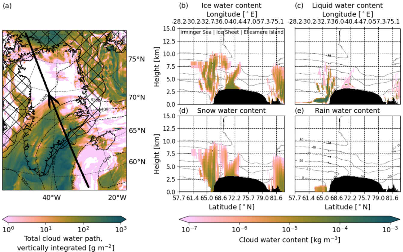
Figure 7. Modelled cloud scene on May 13th, 2025, 03:10 UTC. (a) Total cloud water path, vertically integrated [ \text{g m}^{-2} ], as simulated by RACMO. The thick black line shows the EarthCARE overpass. The contours of the 500 hPa geopotential height [m] levels are shown in dashed black lines. The hatched area indicates the presence of sea ice (sea ice extent larger than 15%). (b-e) Cloud water content [ \text{kg m}^{-3} ] as simulated by RACMO, for the co-located satellite overpass shown in (a) , for (b) cloud ice, (c) cloud liquid water, (d) cloud snow and (e) cloud rain. The dotted lines indicate the -50^{\circ}\text{C} to 0^{\circ}\text{C} temperature isotherms. Note that in (b-e) the x-axis follows the time coordinates. Hence, the latitude and longitude coordinates do not vary monotonically. In (b-e) , black areas correspond to the topography.
