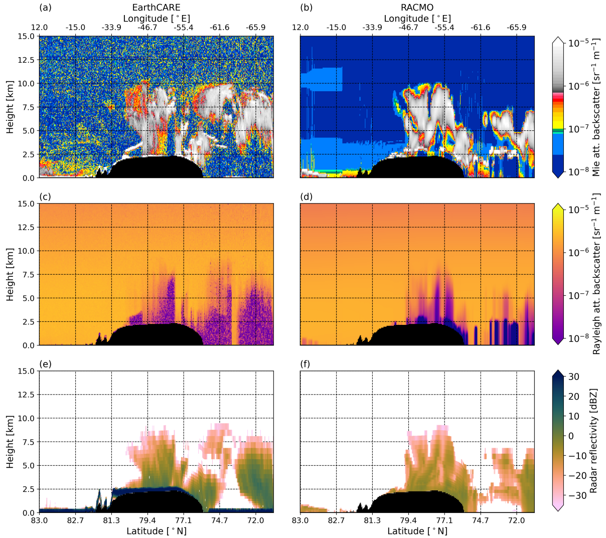
Figure 3. Profiles of the March 12th, 2025, 19:48 UTC (a,c,e) observed (EarthCARE, (a,c) ATL-NOM, baseline BA and (e) CPR-NOM, baseline CA) and (b,d,f) modeled (RACMO) (a-b) Mie attenuated backscatter [ \text{sr}^{-1} \text{m}^{-1} ], (c-d) Rayleigh attenuated backscatter [ \text{sr}^{-1} \text{m}^{-1} ] and (e-f) radar reflectivity [dBZ]. Note that the x-axis follows the time coordinates. Hence, the latitude and longitude coordinates do not vary monotonically. Also note that in (a-d) , the vertical resolution is 100 m, while in (e-f) the vertical coordinates follow the RACMO hybrid-sigma levels. Black areas correspond to the topography.
