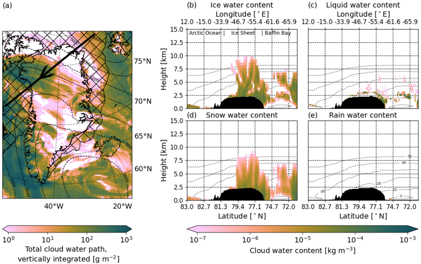
Figure 2. Modeled cloud scene on March 12th, 2025, 19:48 UTC. (a) Total cloud water path, vertically integrated [ \text{g m}^{-2} ], as simulated by RACMO. The thick black line shows the EarthCARE overpass. The contours of the 500 hPa geopotential height [m] levels are shown in dashed black lines. The hatched area indicates the presence of sea ice (sea ice extent larger than 15%). (b-e) Cloud water content [ \text{kg m}^{-3} ] as simulated by RACMO, for the co-located satellite overpass shown in (a) , for (b) cloud ice, (c) cloud liquid water, (d) cloud snow and (e) cloud rain. The dotted lines indicate the -50^{\circ}\text{C} to 0^{\circ}\text{C} temperature isotherms. Note that in (b-e) the x-axis follows the time coordinates. Hence, the latitude and longitude coordinates do not vary monotonically. In (b-e) , black areas correspond to the topography.
