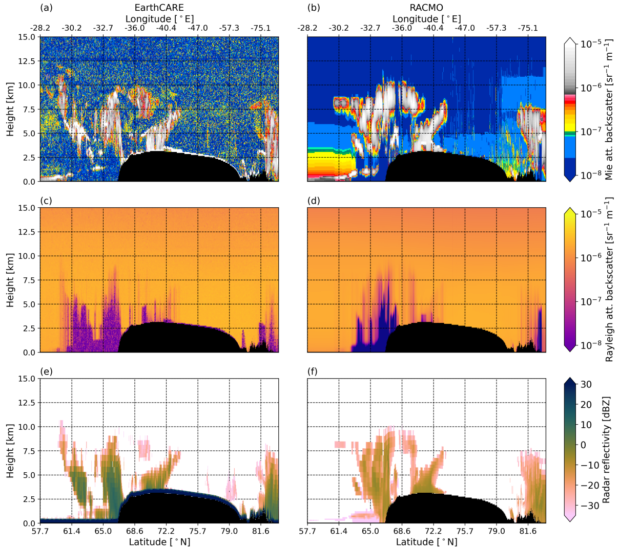
Figure 8. Profiles of the May 13th, 2025, 03:10 UTC (a,c,e) observed (EarthCARE, (a,c) ATL-NOM, baseline BA and (e) CPR-NOM, baseline CB) and (b,d,f) modeled (RACMO) (a-b) Mie attenuated backscatter [ \text{sr}^{-1}\text{m}^{-1} ], (c-d) Rayleigh attenuated backscatter [ \text{sr}^{-1}\text{m}^{-1} ] and (e-f) radar reflectivity [dBZ]. Note that the x-axis follows the time coordinates. Hence, the latitude and longitude coordinates do not vary monotonically. Also note that in (a-d), the vertical resolution is 100 m, while in (e-f) the vertical coordinates follow the RACMO hybrid-sigma levels. Black areas correspond to the topography.
