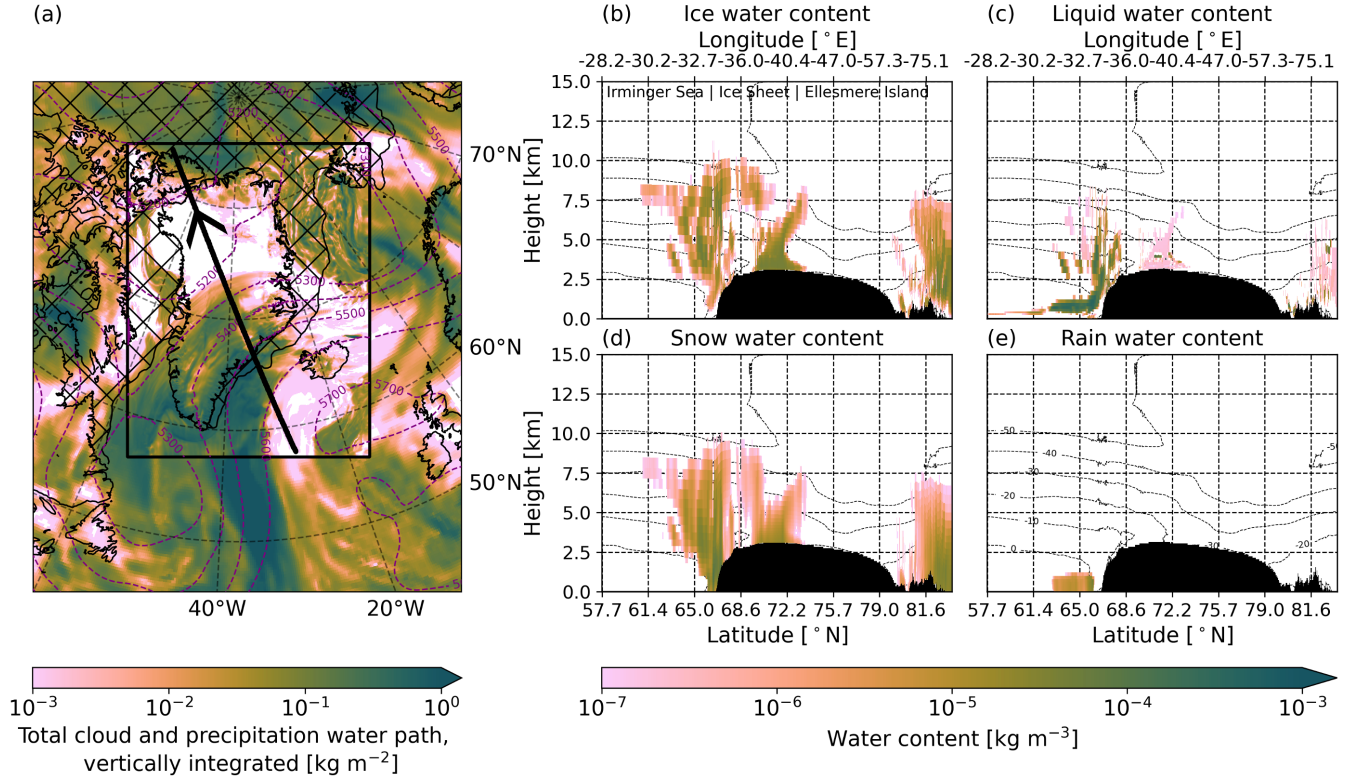
Figure 7. Modelled cloud scene on May 13th, 2025, 03:10 UTC. (a) Total cloud water path, vertically integrated [kg m -2 ], as simulated by RACMO (within the black box) and ERA5 (at 03:00 UTC, outside the black box). The thick black line shows the EarthCARE overpass. The contours of the 500 hPa geopotential height [m] levels are shown in dashed purple lines. The hatched area indicates the presence of sea ice (sea ice extent larger than 15%). (b-e) Water content [kg m -3 ] as simulated by RACMO, for the co-located satellite overpass shown in (a), for (b) cloud ice, (c) cloud liquid water, (d) snow and (e) rain. The dotted lines indicate the -50°C to 0°C temperature isotherms. Note that in (b-e) the x-axis follows the time coordinates. Hence, the latitude and longitude coordinates do not vary monotonically. In (b-e), black areas correspond to the topography.
