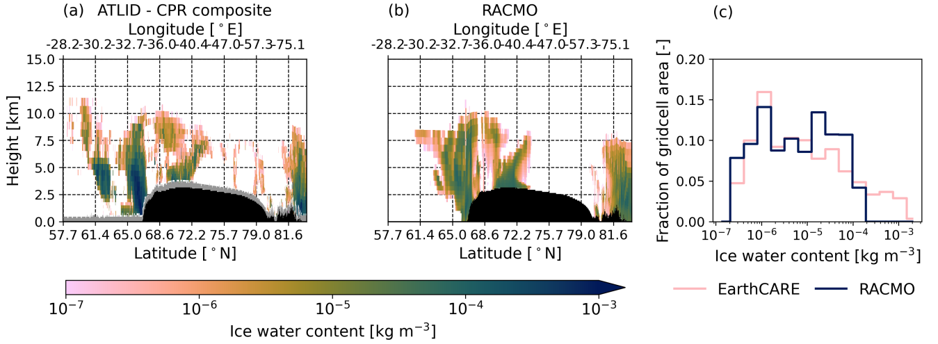
Figure 10. Ice water content [kg m -3 ] from (a) ATLID-CPR (from ATL-ICE and CPR-CLD, baseline BA) composite and (b) RACMO (including snow water content) for May 13th, 2025, 03:10 UTC. (c) shows the gridcell area-weighted histogram of ice water content for EarthCARE (pink, ATLID-CPR composite) and RACMO (blue, including snow water content). When computing the histograms, areas that suffer from surface clutter are masked out in both the EarthCARE and RACMO profiles. Note that in (a-b) the x-axis follows the time coordinates. Hence, the latitude and longitude coordinates do not vary monotonically. In (a-b), black areas correspond to the topography. In (a), gridcells classified as surface clutter are masked in grey.
