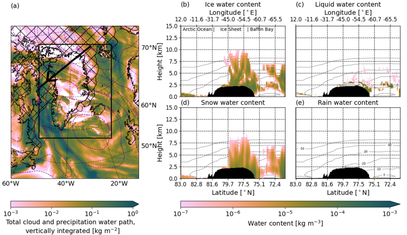
Figure 2. Modeled cloud scene on March 12th, 2025, 19:48 UTC. (a) Total cloud water path, vertically integrated [kg m -2 ], as simulated by RACMO (within the black box) and ERA5 (at 20:00 UTC, outside the black box). The thick black line shows the EarthCARE overpass. The contours of the 500 hPa geopotential height [m] levels are shown in dashed purple lines. The hatched area indicates the presence of sea ice (sea ice extent larger than 15%). (b-e) Water content [kg m -3 ] as simulated by RACMO, for the co-located satellite overpass shown in (a), for (b) cloud ice, (c) cloud liquid water, (d) snow and (e) rain. The dotted lines indicate the -50°C to 0°C temperature isotherms. Note that in (b-e) the x-axis follows the time coordinates. Hence, the latitude and longitude coordinates do not vary monotonically. In (b-e), black areas correspond to the topography.
