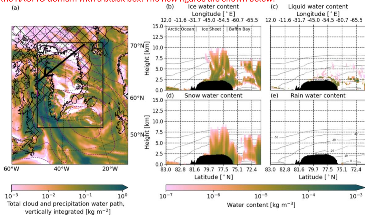
Figure 2. Modeled cloud scene on March 12th, 2025, 19:48 UTC. (a) Total cloud and precipitation water path, vertically integrated [kg m -2 ], as simulated by RACMO (within the black box) and ERA5 (at 20:00 UTC, outside the black box). The thick black line shows the EarthCARE overpass. The contours of the 500 hPa geopotential height [m] levels are shown in dashed purple lines. The hatched area indicates the presence of sea ice (sea ice extent larger than 15%). (b-e) Water content [kg m -3 ] as simulated by RACMO, for the co-located satellite overpass shown in (a), for (b) cloud ice, (c) cloud liquid water, (d) snow, and (e) rain. The dotted lines indicate the -50°C to 0°C temperature isotherms. Note that in (b-e) the x-axis follows the time coordinates. Hence, the latitude and longitude coordinates do not vary monotonically. In (b-e), black areas correspond to the topography.
