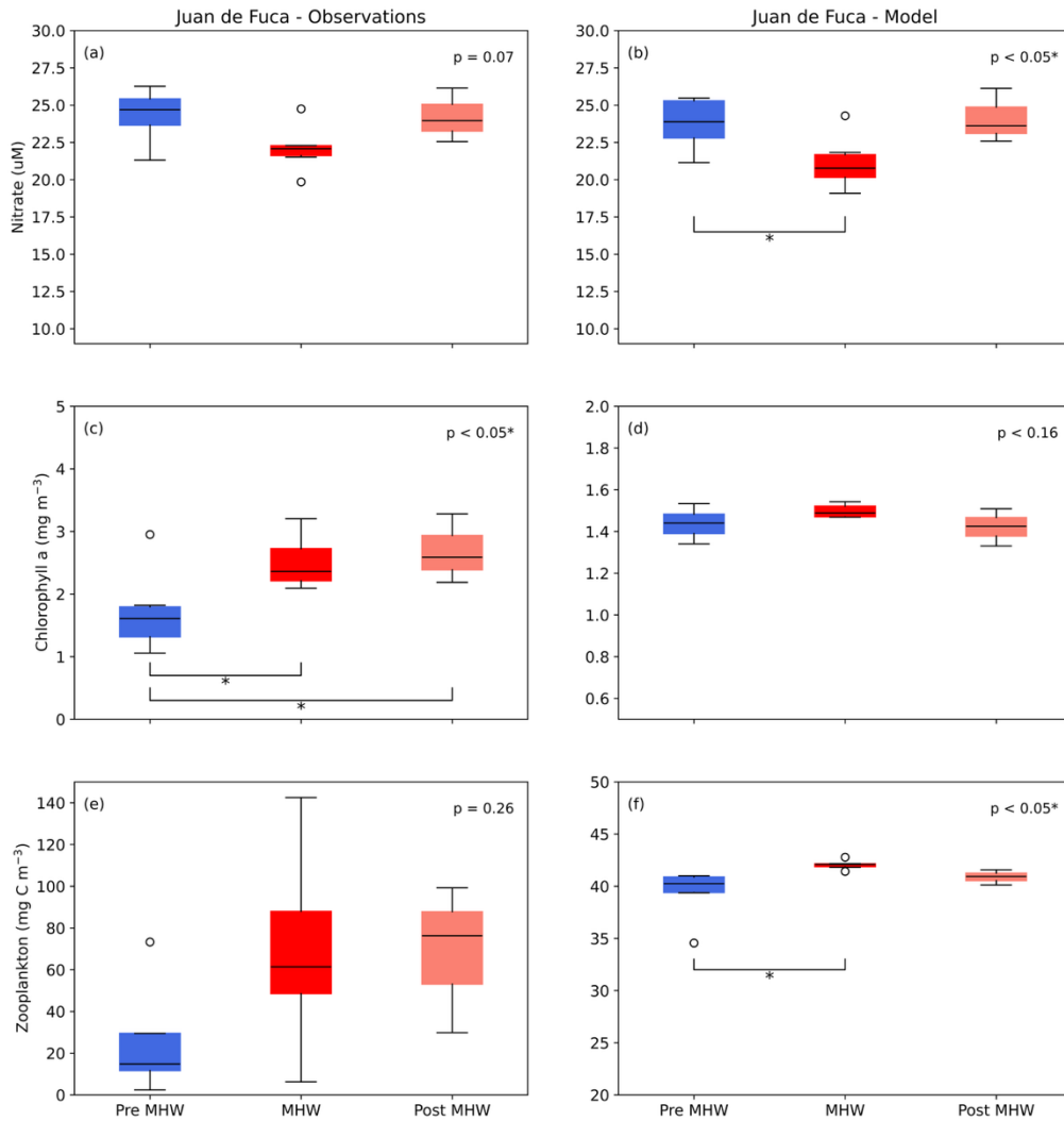
495 Figure 12: Mean 0-10 m nitrate concentration, 0-50 m chlorophyll a biomass, and full water column zooplankton biomass pre-marine heatwave years (Pre MHW; 2007-2013), marine heatwave years (MHW; 2014-2019), and post-marine heatwave years (Post MHW; 2020-2022) for observation and data in the Juan de Fuca Strait region. Vertical scales differ between observed and modelled chlorophyll a and zooplankton to account for the higher and more variable observations, as shown in previous model evaluations (Olson et al. 2020, Suchy et al. 2023). * = significant at p < 0.05 ; ** significant at p < 0.01 ; *** significant at p < 0.001 .
