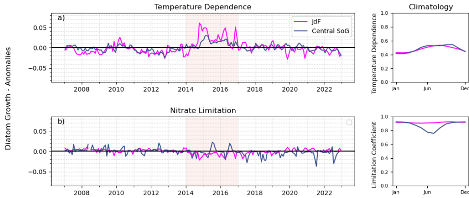
735 Figure 9. Left panels: anomalies in a) temperature dependence, and b) nitrate limitation on diatom growth in the 0-50 m depth layer compared to the 16-year climatology (2007-2022; right panels) in the Juan de Fuca and Central Strait of Georgia regions. Positive anomalies mean less limitation or temperature dependence compared to climatology; negative anomalies reflect more limitation or temperature dependence.
