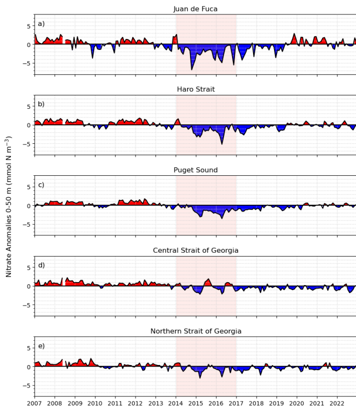
490 Figure 7: Mean model-based 0-50 m nitrate anomalies in the different sub-regions of the Salish Sea from 2007 to 2022. Nitrate anomalies for the 50-150m and 150m to bottom depth ranges are provided in supplemental material (Figs. S3-S4).
