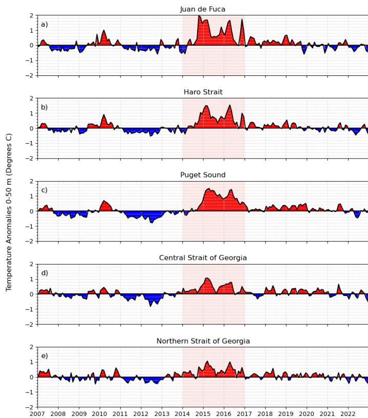
365 Figure 4: Mean model-based 0-50 m temperature anomalies in the different sub-regions of the Salish Sea from 2007 to 2022. Temperature anomalies for the 50-150m and 150m to bottom depth ranges are provided in supplemental material (Figs. S1-S2).
