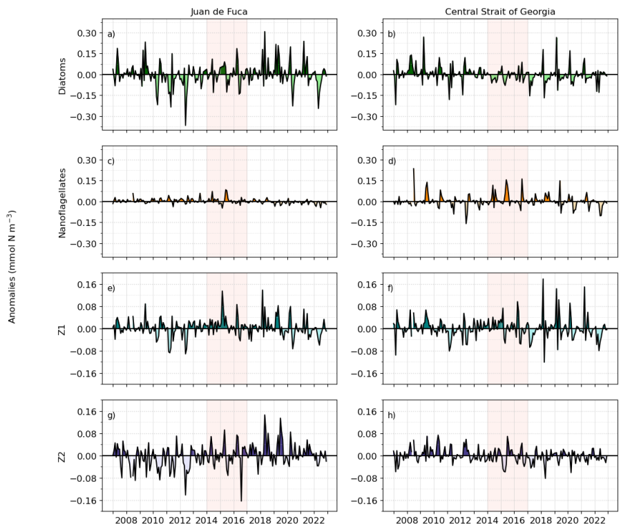
645 Figure 8: Anomalies in mean model-based 0-50 m biological parameters (diatoms, nanoflagellates, Z1, and Z2 zooplankton) in the Juan de Fuca and Central Strait of Georgia regions from 2007 to 2022. For anomalies including the seasonal cycle see Fig. S5.
