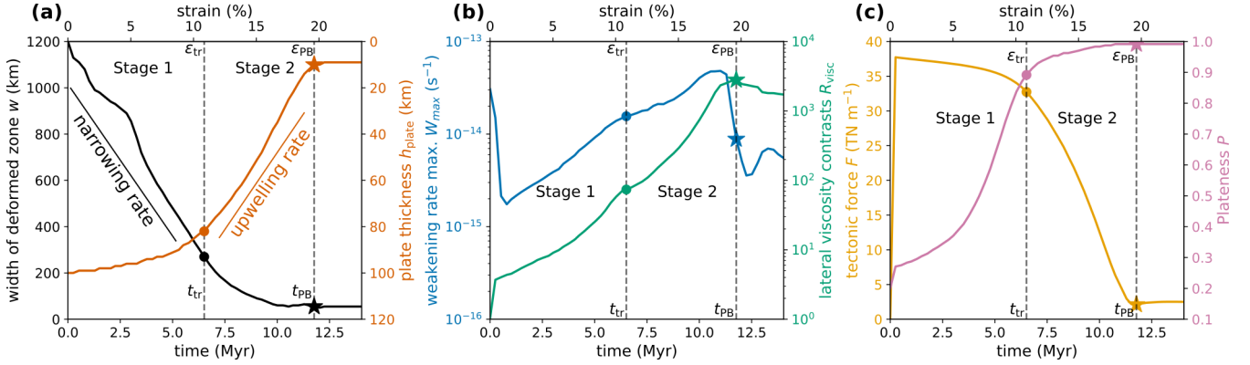
Figure 5. Results for Simulation D - d_{LT-HT} - Y_{500 \text{ MPa}}, \text{ref-1} . (a) Temporal evolution (and corresponding cumulative strain in %) of the width of deformed zone w (black) and minimum lithosphere thickness (orange) as defined in Sect. 3.1. Average narrowing and upwelling rates are calculated for Stage 1 and Stage 2, respectively. Rates can be expressed in \text{km Myr}^{-1} or in \text{cm yr}^{-1} (where 1 \text{ cm yr}^{-1} = 10 \text{ km Myr}^{-1} ). Temporal evolution (and corresponding cumulative strain in %) of (b) the maximum weakening rate (blue) within the lithosphere, defined as the region between the 273 and 1500 K isotherms- at x = 600 \text{ km} (eq. 11), and plate lateral viscosity contrast (green) R_{\text{visc}} (eq. 10), and (c) tectonic force (yellow) and plateness (pink). In all panels, vertical dashed lines indicate the transition time, t_{\text{tr}} and the plate boundary time, t_{\text{PB}} , also displayed on the curves by dots (for t_{\text{tr}} ) and stars (for t_{\text{PB}} ).
