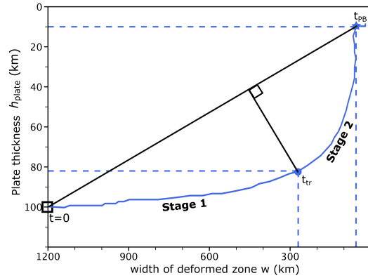
Figure B1. Definition of the transition time t_{tr} illustrated using the reference experiment, Simulation ref-1 (rheology D - d_{LT-HT} - Y_{500} MPa). The transition time t_{tr} is determined as the time at which the distance between the co-evolution of the deformed-zone width w and the plate thickness h_{plate} (blue line), and the straight line between the end-member states at t = 0 and t = t_{PB} (black line) is maximum.
