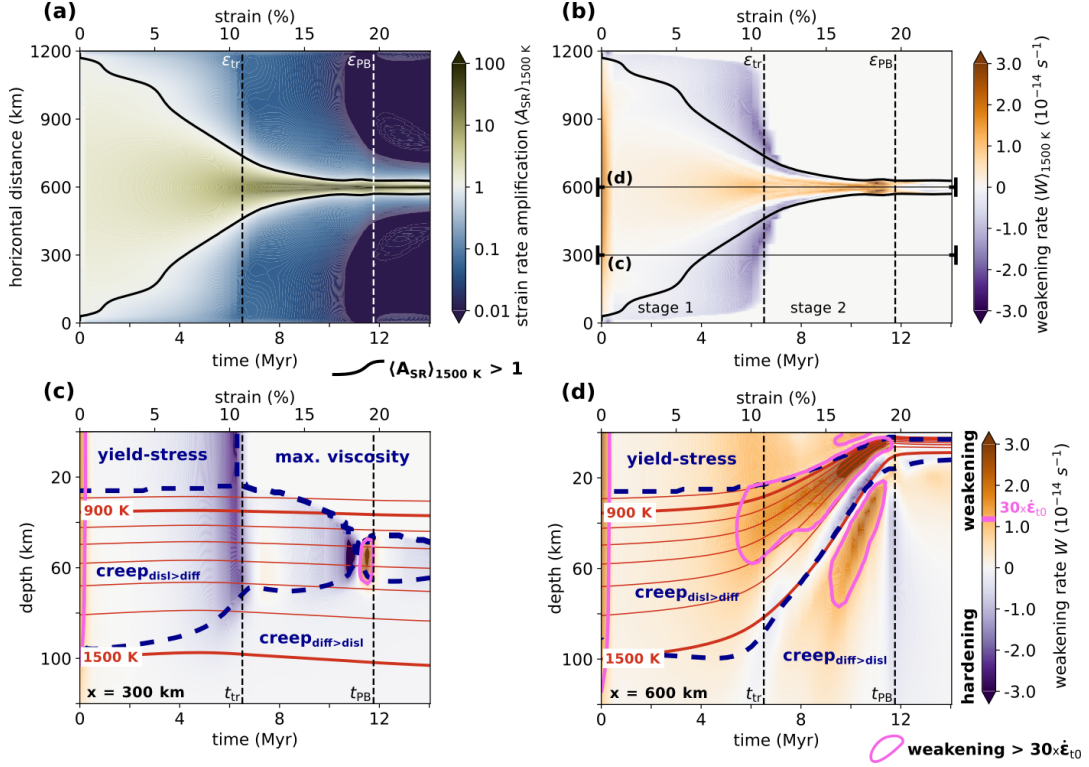
Figure 4. Localization of lithospheric deformation and weakening in Simulation D - d_{LT-HT} - Y_{500\text{ MPa}} (ref-1, Table 3). (a) Time-distance evolution of strain-rate amplification \langle A_{SR} \rangle_{1500\text{ K}}(x, t) , calculated as the vertically-averaged ratio relative to the initial uniform strain rate in the plate (here \dot{\epsilon}_{t_0} \sim 3.73 \cdot 10^{-16}\text{ s}^{-1} , see Sect. 3.1). The thick black line features the isocontour 1 of this ratio. (b) Time-distance plot of the geometric mean of the vertically-averaged weakening rate \langle W \rangle_{1500\text{ K}}(x, t) (Sect. 3.2). Orange shades indicate where weakening ( W > 0 ) affects more than 60 % of lithospheric thickness, with plotted values representing the geometric mean at a given x and time t over all depths z where W(x, z, t) > 0 . On the other hand, purple-blue shades indicate where weakening affects less than 40 % of lithospheric thickness, plotting the vertical geometric mean for depths where W \leq 0 (hardening or neutral). Areas where weakening affects between 40 % and 60 % of the lithospheric thickness are left white. (c), (d) Depth-time evolution of the weakening rate W at x = 300\text{ km} (c) and 600\text{ km} (d). The pink outline highlights zones of high weakening where \frac{W}{\dot{\epsilon}_{t_0}} > 30 , and the red lines indicate isotherms from 800 to 1500 K. Regions with different dominant deformation mechanisms are delineated by dashed dark-blue contours. In all panels, vertical dashed lines indicate the transition time, t_{tr} and the plate boundary time, t_{PB} .
