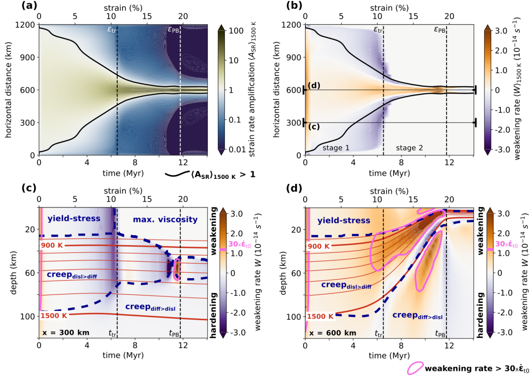
Figure 4. Localization of lithospheric deformation and weakening in Simulation D – d_{LT-HT} - Y_{500\text{ MPa}} (ref-I, Table 3). (a) Time-distance evolution of strain-rate amplification \langle A_{SR} \rangle_{1500\text{ K}}(x, t) , calculated as the vertically-averaged ratio relative to the initial uniform strain rate in the plate (here \dot{\epsilon}_{t_0} \sim 3.73 \cdot 10^{-16} \text{ s}^{-1} , see Sect. 3.1). The thick black line features the isocontour 1 of this ratio. (b) Time-distance plot of the geometric mean of the vertically-averaged weakening rate \langle W \rangle_{1500\text{ K}}(x, t) (Sect. 3.2). Orange shades indicate where weakening ( W > 0 ) affects more than 60 % of lithospheric thickness, with plotted values representing the geometric mean at a given x and time t over all z where W(x, z, t) > 0 . On the other hand, purple-blue shades indicate where weakening affects less than 40 % of lithospheric thickness, plotting the vertical geometric mean -\langle W_{SR} \rangle_{1500\text{ K}}(x, t) for depths where W \leq 0 (hardening or neutral). Areas where weakening affects between 40 % and 60 % of the lithospheric thickness are left white. (c), (d) Depth-time evolution of the weakening rate W at x = 300\text{ km} (c) and 600\text{ km} (d). The pink outline highlights zones of high weakening rate where \frac{W}{\dot{\epsilon}_{t_0}} > 30 , and the red lines indicate isotherms from 800 to 1500 K. Regions with different dominant deformation mechanisms are delineated by dashed dark-blue contours. In all panels, vertical dashed lines indicate the transition time, t_{tr} and the plate boundary time, t_{PB} .
