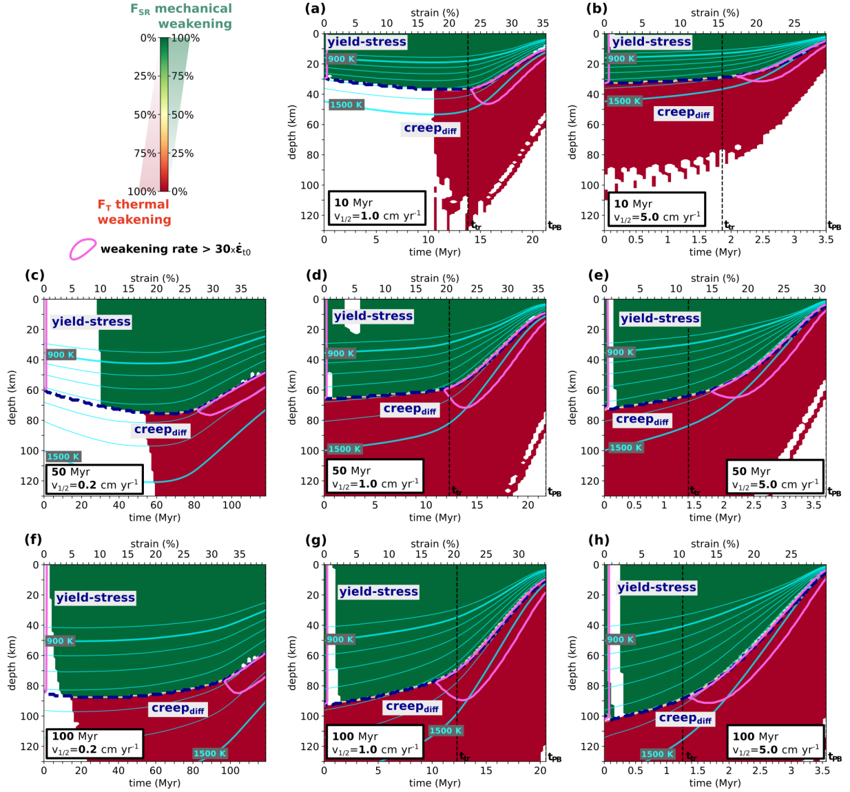
Figure D2. (This figure uses the same representation as Fig. 8) in the main text.) Depth-time evolution of the relative contributions to weakening F_T and F_{SR} calculated at box center x = 600 km with rheology D - Y_{500} MPa. Panels are organized with rows corresponding to varying initial plate age and columns corresponding to varying half-extension velocity v_{1/2} . The central panel represents the reference setup (initial plate age of 50 Myr, half-extension rate of 1 cm yr -1 ). In each panel, time varies from 0 to t_{PB} (which differs between panels), and the transition time t_{tr} is indicated by a vertical dashed line, except in (c-f) where localization is not achieved and the results are shown for the total duration of the simulation. The diagnostics are calculated only in regions in weakening ( W > 0 ), with hardening or stable regions ( W \leq 0 ) shown in white. The colorscale is capped between 0 and 1. Zones of intense weakening, where the weakening rate normalized by the initial strain rate in the plate \frac{W}{\dot{\epsilon}_{t_0}} exceeds 30, are highlighted in pink. Boundaries between dominant deformation mechanisms are marked by dashed dark-blue lines as in Fig. 4, and isotherms from 800 to 1500 K are displayed in light blue.
