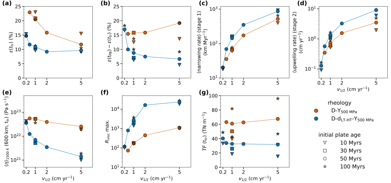
Figure 10. Diagnostics as a function of half-extension velocity v_{1/2} for two different rheologies, D-Y_{500 \text{ MPa}} (red) and D-d_{LT-HT}-Y_{500 \text{ MPa}} (blue). Symbols represent initial plate ages ranging from 10 to 100 Myr. (a) Strain \varepsilon(t_{tr}) , used as a proxy for the duration of Stage 1. (b) Difference \varepsilon(t_{PB}) - \varepsilon(t_{tr}) used as a proxy for duration of Stage 2. (c) Mean narrowing rate during Stage 1. (d) Mean upwelling rate during Stage 2. (e) Effective viscosity vertically-averaged over the lithosphere thickness ( T < 1500 \text{ K} ) at t_{tr} and at horizontal position x = 600 \text{ km} . (f) Maximum lateral viscosity contrast ( R_{\text{visc max.}} ) during the two stages, with a maximum reached around t_{PB} . (g) Tectonic force TF(t_{tr}) at time t_{tr} . In all panels, solid lines connect the markers corresponding to the initial lithospheric age of 50 Myr, used as a reference age.
