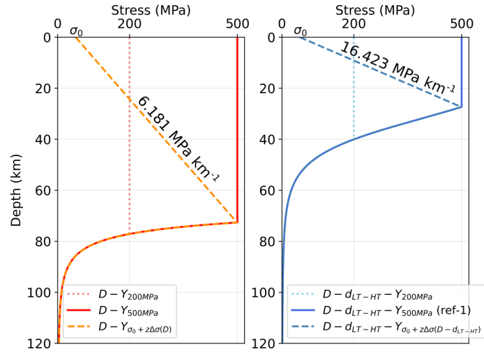
Figure E1. Strength profile computed for a uniform strain rate \dot{\epsilon} = 3 \cdot 10^{-15} \text{ s}^{-1} and a temperature profile corresponding to a 50 Myrs-old Myr-old lithosphere. The red and dark blue curves are respectively: diffusion, and diffusion plus low- and high-temperature dislocation creep rheologies, in combination with a depth-dependent yield stress (dashed lines), or with a constant yield stress of 200 or 500 MPa (orange dotted and light blue solid lines, respectively). The yield-creep transition for the depth-dependent yield stress is reached at a maximum strength of 500 MPa, which is consistent to the yield-creep transition depth for constant yield stress of 500 MPa combinations.
