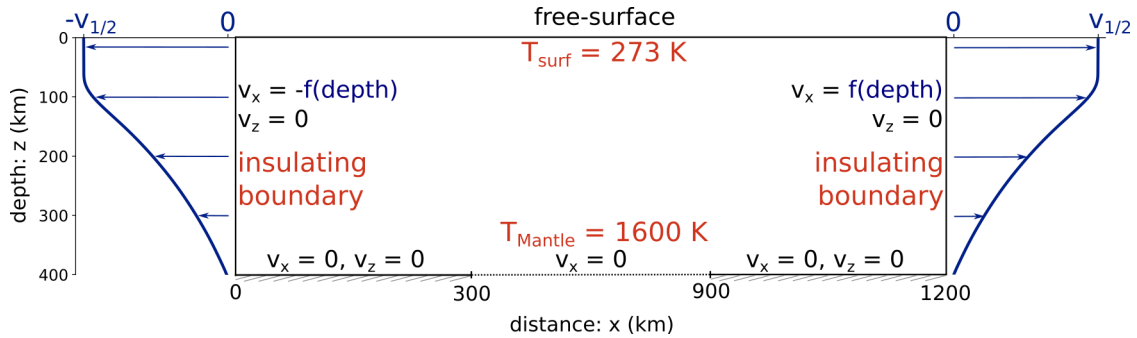
Figure 1. Simulation set-up in the 400 \times 1200 \text{ km} 2-D domain. Mechanical boundary conditions (in blue) are a free-surface top, and depth-dependent horizontal flow on the vertical sides, where v_{1/2} is the plate half extension rate. The bottom boundary is no-slip and closed ( v_z = v_x = 0 ), except over a 600 km-wide open segment between x = 300 and 900 \text{ km} where purely vertical flow is allowed ( v_x = 0 ). Thermal boundary conditions (in red) are constant temperatures at top (273 K) and bottom (1600 K), and insulating vertical boundaries.
