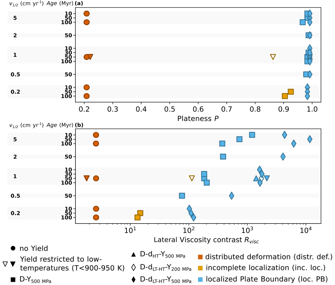
Figure A1. (a) Plateness P and (b) lateral viscosity contrast R_{visc} obtained after 40 % strain for various extension rates, initial plate age, and rheologies. The end-member simulations (distributed deformation, localized plate boundary) are depicted in red and blue, respectively. The incomplete localization case in yellow is intermediate between the two end-members.
