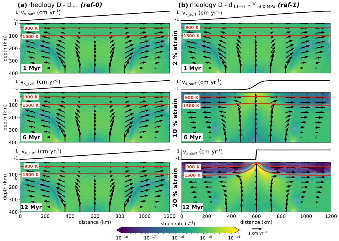
Figure 3. Evolution of the strain rate field (second invariant) during two end-member simulations, shown after 1 Myr, 6 Myr and 12 Myr of extension: (a) Simulation D - d_{\text{HT}} ( ref-0 ), with diffusion creep and high-temperature dislocation creep, Table 3 characterized by uniform and diffuse lithospheric thinning; (b) Simulation D - d_{\text{LT-HT}} - Y_{500 \text{ MPa}} ( ref-1 ), combining diffusion creep, low- and high-temperature dislocation creep, and a yield-stress set to 500 MPa, which successfully localizes plate deformation. For each snapshot, the horizontal velocity at the surface is plotted above. Velocity field is depicted by black arrows, and the 900 K and 1500 K isotherms are indicated in red.
