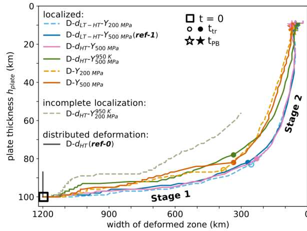
Figure 6. Co-evolution of the minimum plate thickness h_{\text{plate}}(t) as a function of the width w(t) of the most -deformed zone (see Sect. 3.2) for experiments with the same initial age (50 Myr) and extension velocity v_{1/2} = 1 \text{ cm yr}^{-1} for 8 different rheological combinations. The transition time t_{\text{tr}} between Stages 1 and 2 is indicated by a circle symbol and the localization time t_{\text{PB}} by a star symbol. Open and filled symbols correspond to rheologies with a yield stress set to 200 and 500 MPa, respectively. The square represent the initial time.
