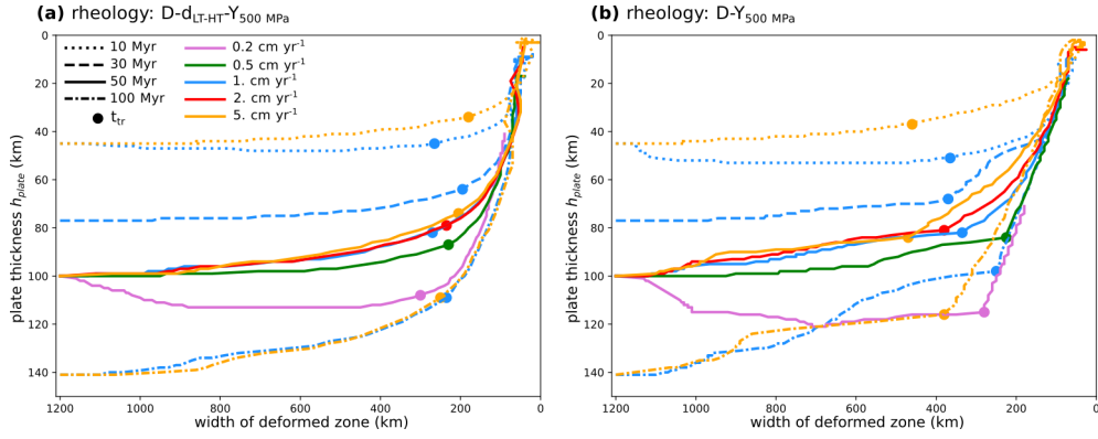
Figure D3. Co-evolution of the minimum plate thickness h_{plate}(t) as a function of the width of the most deformed zone w(t) for two rheological combinations: (a) D - d_{LT-HT} - Y_{500} MPa. (b) D - Y_{500} MPa. Curves are shown for varying initial plate age (indicated by line-styles and half-spreading velocity (indicated by colors). The transition times t_{tr} between Stages 1 and 2 are marked by dots.
