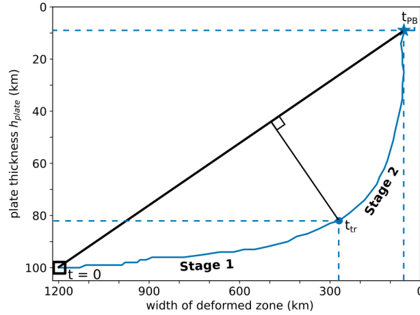
Figure B1. Definition of the transition time t_{tr} illustrated using the reference experiment, Simulation ref-1 (rheology D - d_{LT-HT} - Y_{500 \text{ MPa}} ). The transition time t_{tr} is determined as the time at which the distance between the co-evolution of the deformed-zone width w and the plate thickness h_{plate} (blue line), and the straight line between the end-member states at t = 0 and t = t_{PB} (black line) is maximum.
