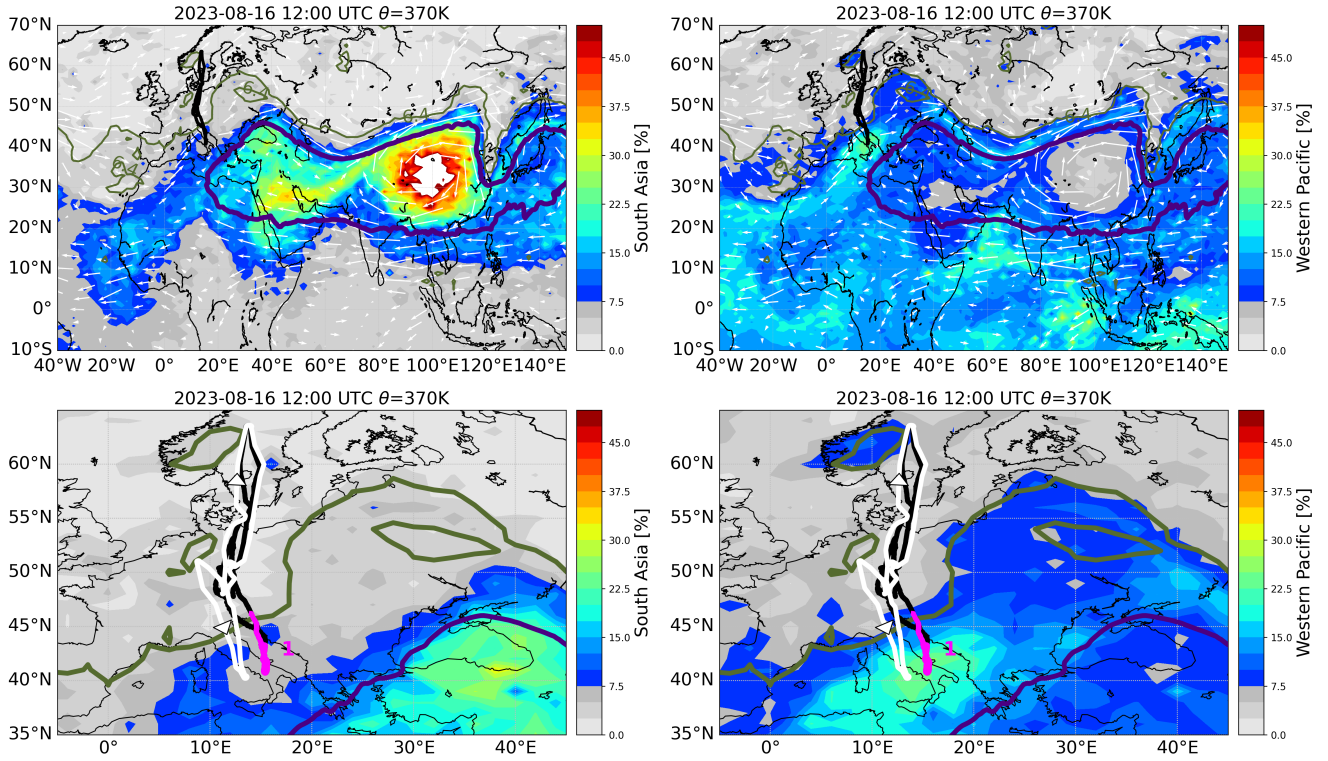
Figure 10. Research-As in Fig. 6 but for research flight F06 on 16 August 2023 conducted from Oberpfaffenhofen, Germany, to the Mediterranean area-region (in direction of South towards southern Italy) reach-. Research flight F06 reaches the outer edge of the ASMA (South Asia surface-origin tracer at 370 K, 12:00 UTC, left), which is dominated by air from the western Pacific (Western Pacific surface-origin tracer at 370 K, 12:00 UTC, right). The surface-origin tracer distributions are based on a CLaMS simulation driven by ERA5. The calculated synoptic HALO flight track position at 12:00 UTC is indicated by the black line. To indicate the edge of the ASMA boundary (indigo line); the boundary of the ASMA is calculated using the Montgomery streamfunction. An optimised background value gives the ASMA boundary (given by MSF = 356.6 \times 10^3 \text{ m}^2 \text{ s}^{-2} ) for 6-16 August 2023 at 12:00 at UTC and 370 K using ERA5 reanalysis data based on the method by Kachula et al. (2025). The climatological isentropic transport barrier ( PV = 6.4 \text{ PVU} ) derived by Kunz et al. (2015) for the Northern Hemisphere at 370 K during summer indicates the barrier between the tropical tropopause layer and the extra-tropical lower stratosphere. Time interval 1 shown in Fig. 11 is marked in magenta (olive line bottom). Further, horizontal winds are indicated by white arrows.
