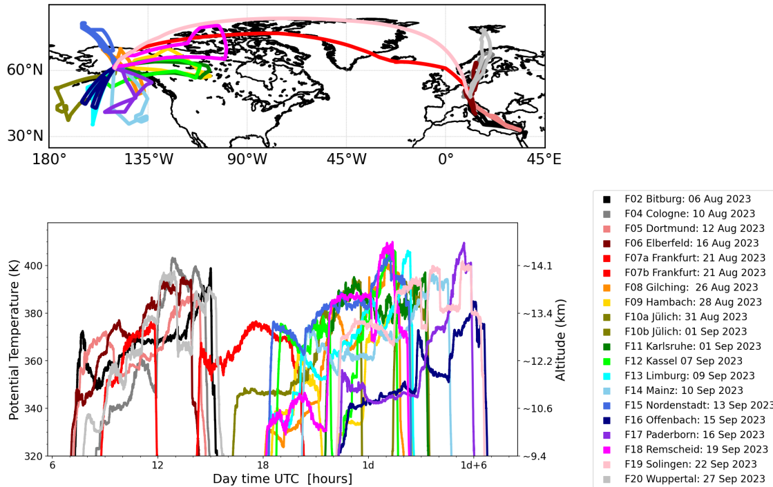
Figure 1. Regional map showing all HALO aircraft flight tracks over the Northern Hemisphere during the PHILEAS campaign 2023 (top). A total of 20-18 scientific flights (F02–F20; excluding the Electromagnetic Compatibility (EMC) flight electromagnetic compatibility and turbulence calibration flights F01 and F03, and counting the double flights F07a/b and F10a/b as one flight each) were conducted between 6 August and 27 September 2023, departing from Oberpfaffenhofen (Germany), and Anchorage (Alaska), USA. Maximum altitudes up to \sim 14.5 km ( \sim 410 K potential temperature) were reached. Research flights from Alaska were conducted during local daytime, which corresponds to nighttime in Coordinated Universal Time (UTC), and therefore often crossed the International Date Line, marked as 1 day (Alaska local time = UTC - 7 h, Germany local time = UTC + 2 h considering summer time).
