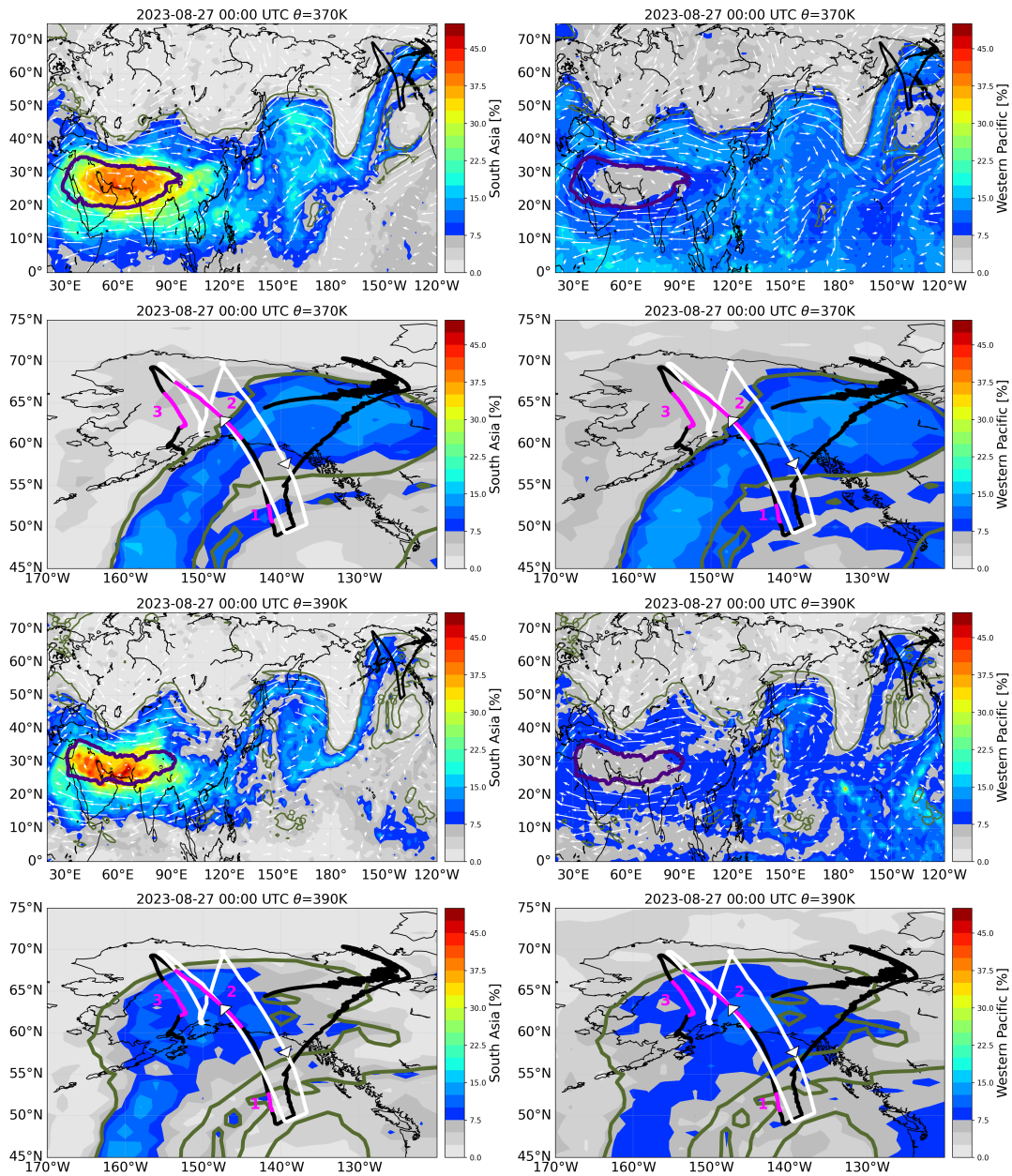
Figure 13. Research-As in Fig. 6 but for research flight F08 on 26-27 August 2023 conducted from Anchorage probing a filament over Alaska separated from the ASMA (South Asia surface-origin tracer at 370 K and at 390 K, 00:00 UTC, left), which is mixed with air from the western Pacific (Western Pacific surface-origin tracer at 370 K and 390 K, 00:00 UTC, right). The surface-origin tracer distributions are based on a CLAMS simulation driven by ERA5. The calculated synoptic HALO flight track position at 27 August 2023 is shown at 00:00 UTC is indicated by the (black line). To indicate the edge of the ASMA boundaries (indigo line), the boundary of the ASMA is calculated using the Montgomery streamfunction. An optimised background value gives the ASMA boundary (are given by MSF = 357.0 \times 10^3 \text{ m}^2\text{s}^{-2} at 370 K and MSF = 367.6 \times 10^3 \text{ m}^2\text{s}^{-2} at 390 K) for 27 August 2023 at 00:00 using ERA5 reanalysis data based on the method by Kaechula et al. (2025). The climatological 00. Climatological isentropic transport barrier-barriers ( PV = 6.4 \text{ PVU} olive line) at 370 K and 8.6 \text{ PVU} ( PV = 6.4 \text{ PVU} ) and at 390 K) derived by Kunz et al. (2015) for the Northern Hemisphere during summer (JJA) are given. Time intervals 1–3 shown in Fig. 15 are marked in magenta in the barrier-between-zoomed plots. The zoomed plots
