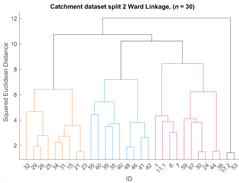
Figure C4. Ward linkage cluster dendrogram of the catchment dataset, split 2.
