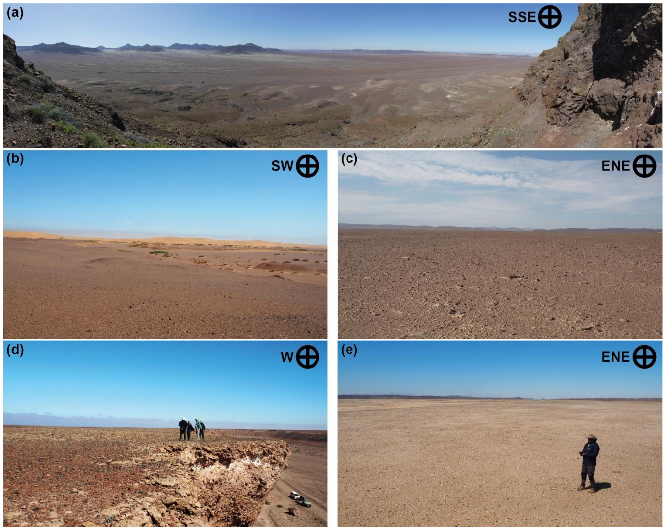
120 Figure 1: Examples of different alluvial fans investigated in this study. From north to south: (a) Sechomib, IDs #11.1 and 11.2, 18.4 °S, 12.6 °E; (b) Kharu-Gaiseb, #30, 19.9 °S, 13.2 °E; (c) Koigab, #44, 20.5 °S, 13.4 °E; (d) Messum (upper), #62.2, 21.4 °S, 14.0 °E; and (e) Horingbaai, #63, 21.6 °S, 13.9 °E. Note the different surface generations evident in (a), dunes of the Skeleton Coast Erg overlying alluvial deposits and blocking overland flow in (b), desert pavement, often on \text{CaSO}_4 -encrusted surfaces in (c) to (e). Images were taken during field campaigns in 2022 and 2023.
