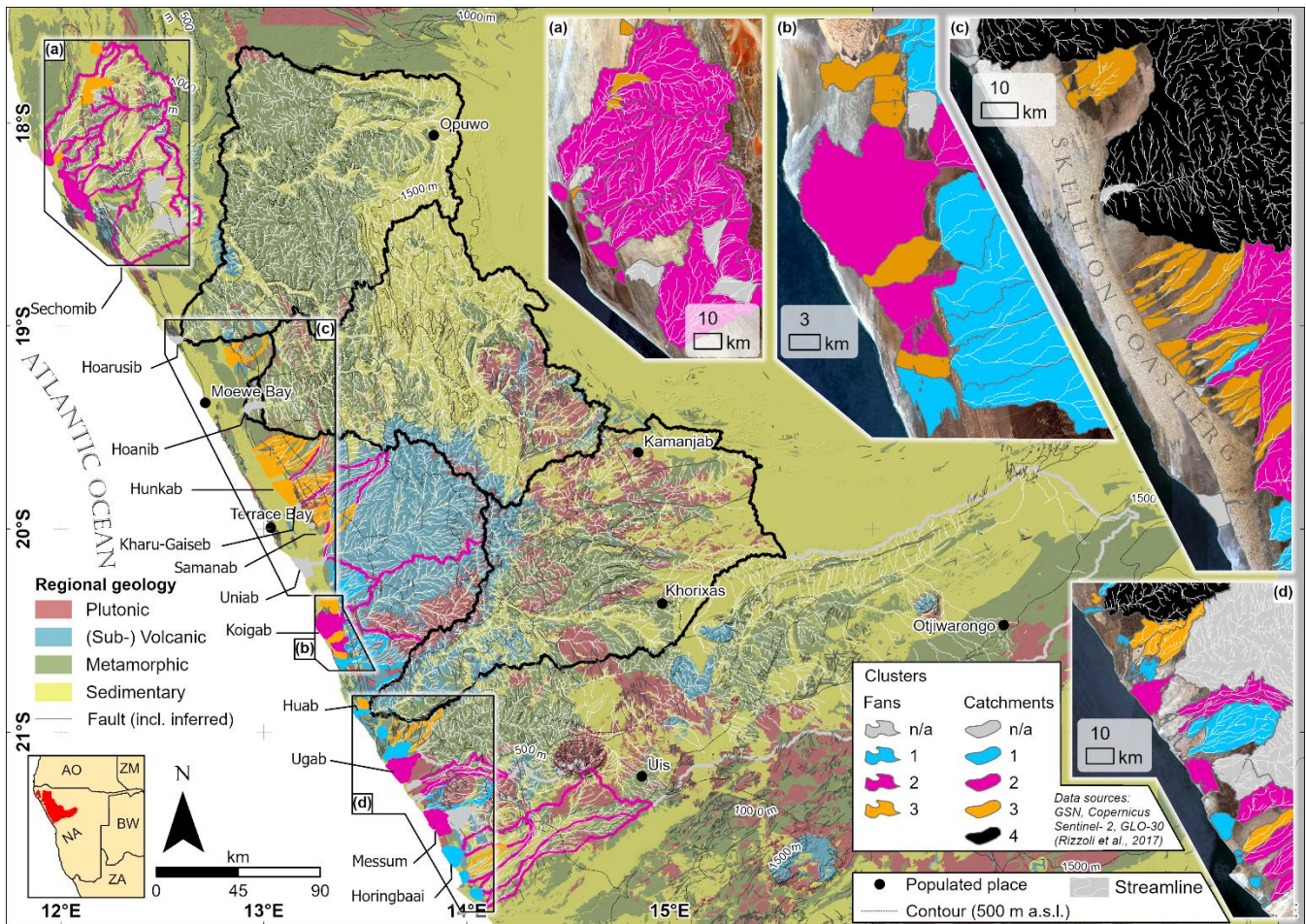
540 Figure 6: Geological map of the Skeleton Coast of Namibia, including catchment and alluvial landform clusters.
