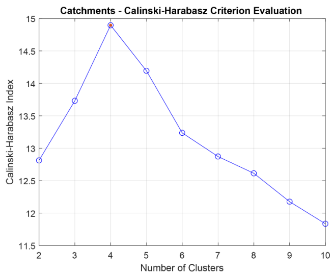
1035 Figure C2. Cluster number determination for the catchment dataset based on the Caliński and Harabasz criterion (Caliński and Harabasz, 1974).
