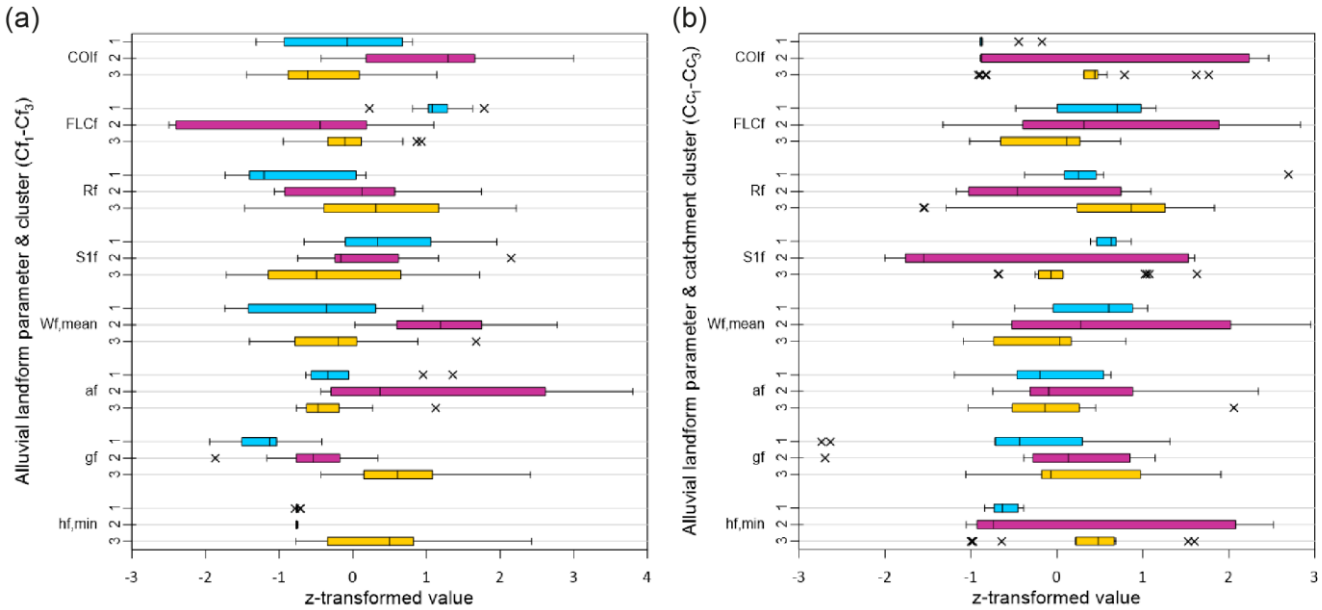
575 Figure 7: Boxplots showing the median, 25 and 75 % quartiles, 1.5x interquartile range and outliers (indicated by crosses) for the alluvial landform variables used to cluster the fan dataset, applied to the alluvial landform (a) and catchment clusters (b). Z-transformed data as used for the clustering is shown to account for the different scales of the individual variables.
