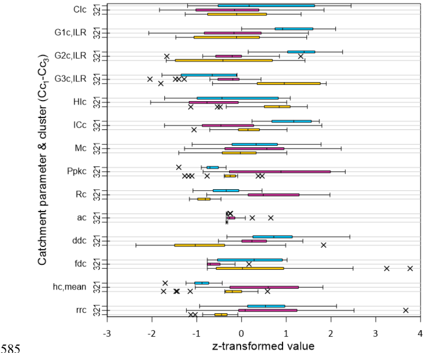
585 Figure 8: Boxplots showing the median, 25 and 75 % quartiles, 1.5× interquartile range and outliers (indicated by crosses) for the catchment variables used to cluster the catchment dataset. Z-transformed data as used for the clustering is shown to account for the different scales of the individual variables.
