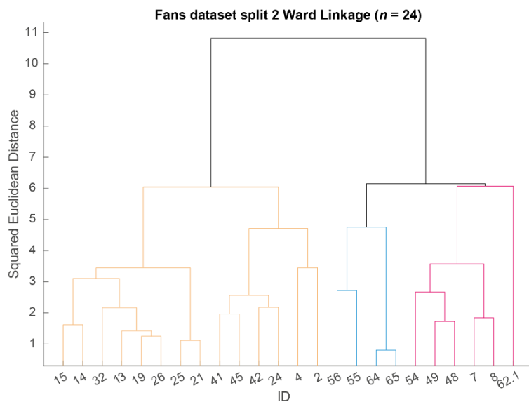
1055 Figure C8. Ward linkage cluster dendrogram of the fan dataset, split 2.
