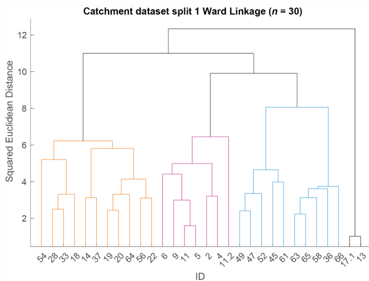
Figure C3. Ward linkage cluster dendrogram of the catchment dataset, split 1.
