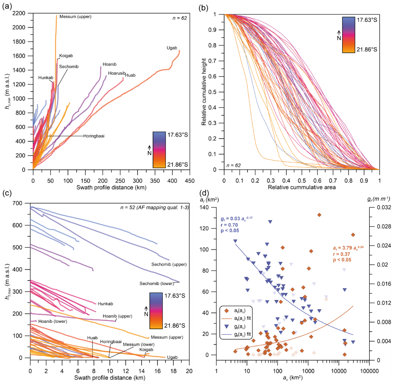
480 Figure 3: Catchment swath profiles (a), hypsometric curves (b), alluvial deposit swath profiles (c), and power-law relationships between fan and catchment morphometrics (d). Data in (a) and (b) is shown for n = 62 catchments, with nested subcatchments not being shown for clarity. In panel (c), all alluvial deposits featuring a mapping quality that deemed sufficient (quality class <4 , cf. Table B1) are shown ( n = 52 ). Likewise, data from this fraction of the population is used to derive the power correlations as shown in (d), with the remaining data shown as greyed-out symbols.
