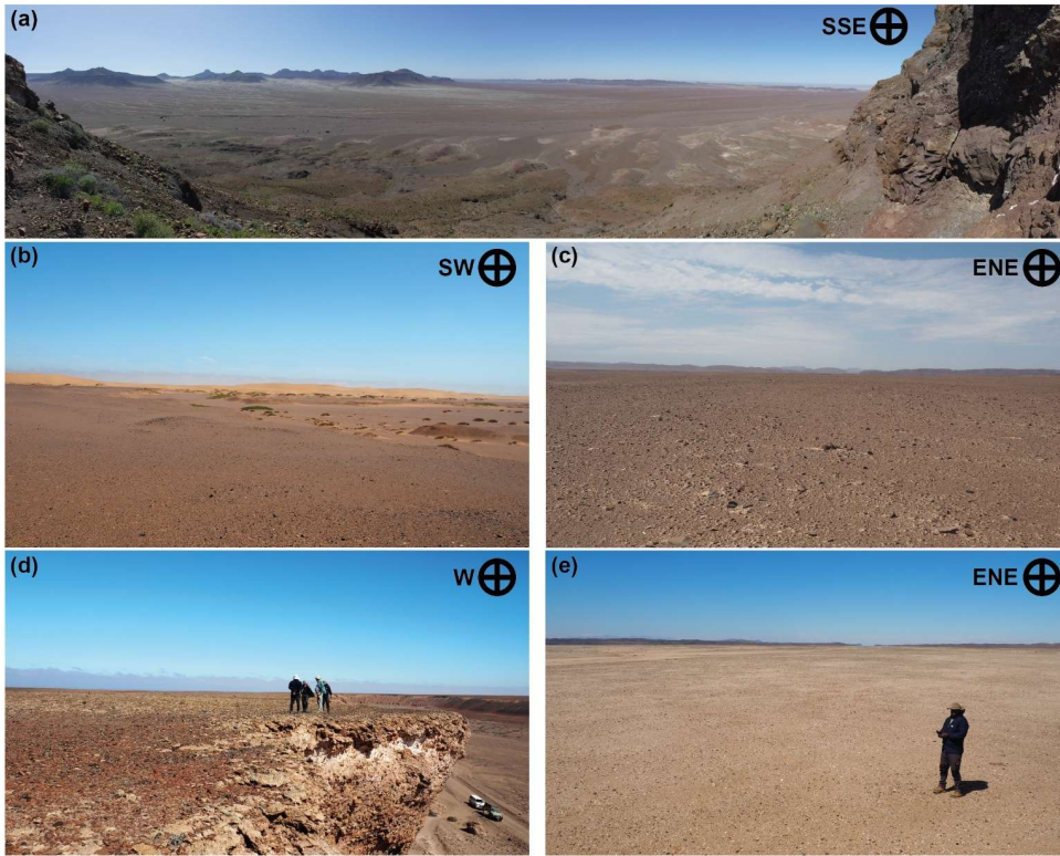
Figure 1: Examples of different alluvial fans investigated in this study. From north to south: (a) Sechomib, IDs #11.1 and 11.2, 18.4 °S, 12.6 °E; (b) Kharu-Gaiseb, #30, 19.9 °S, 13.2 °E; (c) Koigab, #44, 20.5 °S, 13.4 °E; (d) Messum (upper), #62.2, 21.4 °S, 14.0 °E; and (e) Horingbaai, #63, 21.6 °S, 13.9 °E. Note the different surface generations evident in (a), dunes of the Skeleton Coast Erg overlying alluvial deposits and blocking overland flow in (b), desert pavement, often on CaSO 4 -encrusted surfaces in (c) to (e). Images were taken during field campaigns in 2022 and 2023.
