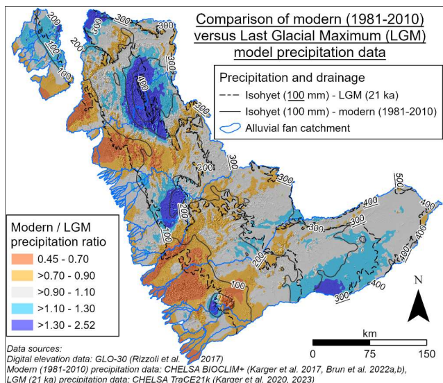
Figure C11. Comparison of modern (1981-2010) versus LGM model precipitation data (Brun et al., 2022b, a; Karger et al., 2017; Karger et al., 2023, 2020). Ratios calculated from the datasets indicate drier modern conditions close to the present-day coastline, while more humid present-day conditions are predominantly located in elevated and hinterland areas. The coast-parallel precipitation gradient appears in both model datasets. The bundle of 21 ka 100 mm isohvet contours was thinned out by removing isolated and closed contours related to topographical noise.
