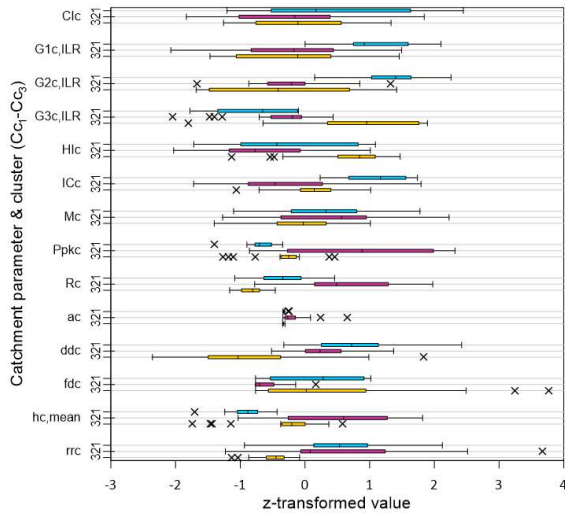
Figure 8: Boxplots showing the median, 25 and 75 % quartiles, 1.5x interquartile range and outliers (indicated by crosses) for the catchment variables used to cluster the catchment dataset. Z-transformed data as used for the clustering is shown to account for the different scales of the individual variables.
