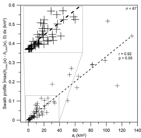
Figure C10. Relationship between fan area a_f and the area between the minimum and maximum (90th percentile) swath profile line. The area represents the integral of the positive part of the elevation difference (calculated in Matlab ver. R2024a using the trapz function on densely gridded, interpolated data points). A similar linear relationship is obtained for the fan dataset ( n = 52 , r = 0.91 ).
