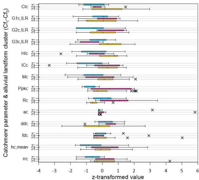
Figure C9. Boxplots showing the median, 25 and 75% quartiles, 1.5x interquartile range and outliers (indicated by crosses) for the catchment variables, grouped by fan variable clustering. Z-transformed data as used for the clustering is shown to account for the different scales of the individual variables.
