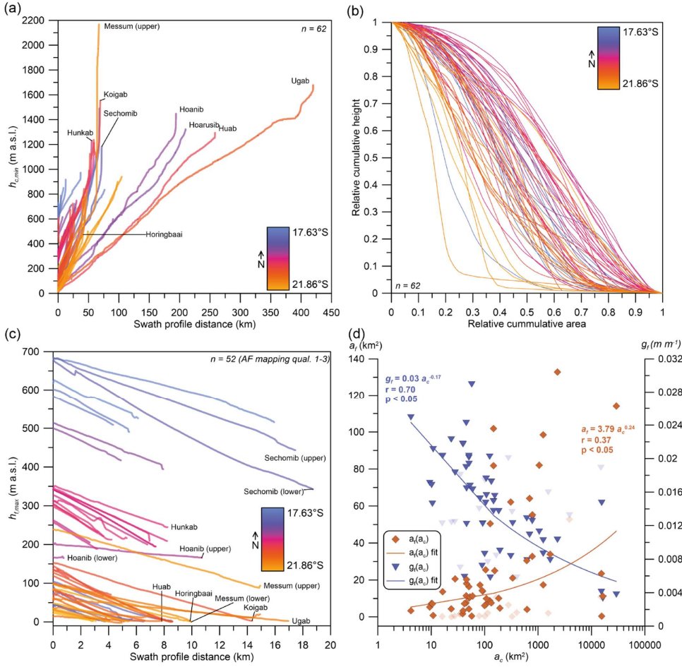
Figure 3: Catchment swath profiles (a), hypsometric curves (b), alluvial deposit swath profiles (c), and power-law relationships between fan and catchment morphometrics (d). Data in (a) and (b) is shown for n = 62 catchments, with nested subcatchments not being removed shown for clarity. In panel (c), all alluvial deposits featuring a mapping quality that deemed sufficient (quality class < 4 , cf. Table B1) are shown ( n = 52 ). Likewise, data from this fraction of the population is used to derive the power correlations as shown in (d), with the remaining data shown as greyed-out symbols.
