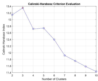
Figure C6. Cluster number determination for the fan dataset based on the Caliński and Harabasz criterion (Caliński and Harabasz, 1974).
