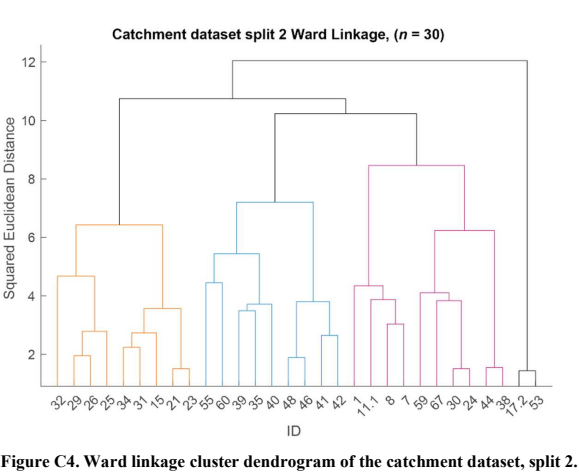
Figure C4. Ward linkage cluster dendrogram of the catchment dataset, split 2.
