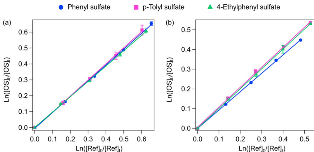
Figure 1. Loss of aromatic OSs and BA during the process of the liquid-phase •OH oxidation at (a) pH 3 and (b) pH 8.
