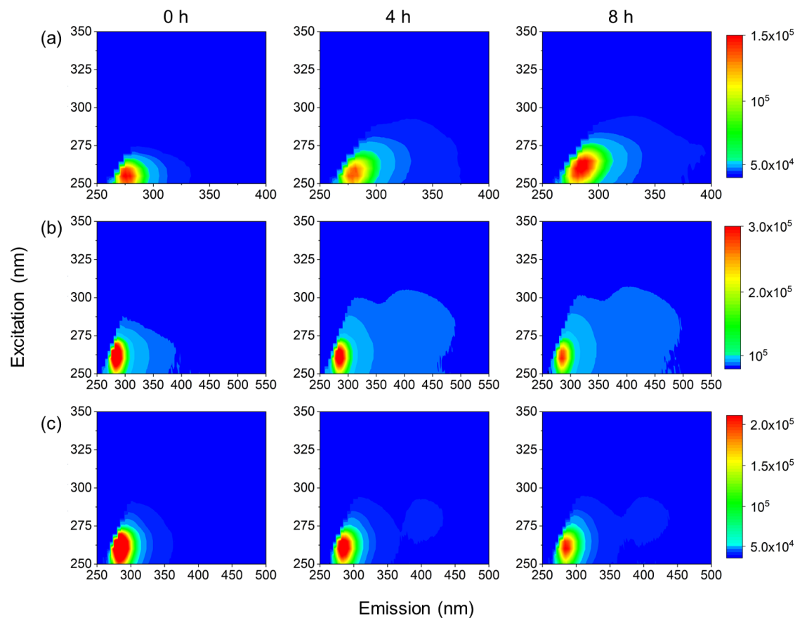
Figure 4. Time profile of excitation–emission matrix (EEM) fluorescence spectra during the processes of (a) phenyl sulfate, (b) p-tolyl sulfate and (c) 4-ethylphenyl sulfate reacting with \bullet OH at pH 3.
