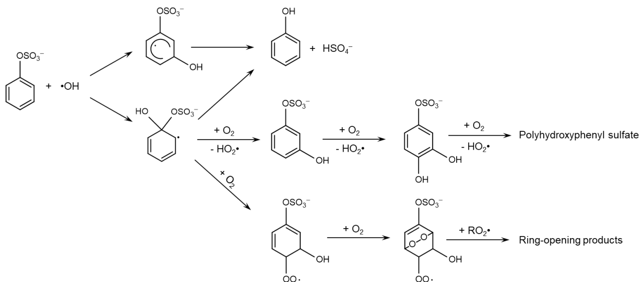
Figure 2. Scheme for the mechanism of phenyl sulfate reacting with \bullet OH .
