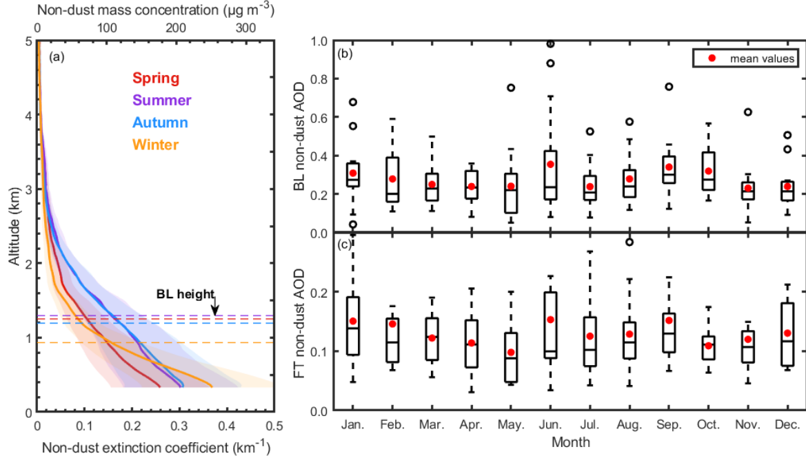
Figure 8. (a) Profiles of seasonally averaged non-dust extinction coefficient \alpha_{nd} and mass concentration M_{nd} . The seasonally averaged boundary layer heights are presented by dashed lines. Box plots of the monthly mean (b) BL and (c) FT non-dust AOD for each month from 2010 to 2024. The parameters for box plots are the same as in Figure 2.
