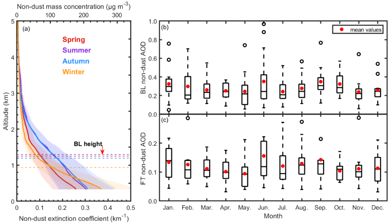
Figure 7. (a) Profiles of seasonally averaged non-dust extinction coefficient \alpha_{\text{nd}} and mass concentration M_{\text{nd}} . The seasonally averaged boundary layer heights are presented by dashed lines. Box plots of the monthly mean (b) BL and (c) FT non-dust AOD for each month from 2010 to 2024. The parameters for box plots are the same as in Figure 2.
