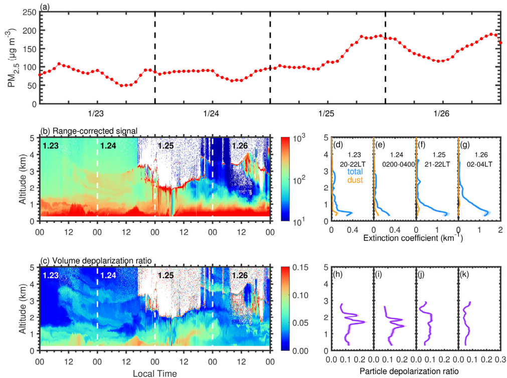
Figure 10. (a) \text{PM}_{2.5} concentration in Wuhan on 23-26 January 2019, and time-altitude contour plots of (b) range-corrected signal and (c) volume depolarization ratio measured by polarization lidar over Wuhan during the same period. Selected typical profiles of (d-g) extinction coefficient and (h-k) particle depolarization ratio.
