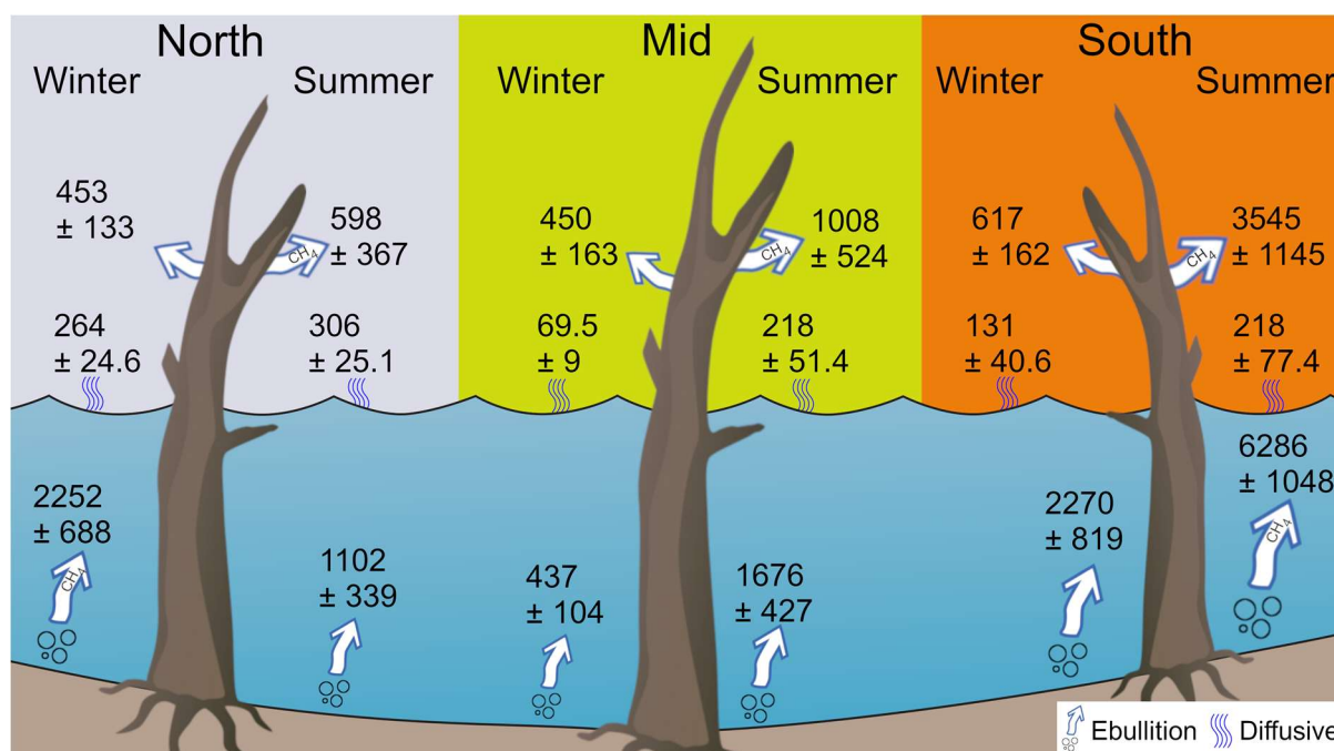
Figure 9: Conceptual figure summarising the three pathways for CH 4 ( \mu\text{mol m}^{-2} \text{ d}^{-1} and \pm is SE) between the three sites and for the winter and summer campaigns. Graphics: Tracey Saxby, Integration and Application Network ( ian.umces.edu/media-library )
