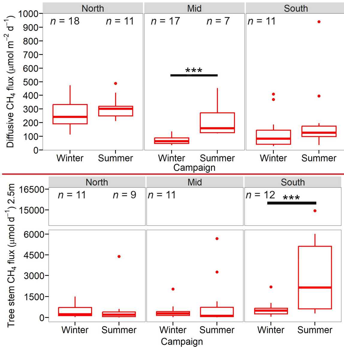
Figure 6: Diffusive CH 4 flux (top) and tree stem CH 4 fluxes (μmol tree -1 d -1 ) (bottom) Tree stem fluxes were scaled to 2.5 m stem height. Significant differences are shown with the solid horizontal line.
