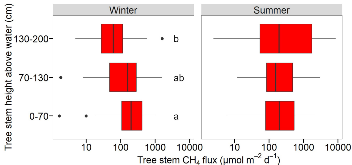
Figure 7: Tree stem CH 4 (in μmol m -2 d -1 ) fluxes measured at three heights (cm) above water level at Hinze Dam ( n = bottom to top: winter: 31, 32 and 31, summer: 22, 27 and 29). Data includes all three study sites during both winter and summer campaigns. Letters indicate significant differences. Note: log scale for x-axis.
