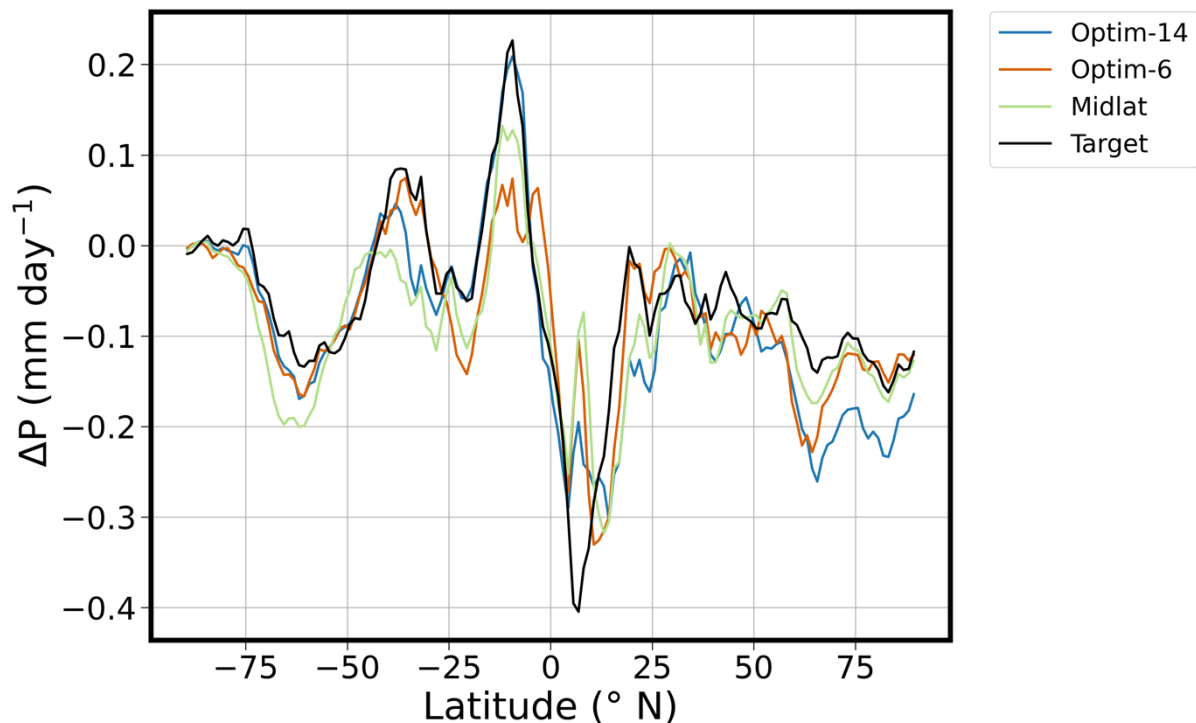
440 Figure 15: Zonal mean 2040s precipitation anomaly ( \Delta P ) for the Optim-14, Optim-6 and Midlat, with respect to the target restoring the 2014-2033 SSP2-4.5 mean.
