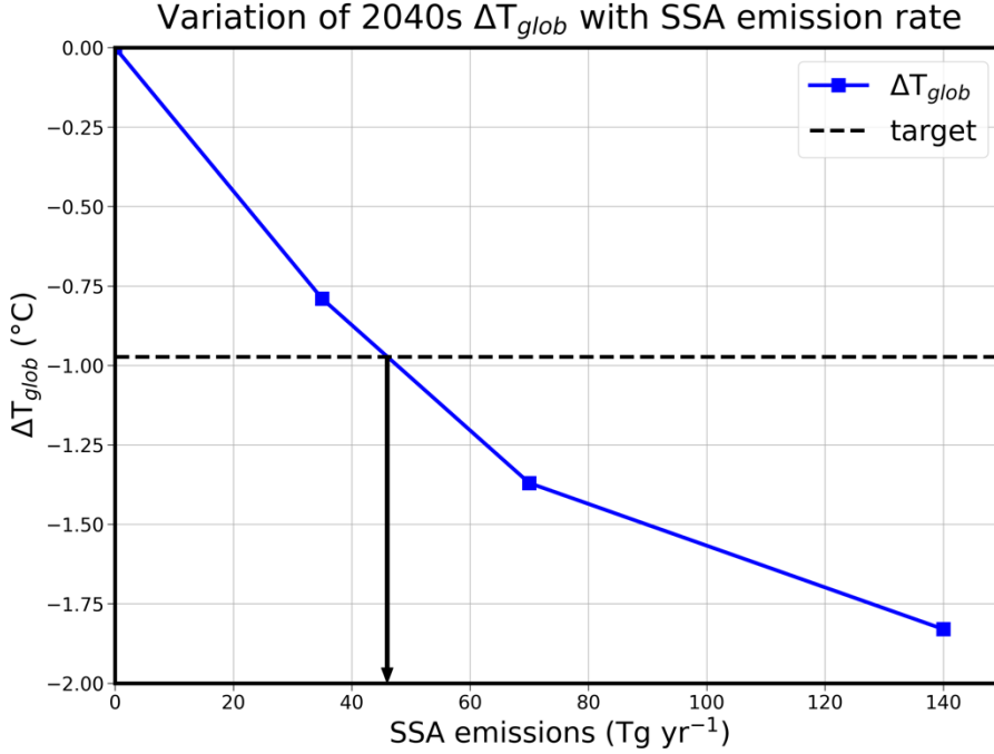
Figure 8: Variation of 2040s global mean surface air temperature anomaly ( \Delta T_{glob} ) with sea salt aerosol (SSA) emission rate for a 35, 70 and 140 \text{Tg yr}^{-1} MCB deployment with the SSA shared equally across the 14 regions. The dashed line indicates the target cooling required to restore the 2014-33 \Delta T_{glob} . Linear interpolation suggests a 46 \text{Tg yr}^{-1} is required to achieve this cooling target.
