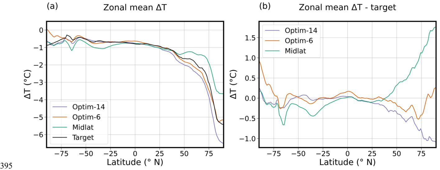
Figure 13: (a) Zonal mean 2040s surface air temperature anomaly ( \Delta T ) for Optim-14, Optim-6, and Midlat, compared to the SSP2-4.5 2014-2033 minus 2040s target. Panel (b) shows the zonal mean \Delta T difference between the deployments and the target.
