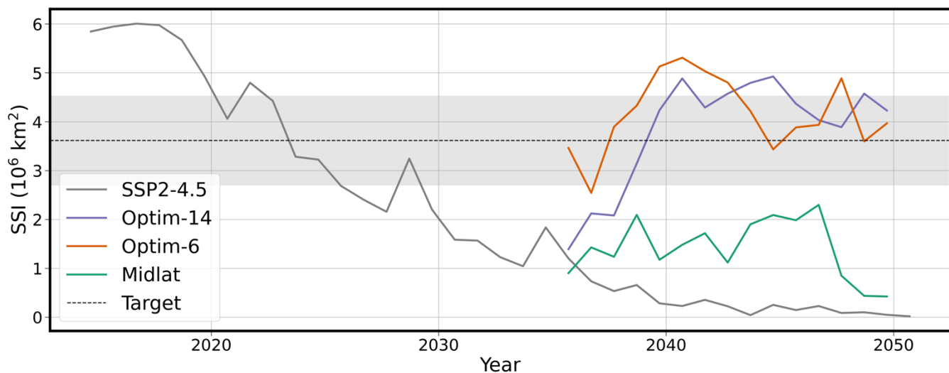
405 Figure 14: Arctic September sea ice extent (SSI) responses of Optim-14, Optim-6 and Midlat, compared to SSP2-4.5. The dashed line shows the 2014-2033 target and the shading shows the target range used in the methodology to produce Optim-14 and Optim-6, as described in Section 4.
