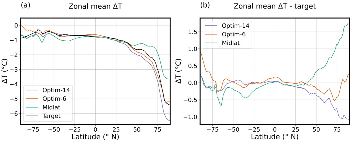
400 Figure 13: (a) Zonal mean 2040s surface air temperature anomaly ( \Delta T ) for Optim-14, Optim-6, and Midlat, compared to the SSP2-4.5 2014-2033 minus 2040s target. Panel (b) shows the zonal mean \Delta T difference between the deployments and the target.
