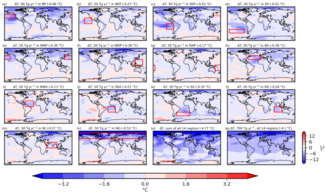
205 Figure 3: Panels (a-n) show the 2040s surface air temperature anomaly ( \Delta T ) from the 50 Tg yr -1 patch simulations relative to SSP2-4.5. Panel (o) shows the sum of the 14 responses in panels (a-n), for comparison with the 700 Tg yr -1 simulation in panel (p). The 2040s global mean surface air temperature anomaly ( \Delta T_{\text{glob}} ) is annotated in brackets above each panel. The horizontal colour bar corresponds to panels a-n, and the vertical colour bar next to panel (p) corresponds to panels (o) and (p).
