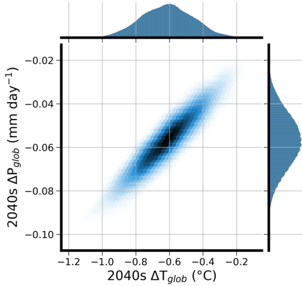
320 Figure 9: A heatmap of the 2040s global mean precipitation anomaly ( \Delta P_{\text{glob}} ) against 2040s global mean surface air temperature anomaly ( \Delta T_{\text{glob}} ) combination space for a 1,144,066 sample of possible 50 Tg yr -1 MCB combinations, estimated using equation 2, assuming additivity and linearity with the patch simulations.
