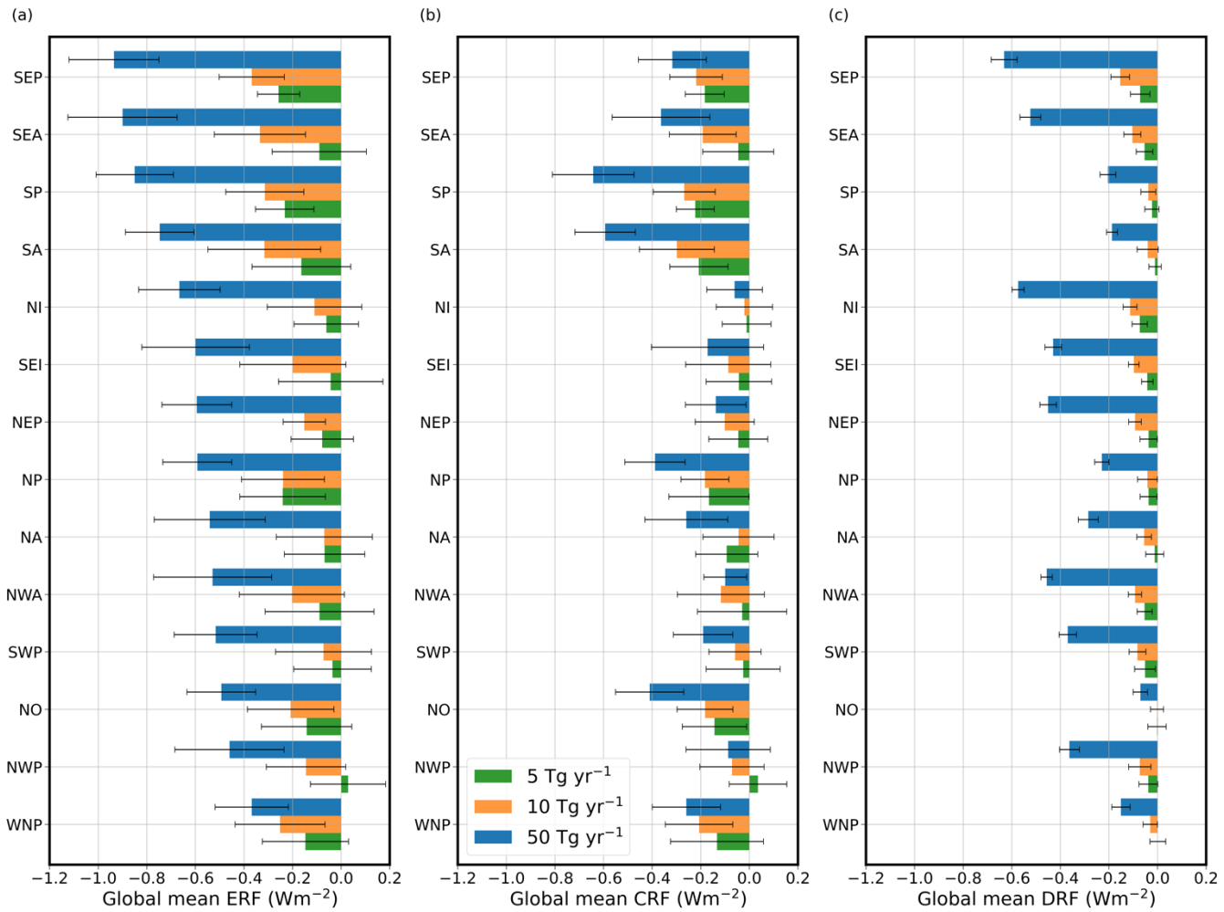
175 Figure 2: Panel (a) shows the 10-year mean ERF from the MCB simulations for the different regions shown in Fig. 1 and defined in Table 1. The cloudy and clear-sky components of the ERF are shown in panels (b) and (c) respectively. Error bars show one standard deviation of the annual mean ERF responses.
