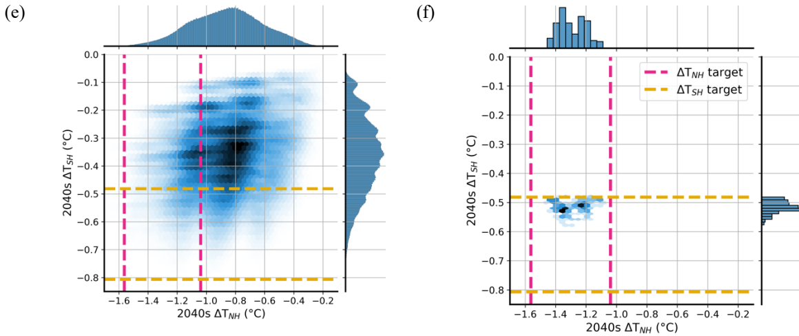
Figure 10: Heatmaps showing the narrowing down of the combinations based on climate response targets defined in Table 2. Panels (a), (c) and (e) show the heatmaps for the 1,144,066 combinations. Panels (b), (d) and (f) show the heatmaps for the remaining 172 combinations that satisfy all 6 climate response targets. Dashed lines show the upper and lower bounds of a given target.
