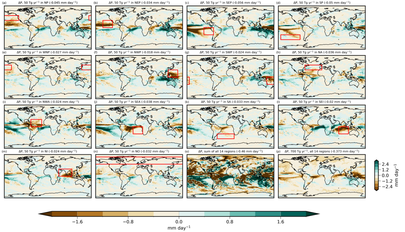
195 Figure 4: Same as in Fig. 3, but for 2040s precipitation anomaly ( \Delta P ). The 2040s global mean precipitation anomaly ( \Delta P_{\text{glob}} ) is annotated in brackets above each panel.
