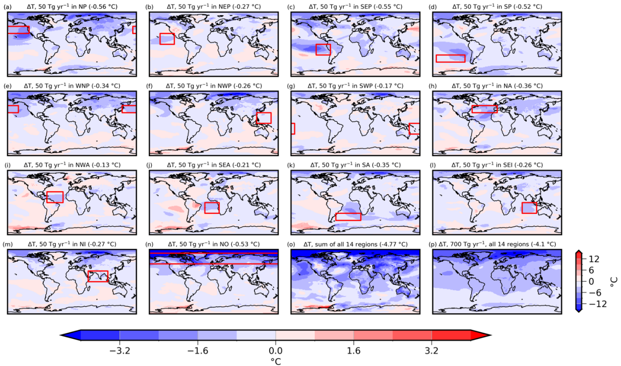
Figure 3: Panels (a-n) show the 2040s surface air temperature anomaly ( \Delta T ) from the 50 Tg yr -1 patch simulations relative to SSP2-4.5. Panel (o) shows the sum of the 14 responses in panels (a-n), for comparison with the 700 Tg yr -1 simulation in panel (p). The 2040s global mean surface air temperature anomaly ( \Delta T_{\text{glob}} ) is annotated in brackets above each panel. The horizontal colour bar corresponds to panels a-n, and the vertical colour bar next to panel (p) corresponds to panels (o) and (p).
