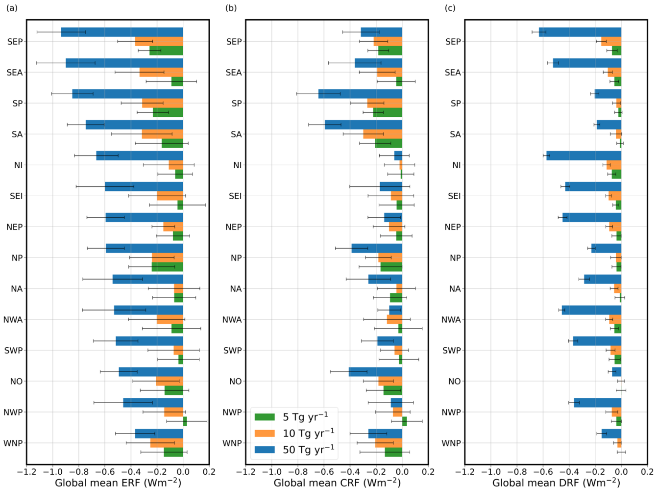
165 Figure 2: Panel (a) shows the 10-year mean ERF from the MCB simulations for the different regions shown in Fig. 1 and defined in Table 1. The cloudy and clear-sky components of the ERF are shown in panels (b) and (c) respectively. Error bars show one standard deviation of the annual mean ERF responses.
