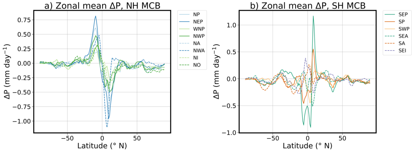
Figure 5: Zonal mean 2040s precipitation anomaly ( \Delta P ) for the 50 Tg \text{yr}^{-1} patch simulations in (a) the Northern Hemisphere (NH) and (b) the Southern Hemisphere (SH) relative to SSP2-4.5.
