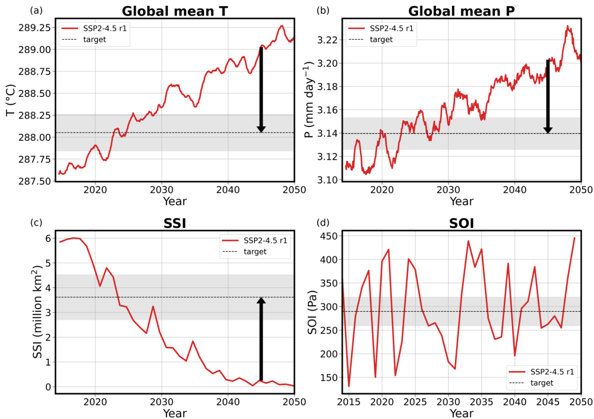
Figure 7: (a) global mean surface air temperature, (b) global mean precipitation, (c) Arctic September sea ice extent (SSI) and (d) Southern Oscillation Index (SOI) targets, aiming to restore the 2040s climate to the 2014–2033 mean state (dashed line). The shading shows the target range and the black arrows show the magnitude for a conceptual target restoration. This is omitted in panel (d) due to the small magnitude of the SOI target.
