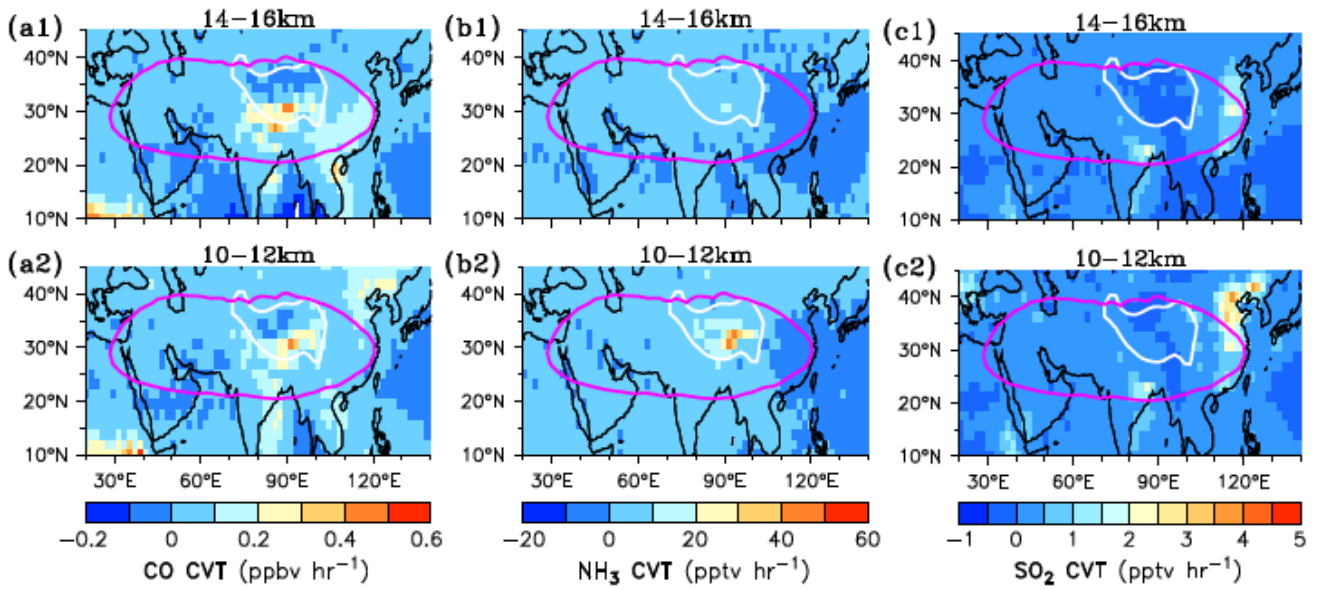
Figure 5. EMAC simulated mean deep convective transport tendency (CVT) of CO ( a1 and a2 ), \text{NH}_3 ( b1 and b2 ) and \text{SO}_2 ( c1 and c2 ) at selected altitudes, i.e., 14-16 km ( a1 , b1 and c1 ) and 10-12 km ( a2 , b2 and c2 ) above sea level, averaged for JJA over the years 2010-2020. Purple lines show the 16.64 km geopotential height contour at 100 hPa, highlighting the main ASMA area (see Figure S1). White lines represent the 3 km terrain height contour, highlighting the Tibetan Plateau.
