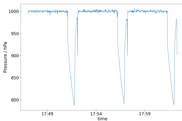
Figure A5. Example of detected inlet icing. At the start of the expansion and the end of refill a steep drop can be seen in the pressure. The plot also shows This is due to the characteristic reduced pressure inside the chamber resulting from the iced inlet . The pressure drop at results from the end of equilibrating gas once the refill valve switches . The plot shows operation 198, runs 10 to 12 from the CORONA campaign.
