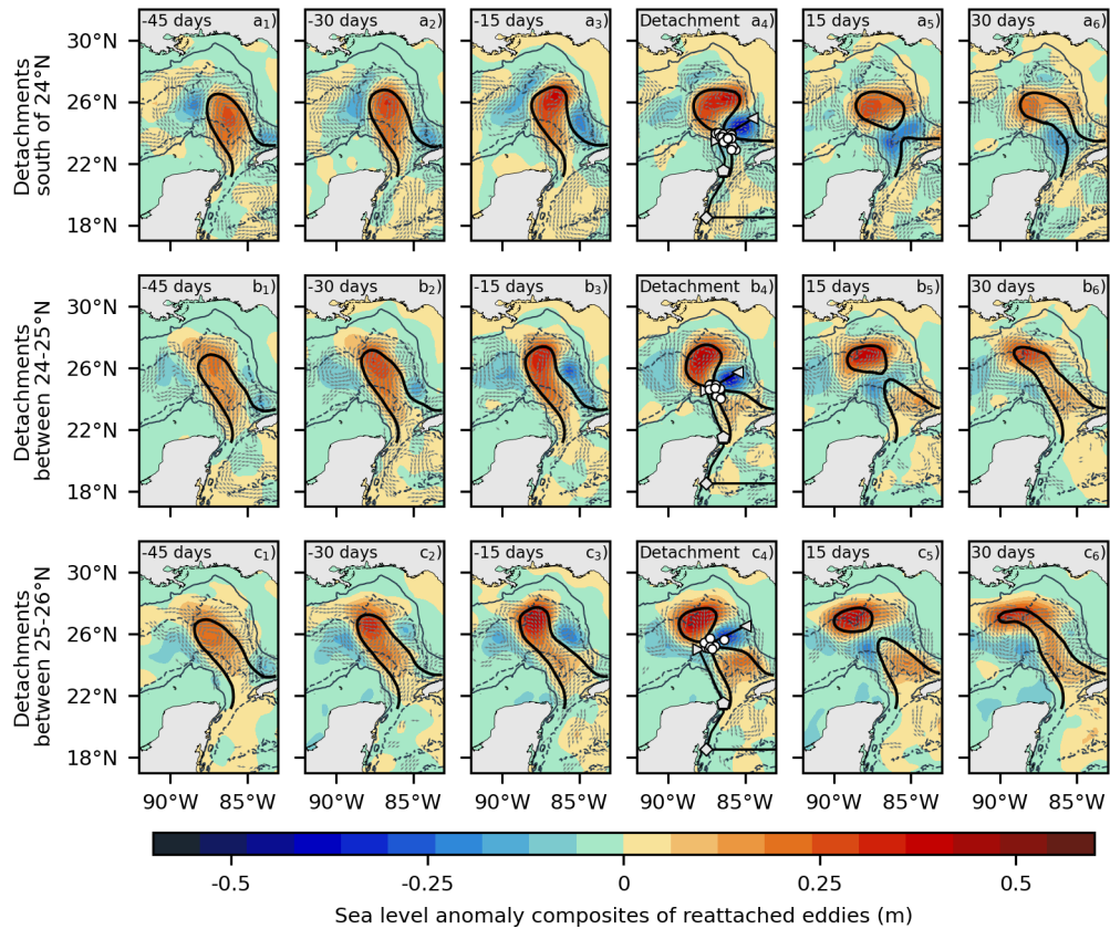
Figure 5. SLA composites related to detachments occurring south of 24^{\circ}\text{N} (first row), between 24 and 25^{\circ}\text{N} , and between 25 and 26^{\circ}\text{N} , that turn into reattachment events. Continued tick black contours represent the LC composite (ADT 17 cm). White circles in the fourth column represent the LC outermost position after detachment events used for the composites. The gray arrows depict the direction of surface geostrophic currents with speeds stronger than 0.1 \text{ m s}^{-1} . The light gray contours refer to the 200 m (continuous) and 2500 m (dashed) depths.
