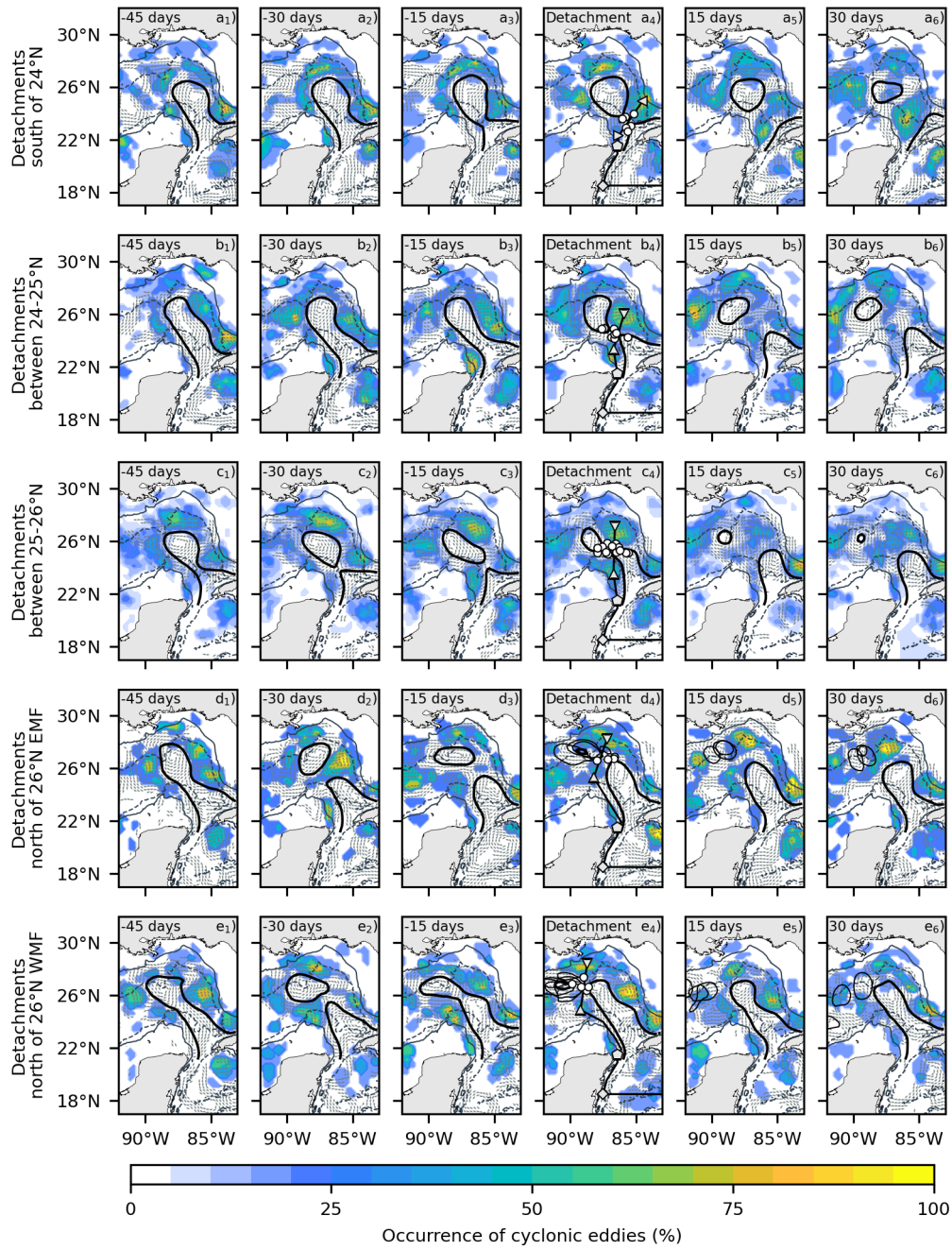
Figure A3. Occurrence of cyclonic eddies during the evolution of LCEs separation events south of 24^{\circ}\text{N} (first row), between 24\text{--}25^{\circ}\text{N} (second row), between 25\text{--}26^{\circ}\text{N} (third row), as well as separations north of 26^{\circ}\text{N} occurring east (EMF; fourth row) and west (WMF; fifth row) of the Mississippi Fan. Thick contours represent the composite LC and detached LCEs. Thin contours in the last three columns of separations north of 26^{\circ}\text{N} represent the LCEs for each detachment case in the region. The gray arrows depict the direction of surface geostrophic currents with speeds stronger than 0.1\text{ m s}^{-1} . White circles represent the LC outermost position after detachment events used for the composites. The light gray contours refer to the 200 m (continuous) and 2500 m (dashed) depths.
