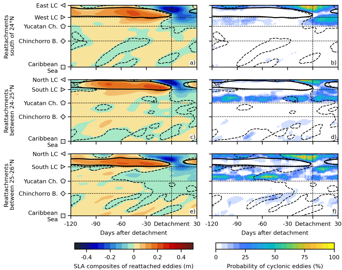
Figure 8. Hovmöller composites of SLA (first column) and the occurrence of cyclonic eddies from the AVISO Atlas (second column) during reattachments occurring south of 24^{\circ}\text{N} (first row), between 24\text{-}25^{\circ}\text{N} (second row), and between 25\text{-}26^{\circ}\text{N} (third row). Thick continuous-black contours represent the composite LC (ADT 17-cm). Thick segmented-black contours depict cyclonic anomalies. Thin vertical segmented lines exhibit the detachment of LCEs. Horizontal segmented lines indicate the location of the Chinchorro Bank, Yucatan Channel, and the southern region of the LC (western region of the LC in a).
