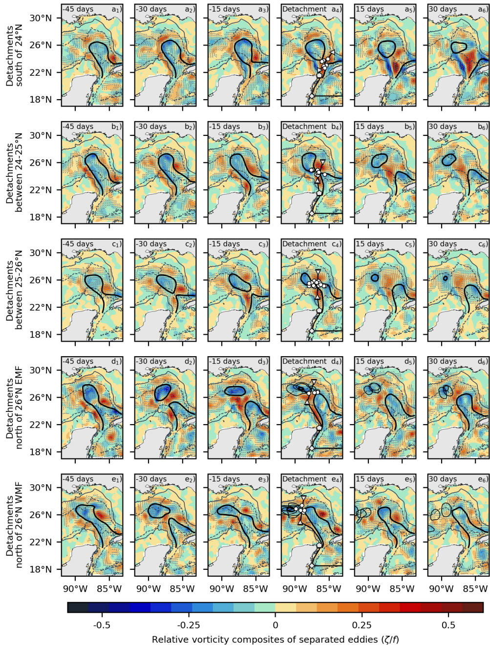
Figure A2. Time evolution of Rossby number during LCEs separation south of 24^{\circ}\text{N} (first row), between 24\text{--}25^{\circ}\text{N} (second row), between 25\text{--}26^{\circ}\text{N} (third row), as well as separations north of 26^{\circ}\text{N} occurring east (EMF; fourth row) and west (WMF; fifth row) of the Mississippi Fan. Thick contours represent the composite LC and detached LCEs. Thin contours in the last three columns of separations north of 26^{\circ}\text{N} represent the LCEs for each detachment case in the region. The gray arrows depict the direction of surface geostrophic currents with speeds stronger than 0.1 \text{ m s}^{-1} . White circles represent the LC outermost position after detachment events used for the composites. The light gray contours refer to the 200 m (continuous) and 2500 m (dashed) depths.
