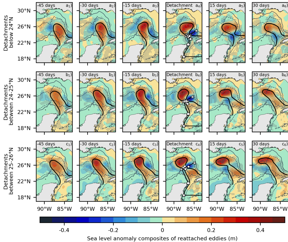
Figure 5. SLA composites related to detachments occurring south of 24^{\circ}\text{N} (first row), between 24 and 25^{\circ}\text{N} , and between 25 and 26^{\circ}\text{N} , that turn into reattachment events. Continued tick black contours represent the LC composite (ADT 17 cm). White circles in the fourth column represent the LC outermost position after detachment events used for the composites. The gray arrows depict the direction of surface geostrophic currents with speeds stronger than 0.1 \text{ m s}^{-1} . The light gray contours refer to the 200 m (continuous) and 2500 m (dashed) depths.
