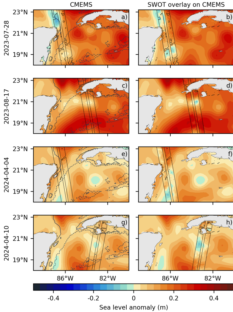
Figure 9. Examples of a comparison between SLA estimations between altimetric gridded maps from CMEMS (first column) and along-track observations from SWOT (second column). Both the first and second columns show CMEMS SLA fields and the spatial extent of the SWOT swath. In the second column, SWOT along-track measurements are additionally overlaid on the CMEMS fields within the swath. Each row refers to a different date. Continuous black contours show the 200-m depth contour, whereas dashed black contours show the 2500-m depth contour. The following describes the differences between the two products. First row: Cyclonic structure around 86^{\circ}\text{W} , 19^{\circ}\text{N} that is not visible in CMEMS but is visible in SWOT. Second row: Cyclonic structure around 84^{\circ}\text{W} , 21^{\circ}\text{N} that is not visible in CMEMS but is visible in SWOT. Third row: Cyclonic structure around 87^{\circ}\text{W} , 19^{\circ}\text{N} that is not visible in CMEMS but is visible in SWOT. Fourth row: Cyclonic structure around 83^{\circ}\text{W} , 21^{\circ}\text{N} with a weak signature in CMEMS but clearly visible in SWOT.
