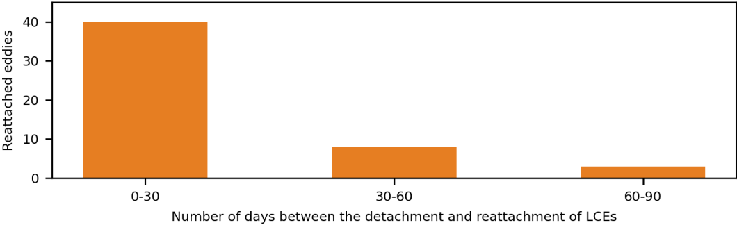
Figure A1. Histogram of the number of days it takes the LC to reattach the LCEs.
