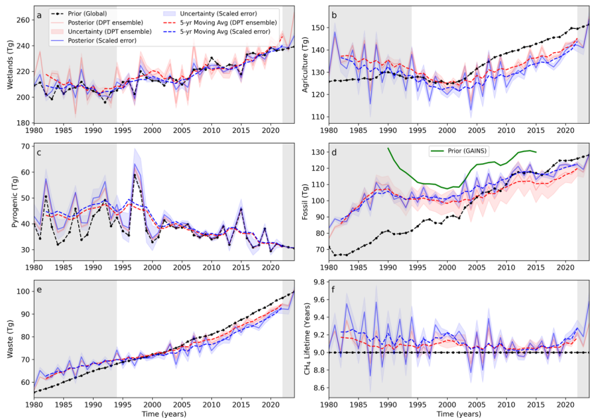
700 Figure 4: Prior (black, dotted) and posterior (coloured; raw, 5-year moving average and uncertainty) emission rates for 5 source categories (a-e) and lifetime (f) computed from (i) ensemble mean of the DPT optimised runs filtered from sensitivity tests ( <0.1 RMSE) and (ii) error-scaled inversion for source and lifetime. Posterior fossil emissions are also compared with GAINS (green) emissions alongside the priors (EDGAR). Grey shading indicates spin-up (1980-1993) and spin-down (2023- 2024) periods; the unshaded region (1994-2022) is the analysis period. The hemisphere-specific version of Figure 4 is available in Section 12 of the SI.
