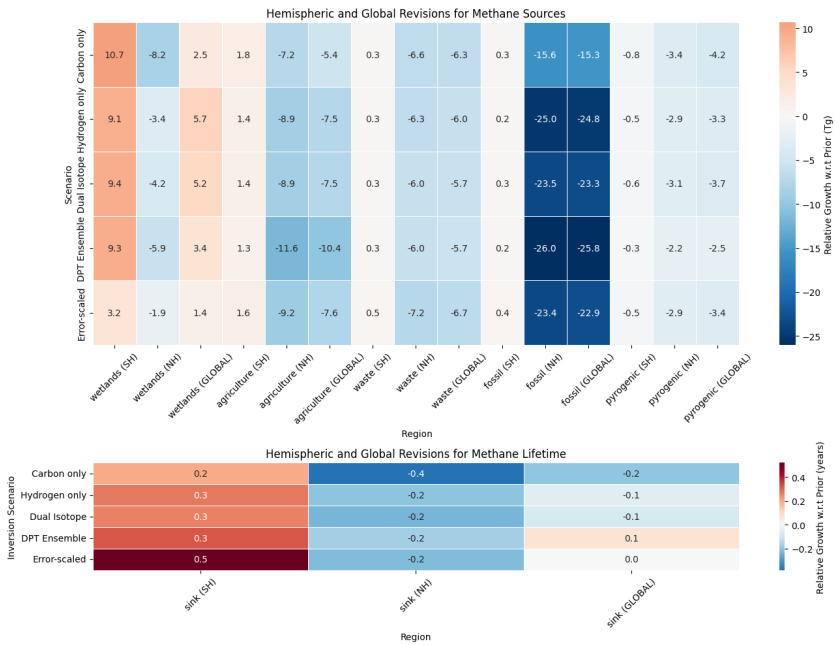
Fig. 5: Top panel: Hemispheric and global revisions w.r.t the priors ( Growth_{posterior} - Growth_{prior} ) of the growth in emissions by sector (wetlands, agriculture, waste, fossil, pyrogenic) in teragrams (Tg) per year. Growth is defined as the difference between the 1993-95 and 2021-23 averages. Bottom panel: hemispheric and global revisions for CH_4 lifetime (in years). The \chi(CH_4) -only inversion (using mole fraction data without isotopic constraints) is shown in SI section 12. This inversion produces unrealistic source partitioning because it lacks isotopic information to distinguish biogenic from thermogenic sources, confirming the necessity of isotopic constraints for robust source attribution.
