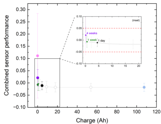
Figure 7. Plot of combined LOC-optode sensor package performance accuracy (relative to lab validation samples) as a function of charge required (by the LOC) to achieve the corrected accuracy. The colour-filled circle symbols are highlighted to illustrate five distinct points (i.e., uncorrected, 1 month, 1 week, 1 day, and 1 hour correction intervals). An inset provides a clearer zoomed-in region, and the dashed red lines indicate \pm 0.05 pH units for visual purposes.
