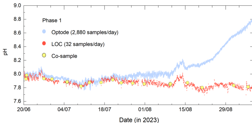
250 Figure 2. Overlay of optode (light blue filled circles), LOC (red filled circles), and discrete lab validated co-sample (yellow filled circles) pH data during phase 1.
