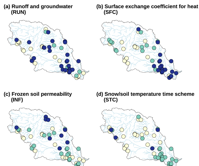
Figure 3 Changes in KGE at 50 HCDNs by the alternative parameterization scheme of (a) runoff and groundwater (RUN), (b) surface exchange coefficient for heat (SFC), (c) frozen soil permeability (INF) and (d) snow/soil temperature time scheme (STC). Subbasins are classified into three categories with different colors indicating No Improvement, Moderate Improvement, and Substantial Improvement.
