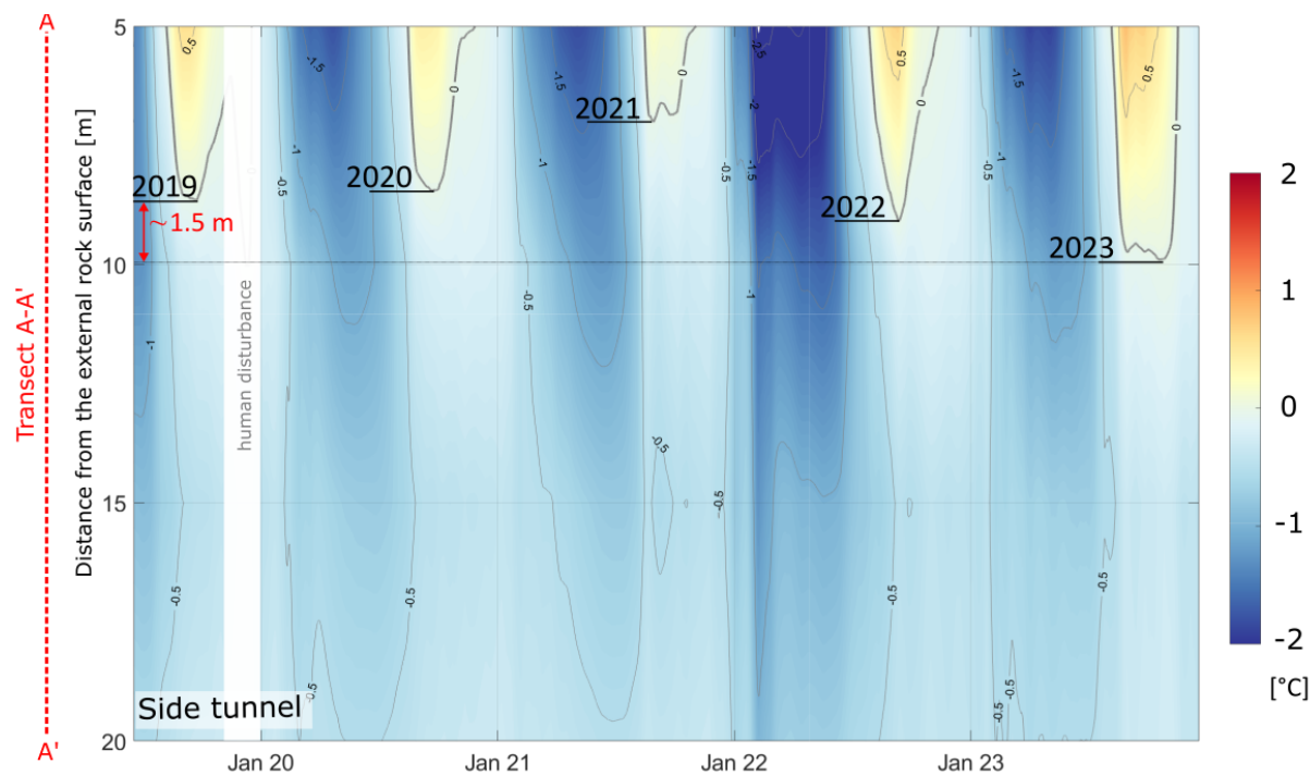
Figure 2. Temperature profile in the side tunnel. The location of the transect is visible in Fig. 1b (profile A-A').
