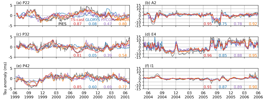
Figure 9. Time series of \tau anomaly at selected PIES sites. Comparison between PIES observation (black), TS-Cast (red), GLORYS (blue), HYCOM (purple), and ARMOR3D (orange). Correlation coefficients for each model are shown in the bottom right of each panel. The locations of these sites are shown in Figure 8.
