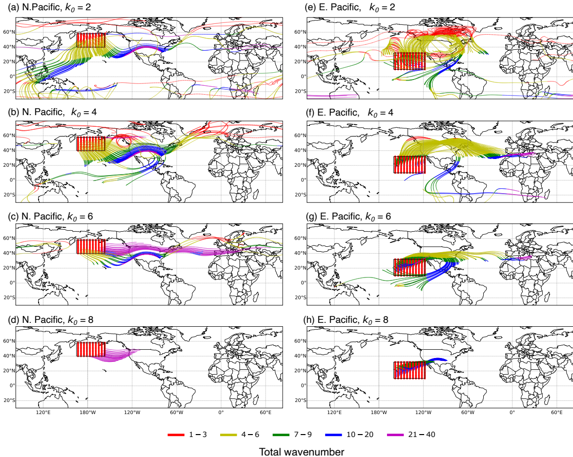
Figure 8. Samples of Rossby wave rays using the climatological July circulation from ERA-Interim as the base state. Each panel shows rays initiated from different the North Pacific source regions and region are shown on the left column, starting with a specific different initial zonal wavenumber ( k ) wavenumbers: (a) the North Pacific source region with initial k = 3k_0 = 2 , (b) also from the North Pacific source region but with initial k = 8k_0 = 4 , (c) the East Pacific source region with initial k = 2k_0 = 6 , and (d) also k_0 = 8 . The right column shows the rays from the tropical East Pacific source region but with initial k = 6 : (e) the Tibet source region with initial k = 1k_0 = 2 , (f) also from the Tibet source region but with initial k = 9k_0 = 4 , (g) k_0 = 6 , and (h) k_0 = 8 . Line colors represent time-dependent total wavenumber K (equation C10), and red dots show the source point location. Rays are terminated when the total wavenumber reaches 40 (wavelength of \approx 1,000 km), assuming that they are not small-amplitude perturbations at the geostrophic scale anymore (wave-breaking).
