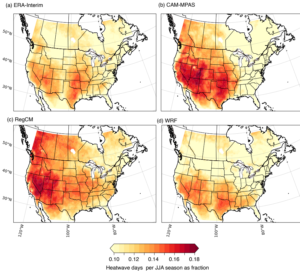
Figure 15. Fraction of the days identified as heatwaves (HWs) (or number of HW days per JJA (92) days) identified as HWs , in (a) ERA-Interim, (b) CAM-MPAS, (c) RegCM4, and (d) WRF.
