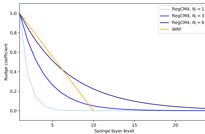
Figure B7. Illustration of the lateral boundary conditions in the RegCM4 and WRF configurations for NA-CORDEX: (a) an example configuration of specified and relaxation zones in the western boundary with n_{relax} = 10 , and (b) weighing coefficients ( F(n) ) in RegCM4 and WRF. Three curves are shown for RegCM4 corresponding to N_I = 1, 3, 6 .
