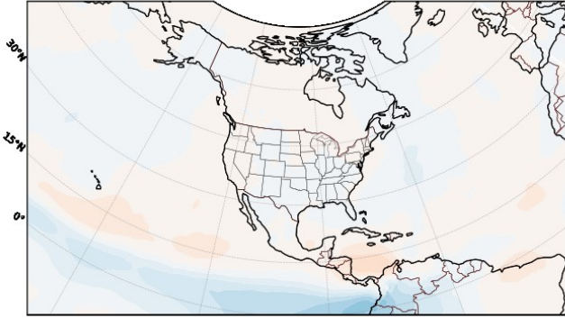
(c) WRF NoNudge - ERA-Interim, va_{200}
