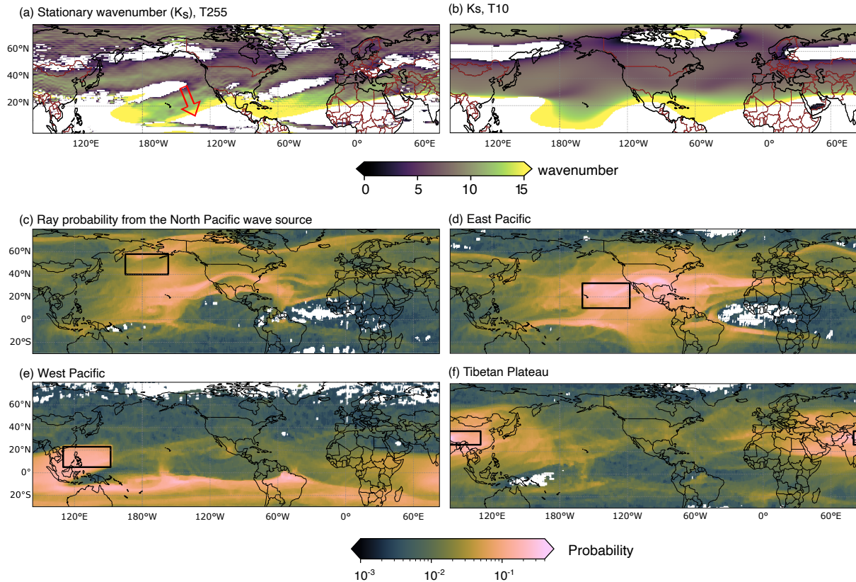
Figure 7. Probability-Waveguides for (quasi-)stationary Rossby waves, (a,b) diagnosed by stationary wavenumber, K_s , (eqn. 4) and (c-f) by the probability of Rossby wave propagation from obtained by the LZ15 ray tracing method. In (a selected), K_s is calculated from the JJA climatology from ERA-Interim on its native grid resolution (T255), while in (b) it is calculated from the smoothed climatology (T10), same as the background state for the ray tracing. The grid boxes with imaginary K_s are shown in white. The ray tracing results are presented separately for each source region: (ac) northern North Pacific, (bd) eastern subtropical Pacific, (ee) western tropical Pacific, (d) East-Asian Monsoon, (e) Indian Monsoon, and (f) Tibetan Plateau. Probability is calculated for each grid box as the fraction of rays reaching the grid box over the total number of rays traced from a source region. The base-state wind fields are the 1980-2010 monthly climatologies for June, July, and August from ERA-Interim.
