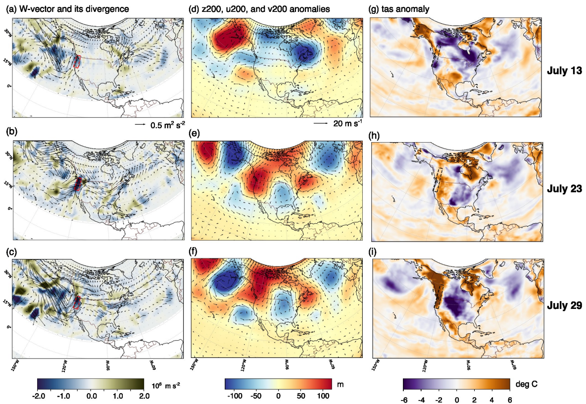
Figure 1. Evolution of stationary-quasi-stationary Rossby waves and surface air temperature ( tas ) during the 2009 heatwave event: (a-c) the flux (arrows) and divergence (color, blue = convergence, green = divergence) of daily-mean wave activity (WA) flux of derived from the 25-90 day band-passed geopotential height anomalies, (d-f) 200-hPa winds and geopotential height anomalies (25-90 day band-passed), and (g-i) daily tas anomaly, all variables from ERA-Interim.
