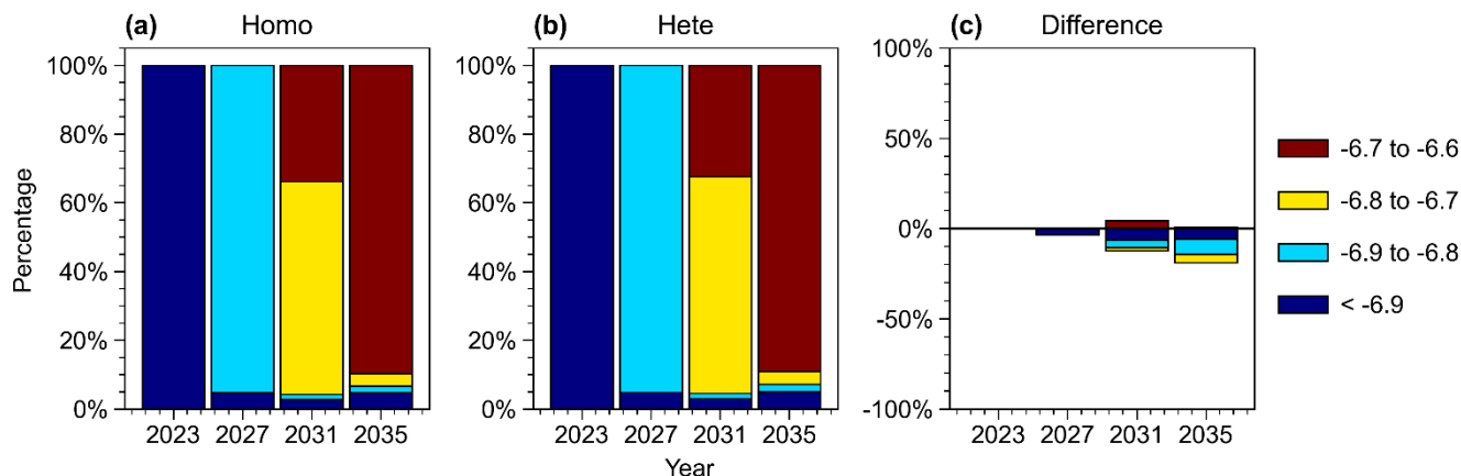
335 Figure 9. Area-contribution analysis of concentration log-difference response classes under denitrification. (a) Homogeneous; (b) Heterogeneous; (c) Relative difference.
