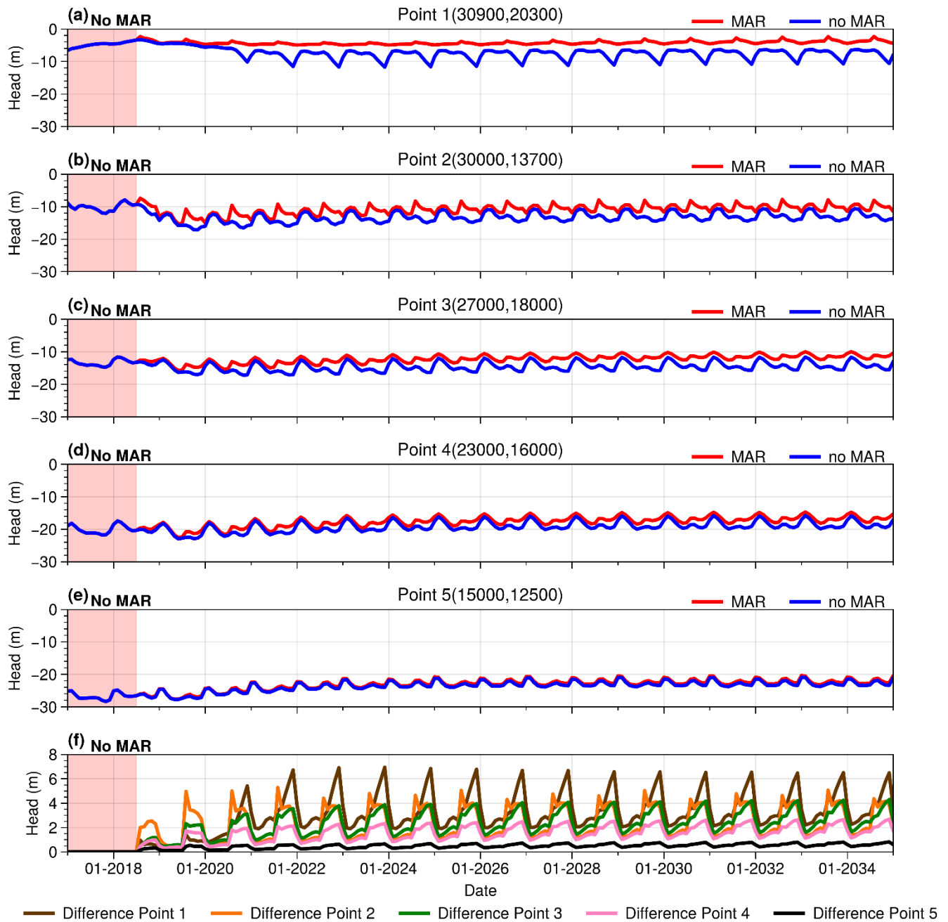
265 Figure 5. Groundwater level changes and differences at observation points; (a)–(e) Time series of water level changes at observation points (Point 1 to Point 5) with and without MAR; (f) Differences in water levels (MAR vs Without MAR) for all observation points
