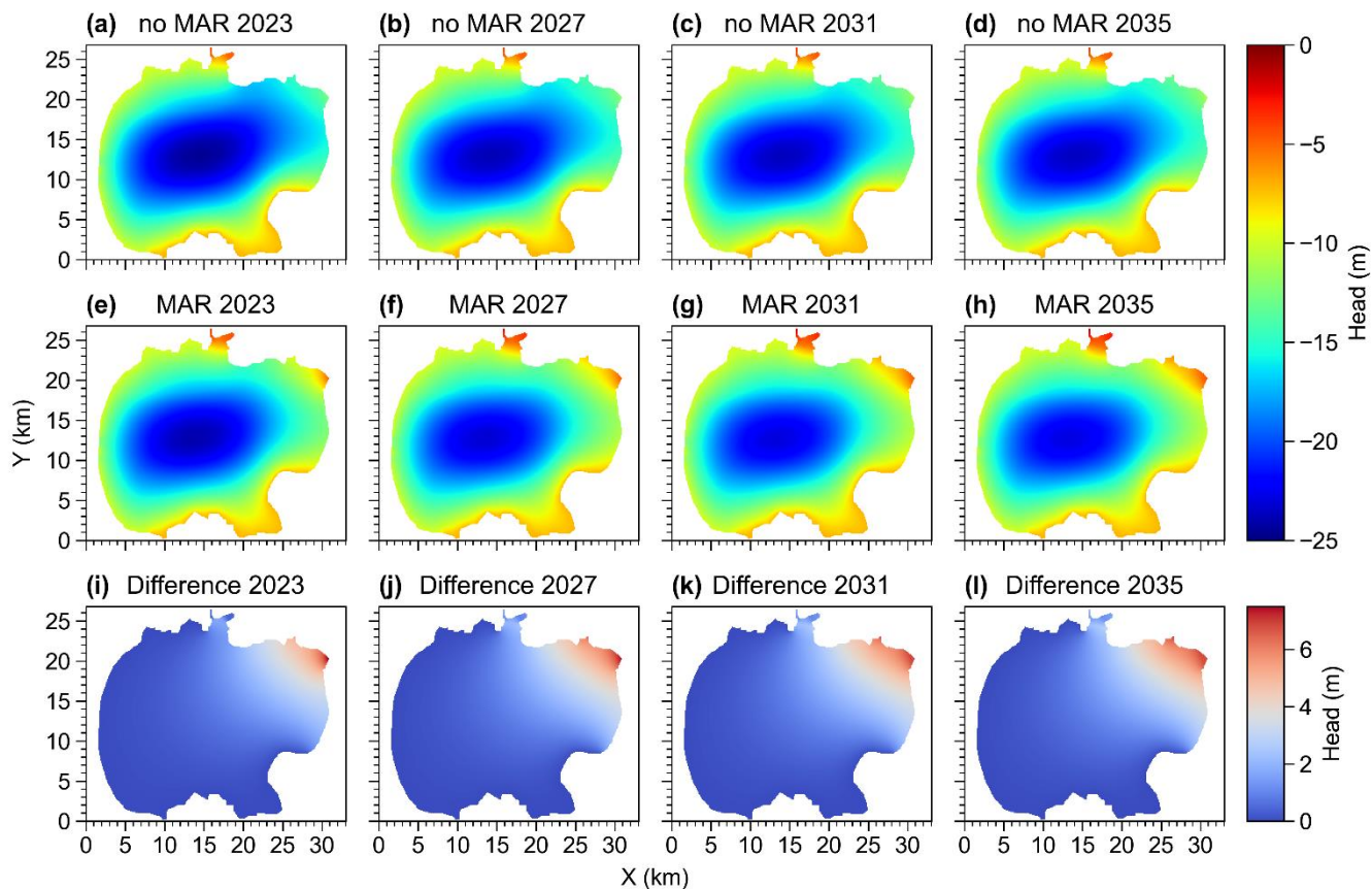
250 Figure 4. Spatial distribution of groundwater levels and changes with and without MAR (a)–(d) Spatial distribution of groundwater levels without MAR. (e)–(h) Spatial distribution of groundwater levels with MAR. (i)–(l) Spatial distribution of groundwater head differences.
