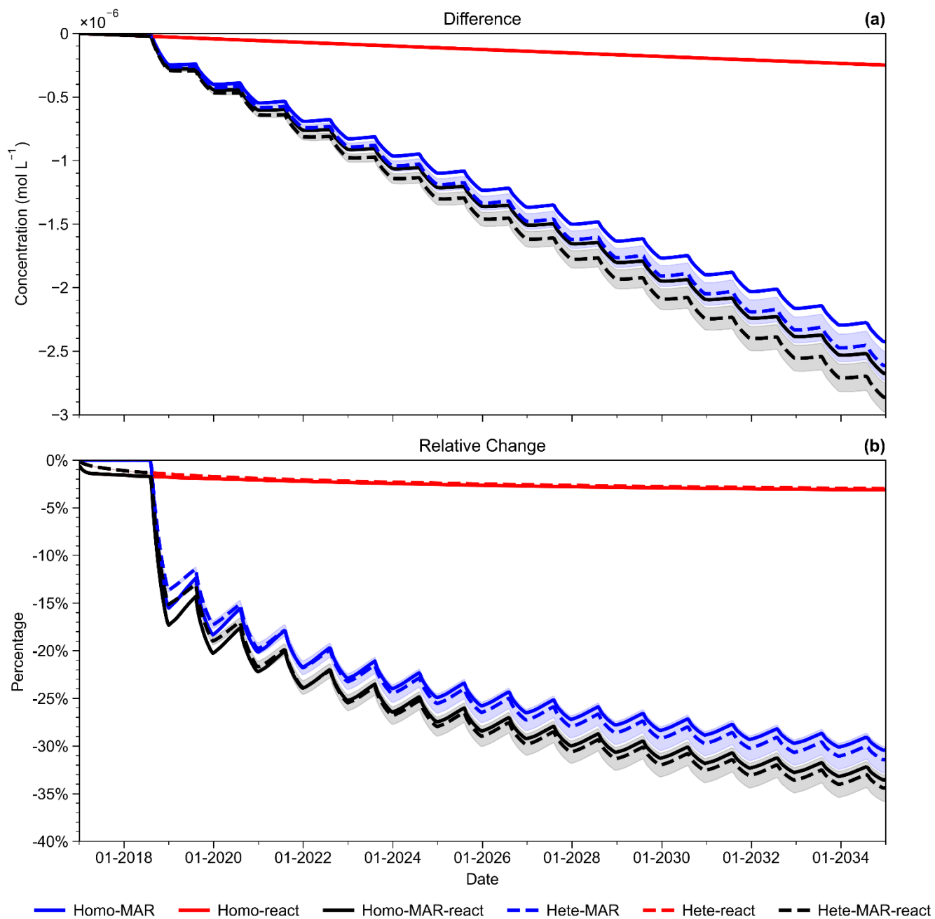
390 Figure 13. Domain-mean nitrate response over time. (a) Absolute difference in concentration relative to the baseline scenario (mol L -1 ). (b) Relative change (%).
