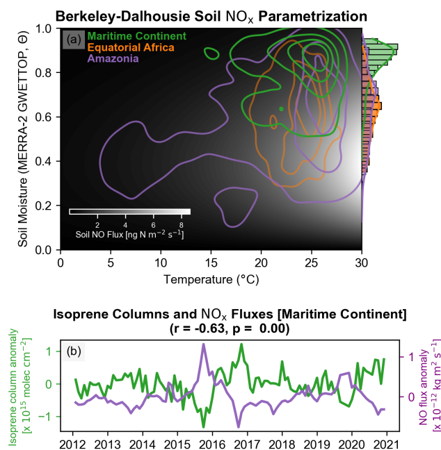
Figure 4. (a) Temperature and soil moisture dependence of the Berkeley-Dalhousie Soil NO x Parametrization, as described by Hudman et al. (2012). Soil NO x fluxes are displayed in grayscale, with white representing the highest soil NO x fluxes. Overlaid on the fluxes is temporally-averaged, land-masked soil moisture (GWETTOP) from the three tropical regions: Amazonia (purple), equatorial Africa (orange), and the Maritime Continent (green). As this data is temporally averaged, these contours represent the spatial distribution of soil moisture within these three regions. Of the three regions, the Maritime Continent has the least variance and the highest average soil moisture. (b) Time-series showing the isoprene column anomaly from CrIS over the Maritime Continent (green) alongside the soil NO x flux anomaly (purple) derived from offline BDSNP emissions forced by MERRA-2. The soil NO x is weighted by the gridpoint's average isoprene column over 2012–2020, which increases the impact of variations that occur in areas with high isoprene columns and thus potentially elevated isoprene emissions.
