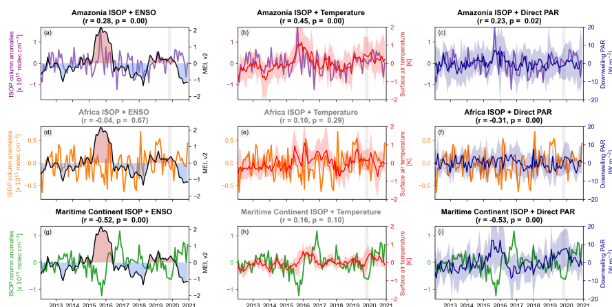
Figure 2. (a) Time-series of the multivariate ENSO Index, v2, against spatially-averaged isoprene column anomalies over Amazonia (in molecules \text{cm}^{-2} , purple). Isoprene columns over the Amazon positively correlate with ENSO. An analogous time-series for isoprene anomalies over equatorial Africa (orange) and the Maritime Continent (green) can be found in subplots (d) and (g). The Maritime Continent exhibits a strong negative correlation with the ENSO index. (b) Time-series of surface air temperatures (in K, red) from MERRA-2 reanalysis, and isoprene column anomalies (purple), showing a similar positive correlation over Amazonia. An analogous time-series for isoprene anomalies over equatorial Africa (orange) and the Maritime Continent (green) can be found in subplots (e) and (h). Shading represents the 10th to 90th percentile in temperature over each month. A gray title indicates a non-significant correlation ( p > 0.05 ). (c) Time-series of direct PAR (in \text{W m}^{-2} , blue) from MERRA-2 reanalysis, and isoprene column anomalies (purple) over Amazonia. Analogous time-series for equatorial Africa and the Maritime Continent can be found in subplots (f) and (i). Shading represents the 10th to 90th percentile in direct PAR over each month.
