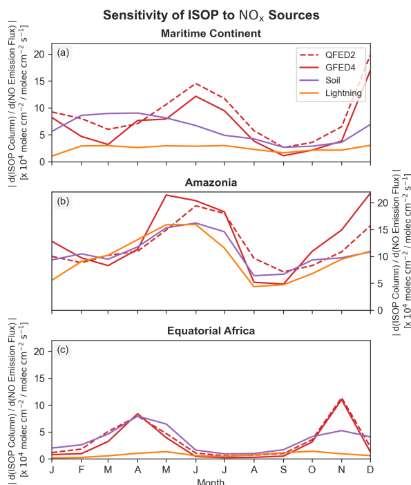
Figure 8. The absolute value of the change in isoprene columns for the four GEOS-Chem sensitivity studies, normalized by the change in column-integrated \text{NO}_x fluxes. All columns and fluxes were weighted by each box’s geographical area and summed over the entire bounding box for each region. These fluxes were calculated by decreasing each source’s inventory by 10%. The QFED2 perturbation changes were calculated relative to a control run with QFED2 biomass burning. Subplot (a) shows these values for the Maritime Continent, (b) for Amazonia, and (c) for equatorial Africa. Over equatorial Africa and the Maritime Continent, soil (purple) and biomass burning (red) \text{NO}_x have comparable sensitivities, while lightning \text{NO}_x (orange) has the lowest sensitivity of the three.
