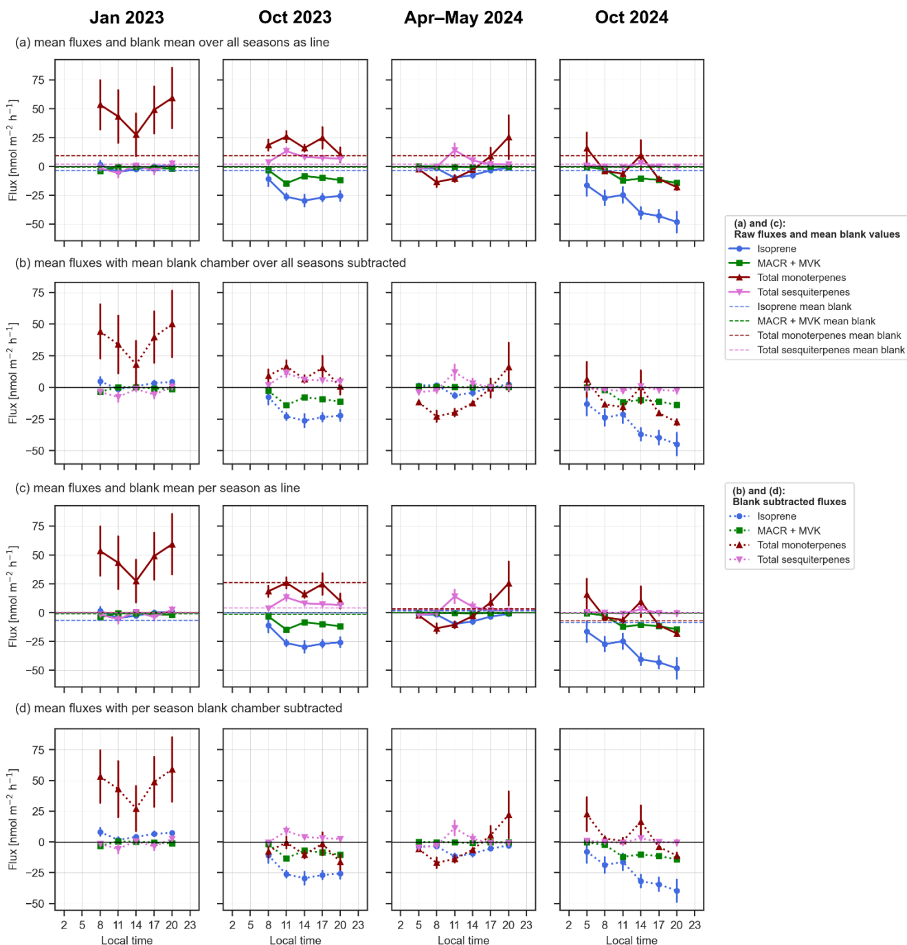
680 Figure A3 Diurnal curves of the mean calculated fluxes of isoprene (blue), isoprene oxidation products methacrolein (MACR) and methyl vinyl ketone (MVK), the total monoterpenes (red) and the total sesquiterpenes (pink) over the four measured seasons Jan 2023, Oct 2023, Apr-May 2024 and Oct 2024 in the course of a day from 5 am to 8 pm with blank values as dotted lines as mean (a) over all seasons (N=21) and (b) for each season (N=2 for Jan 2023, N=4 for Oct 2023, N=4 for Apr-May 2024, and N=11 for Oct 2025) and with subtracted blank values from the flux (b) over all seasons and (d) per season in \text{nmol m}^{-2} \text{h}^{-1} . Error bars indicate the standard error of the mean.
