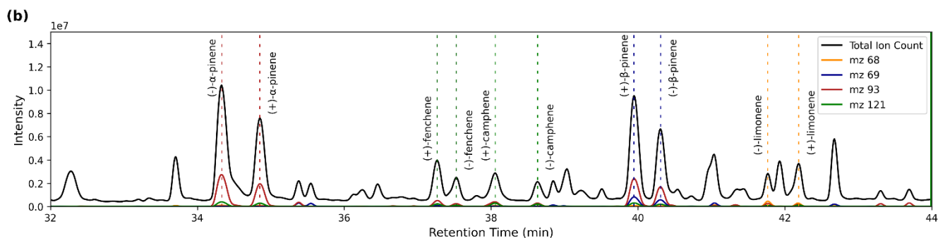
Figure A1 (a) Example Chromatogram of a soil chamber sample from October 2023 with annotation of isoprene, MACR, and MVK peaks, the chiral monoterpenes, and the two most prominent sesquiterpenes (b) Zoomed into the chiral monoterpene resolution.
