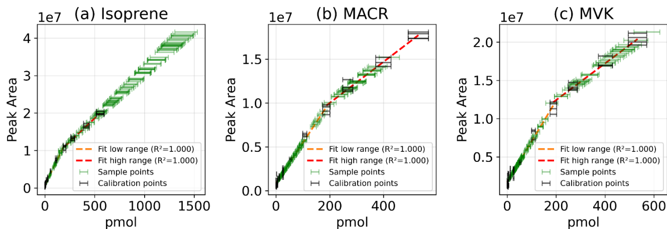
Figure A2 Calibration curve fit of integrated Peak Areas against substance on the cartridge in pmol for (a) isoprene, (b) MACR, and (c) MVK with calibration points with error bars plotted in black, linear fit in the lower range in orange and in the higher range in red, and sample points (from October 2024) in green with error bars.
