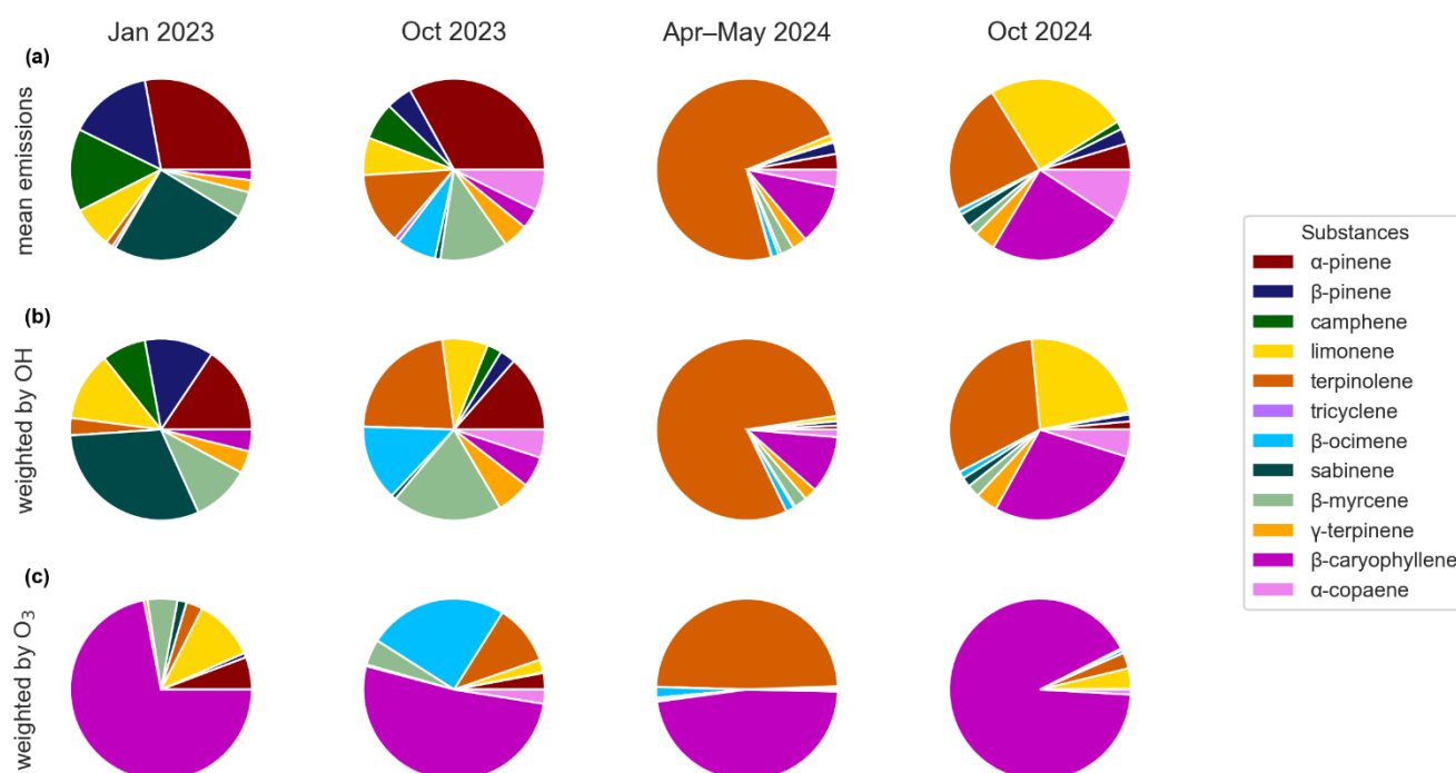
Figure 7 (a) Pie charts representing the mean emission fluxes composition. Reactivity impact on atmospheric chemistry towards (b) OH radicals and (c) Ozone ( \text{O}_3 ).
