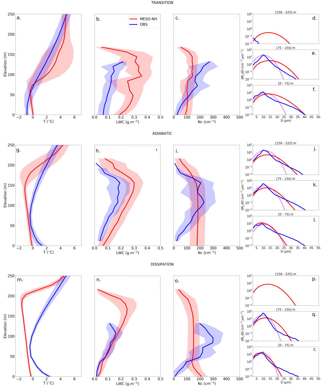
Figure 9. IOP 6: vertical profiles aggregated averaged by phases (23 for the thin-to-thick transition for the first line, 16 for the adiabatic for the second line, 3 for dissipation for the third line) of: Observed and simulated (a,g,m) absolute temperature, (b,h,n) LWC in g.m -3 , and (c,i,o) Nc in cm -3 . Panels on the right represent droplets distribution integrated over different layers. Model results are in continuous red and observation in dashed blue. For the DSDs, the pink line represents the distribution that the model would represent with the observed LWC and Nc. The envelopes for the vertical profiles represent \pm the standard deviation.
