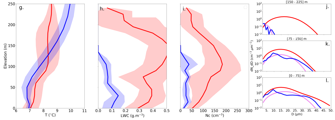
Figure 10. Same as Fig. 9 for IOP 11, but only for the 2 first periods, with 5 profiles aggregated averaged for the formation phase for the first line and 3 for the thin-to-thick transition for the second line.
