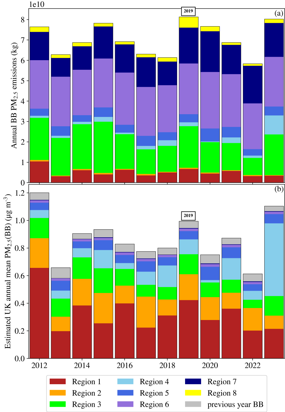
Figure 5. (a) The contributions from Regions 1-8 to annual global BB emissions of PM 2.5 from 2012 to 2023, using data from FINNv2.5 (Wiedinmyer et al., 2023). Regions are defined in Figure 2. (b) An estimate of the contributions of the source region emissions shown in panel (a) to UK annual mean PM 2.5 (BB) in 2012 to 2023, using 2019 as a reference year. The methodology and its assumptions are described in the main text. The bar for 2019 in plot (b) shows the absolute annual means corresponding to the relative contributions shown in Figure 4f.
