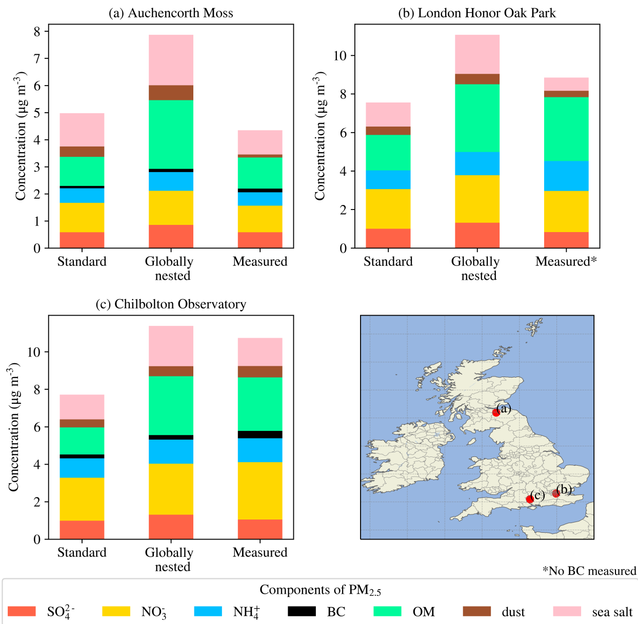
Figure B1. Comparison between modelled and measurement-derived SO 4 2- , NO 3 - , NH 4 + , BC, OM, dust and sea salt components of PM 2.5 at (a) Auchencorth Moss, (b) London Honor Oak Park and (c) Chilbolton Observatory measurement sites. Sites (a) and (c) are rural background sites, (b) is an urban background site. Site locations are shown in the bottom right panel. The left and middle bar of each panel show the 2019 annual modelled mean concentrations calculated using the standard and globally nested configurations of EMEP4UK, respectively, for the model grid containing the measurement site. The concentrations for each component in the right bar are the averages calculated using all available measurements in 2019 for that component at that site. Measurements were taken from the UK Air data archive (DEFRA, 2025). There were no measurements of BC at site (b) in 2019, so BC has also been omitted from the modelled data at this site.
