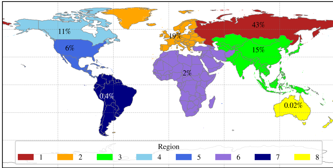
Figure 2. The eight source regions used for source-receptor experiments with the UK as the receptor region. The legend shows the assigned numbers. The percentage value superimposed on each source region is the relative contribution made by that region's BB emissions to the 2019 UK annual mean PM_{2.5} conditional on biomass burning. The percentages do not sum to 100% because of contributions from BB emissions in 2018 and non-linear interactions not captured by these 'brute force' model experiments.
