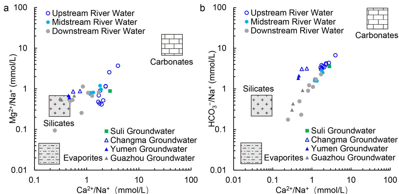
260 Figure 7: Mixing diagram of the Na-normalized molar ratios of (a) \text{Ca}^{2+} versus \text{Mg}^{2+} and (b) \text{Ca}^{2+} versus \text{HCO}_3^- in the Shule river. The data for the three endmembers, i.e., carbonates, silicates and evaporites, are obtained from Gaillardet et al. (1999).
