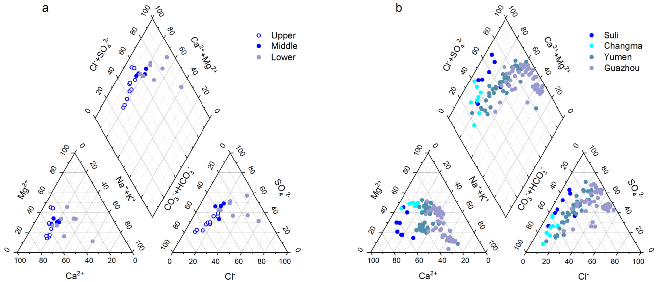
235 Figure 5: Piper trilinear plots for the chemical compositions of the river water and groundwater in the study area. In order to more clearly understand the changes in the hydrochemical characteristics of groundwater, groundwater samples were classified according to the sampling locations. The upper reaches include Suli and Changma, the middle reaches include Yumen, and the lower reaches include Guazhou.
