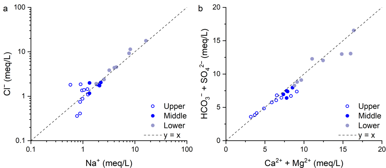
410 Figure 9: Bivariate ionic correlations in Shule River water: (a) \text{Na}^+ versus \text{Cl}^- concentrations, (b) (\text{Ca}^{2+} + \text{Mg}^{2+}) versus (\text{HCO}_3^- + \text{SO}_4^{2-}) concentrations.
